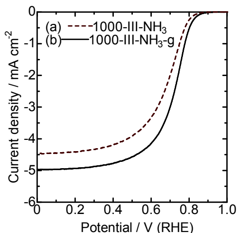
Figure 8. ORR voltammograms with the 1000-III-NH 3 and 1000-III-NH 3 -g catalysts. Temperature: RT, catalyst loading: 0.2 mg cm -2 , electrolyte: 0.5 M H 2 SO 4 , rotation: 1500 rpm.
