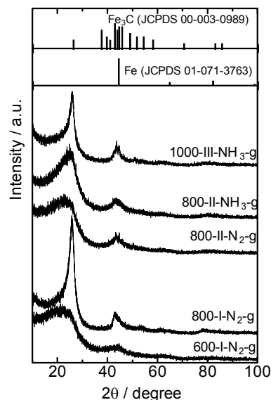
Figure 2. XRD patterns of the catalysts prepared by different pyrolysis protocols.
