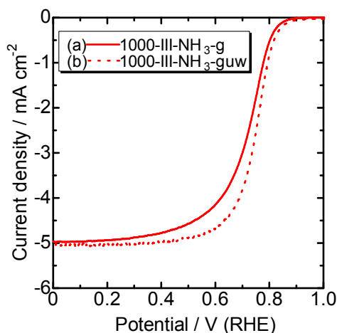
Figure 6. ORR voltammograms with the 1000-III-NH 3 -g and 1000-III-NH 3 -guw catalysts. Temperature: RT, catalyst loading: 0.2 mg cm -2 , electrolyte: 0.5 M H 2 SO 4 , rotation: 1500 rpm.
