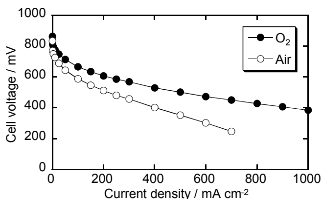
Figure 9. I-V polarization curve of the MEA with the 1000-III-NH 3 -g catalyst. Cathode: 1000-III-NH 3 -g 4 mg cm -2 , O 2 0.2 MPa. Anode: PtRu/C catalyst 0.4 mg-Pt cm -2 , H 2 0.2 MPa. Electrolyte: Nafion NR211. T: 80°C.
