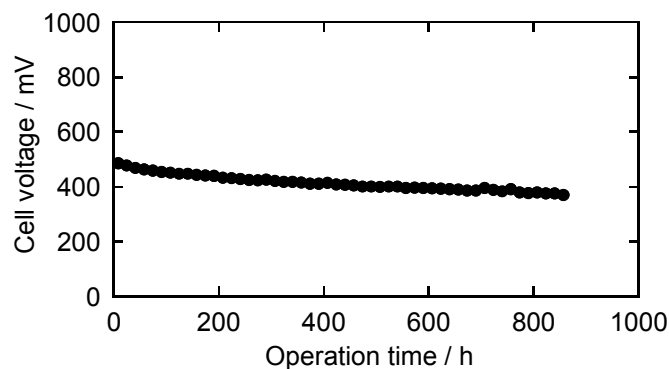
Figure 10. Durability test of the MEA with the 1000-III-NH 3 -g catalyst. Cathode: Air 0.2 MPa. Anode: H 2 0.2 MPa. Current density: 200 mA cm -2 .
