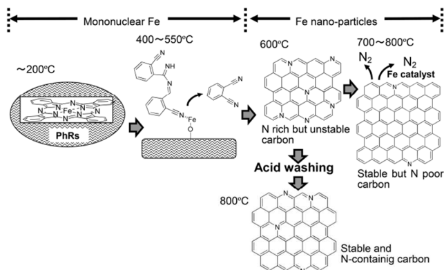
Figure 1. The concept of multi-step pyrolysis.
