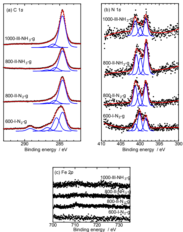
Figure 3. (a) C 1s, (b) N 1s and (c) Fe 2p XPS spectra of the prepared carbon materials, dots: measured data; lines: fitted curves.
