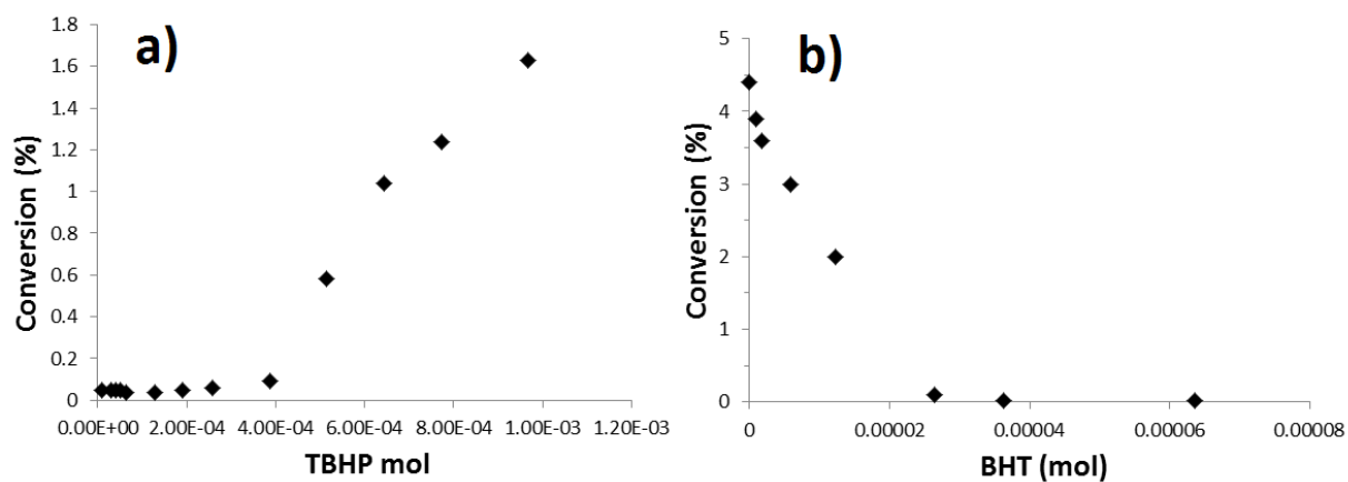
Figure 2: a) The addition of radical initiator to cyclopentene containing BHT ( 3 \times 10^{-5} M) and b) the addition of BHT to stabiliser free cyclopentene. Reaction conditions: substrate (10 ml), catalyst (0.12g), glass reactor, atmospheric pressure.
