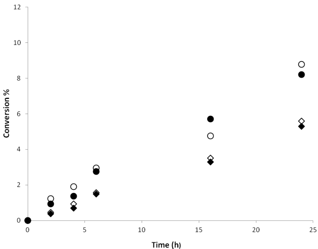
Figure 1: Effect of reaction time for the conversion of cis-cyclooctene at 80 °C and cyclohexene at 50 °C. Reaction conditions: 5 ml of alkene, 0.06g Au/G, glass reactor, TBHP ( 0.032 \times 10^{-3} mol) and atmospheric pressure. Cyclohexene containing stabiliser with TBHP (●), stabiliser-free cyclohexene without TBHP (○), cis-cyclooctene containing stabiliser with TBHP (◆) and cis-cyclooctene after the removal of stabiliser without TBHP (◇).
