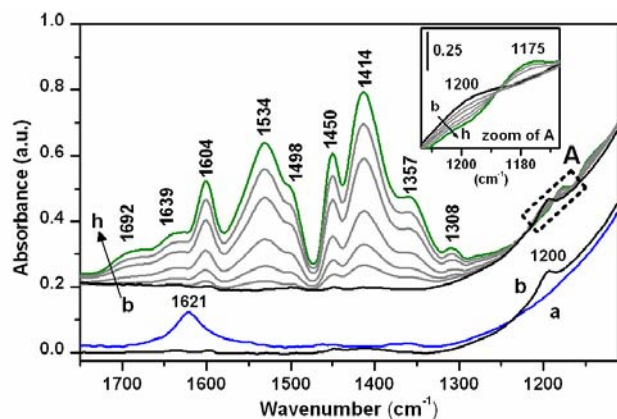
Figure 2. IR spectra of: (curve a) TiO 2 activated at 450 °C, then contacted with water vapor pressure and subsequently outgassed at b.t. for 30 min; (curve b) after D 2 O adsorption/desorption cycles (until attainment of spectra invariance) and subsequent outgassing at b.t. for 30 min; (curves c-h) increasing amounts of BA-d adsorbed from the vapor phase. Inset: zoomed view of the 1215–1165 cm -1 range of the spectra from D 2 O irreversibly adsorbed at b.t. (curve b) to its complete displacement by BA-d (curve h). The full range spectra are reported in Figure S1 in the Supporting Information.
