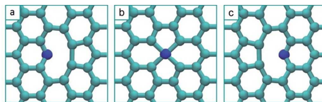
Figure 2. Initial ground state (a), transition state (b), and final ground state (c) for one migration step of the reconstructed 5/9 monovacancy in graphene. Reprinted (adapted) from ref. 161.
