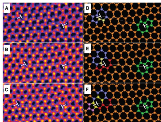
Figure 10. Real-time dislocation dynamics. HRTEM images showing changes in the position of an edge glide dislocation with time under continuous electron beam irradiation. Time (A) 0 s. (B) 141 s. (C) 321 s. (D to F) Atomic models illustrating the structures inferred from (A) to (C), respectively. The white T indicates the position of the dislocation. The transition from structures (A,D) to (B,E) corresponds to a glide of the dislocation core, while the transition from (B,E) to (C,F) corresponds to a climb step, associated with the emission of a pair of atoms. Reprinted (adapted) from ref. 218 with permission from AAAS.
