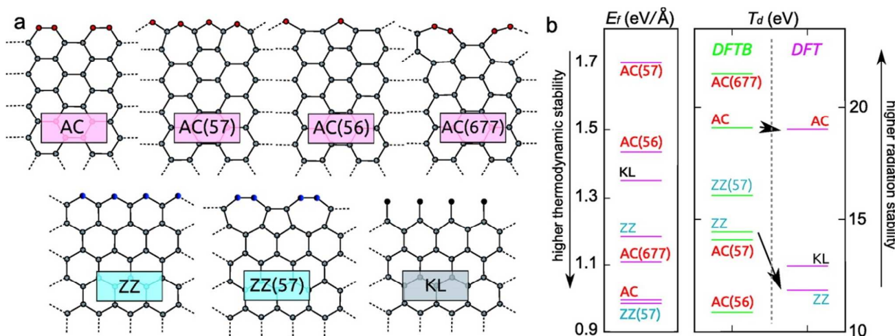
Figure 13. (a) Different edge reconstructions as optimised by DFT and (b) their formation energies E_f and displacement thresholds T_d . Displacement thresholds as calculated with both DFT and DFTB are presented, showing the disagreement between DFT and DFTB for ZZ edges. Uncertainties in the T_d are of the order of 0.1 eV. Reprinted (adapted) with permission from ref. 148. Copyright (2014) American Chemical Society.
