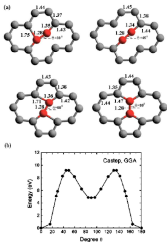
Figure 8. The Stone-Wales transformation: (a) Intermediate structures corresponding to different angles of bond rotation \vartheta (in degrees) as indicated in the panels. The atoms at the defect core are shown in red. All the bond lengths are in Å. (b) The corresponding formation energy as a function of the rotation angle \vartheta . Reprinted (adapted) from ref. 166. Copyright (2005) by the American Physical Society.
