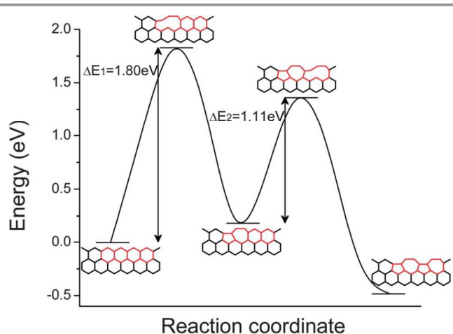
Figure 14. The minimum energy path of the first and second step transitions from a hexagon-hexagon pair to a pentagon-heptagon pair. Reprinted (adapted) from ref. 77.
