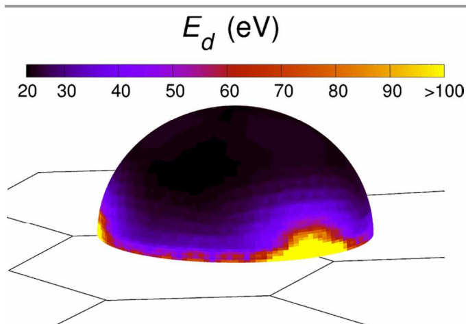
Figure 15. Mapping of the threshold energy for emission of an atom from pristine graphene as a function of the angle of transferred momentum from the e-beam. The threshold energy of 23 eV rises very rapidly to large energies at angles parallel to the graphene sheet. Reprinted figure with permission from ref. 265. Copyright (2007) by the American Physical Society.
