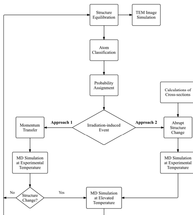
Figure 1. CompuTEM algorithm for including irradiation-induced structure changes in TEM image simulations. Reprinted (adapted) from ref. 15.
