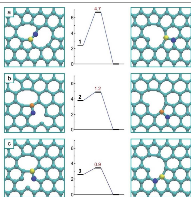
Figure 6. The final steps of the merging of a 5/9 monovacancy with a V_2(5-8-5) divacancy, from the three non-equivalent 3rd nearest neighbour positions (a), (b), and (c), where the two atoms involved in each transition have been coloured to track their movement. The energies of initial and transition states relative to the final state are indicated. Reprinted (adapted) from ref. 161.
