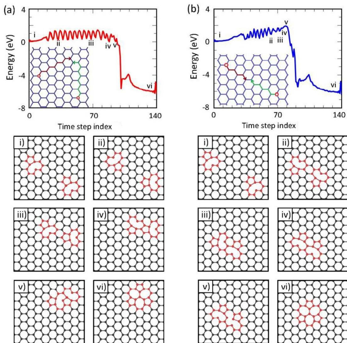
Figure 5. The process of merging monovacancies into a V_2(555-777) divacancy for different pathways for the approaching migration of vacancies. The potential energy of system relative to the initial state along migration pathways is shown as function of time step index in action-derived molecular dynamics simulation. Reprinted (adapted) from ref.142. Reproduced by permission of IOP Publishing. All rights reserved.
