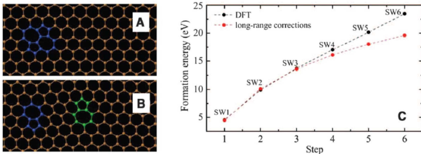
Figure 11. (A and B) Atomistic models obtained within DFT for one and four Stone-Wales bond rotations (steps 1 and 4). (C) Formation energy at each step (one dislocation is stationary and the other one is moving along the glide direction). The black dots represent the DFT data. The red dots represent the DFT data corrected for long-range strain-field interactions. Reprinted (adapted) from ref. 218 with permission from AAAS.
