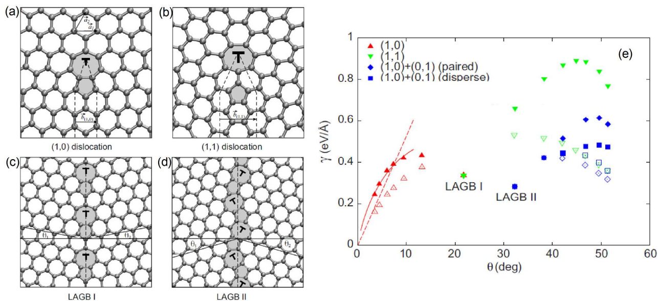
Figure 12. (a,b) Atomic structures of (1,0) and (1,1) dislocations. The dashed lines delimit the semi-infinite strips of graphene introduced at the dislocation core. Non-hexagonal rings are shaded. (c,d) Atomic structures of the \theta=21.8^\circ (LAGB I) and the \theta=32.2^\circ (LAGB II) symmetric large-angle grain boundaries, respectively. The dashed lines show the boundary lines and the solid lines define angles \theta_1 and \theta_2 ( \theta=\theta_1+\theta_2 ) defining orientations of the graphene grains. (e) Grain-boundary energy per unit length \gamma as a function of misorientation angle \theta for various flat (filled symbols) and buckled (open symbols) grain-boundary structures. The two energetically favorable large-angle grain boundaries, LAGB I and LAGB II, are labeled. The dashed curve shows the asymptotic linear dependence of \gamma for the buckled small-angle armchair grain boundaries ( E_f = 7.5 eV). Reprinted figures with permission from ref. 221. Copyright (2010) by the American Physical Society.
