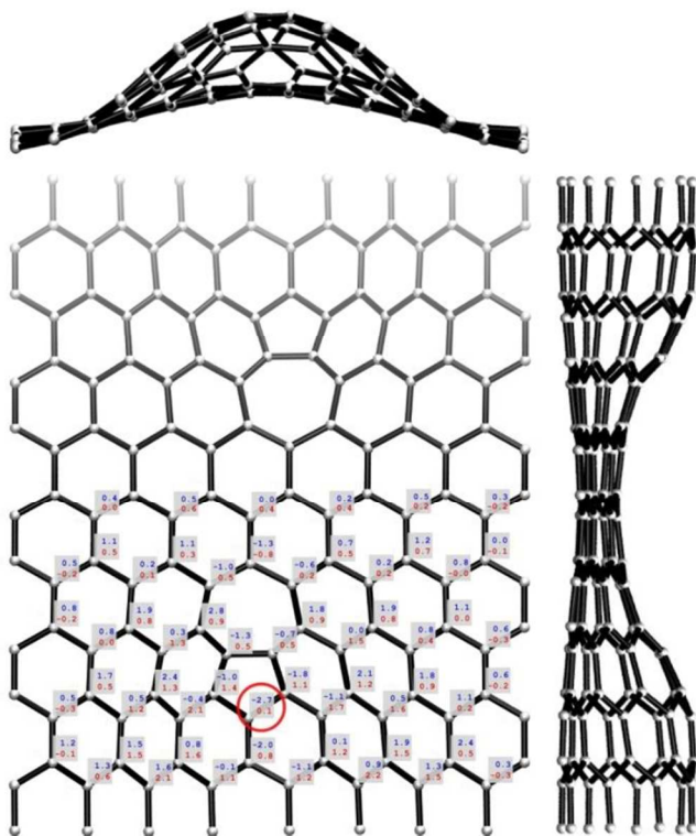
Figure 16. Emission threshold energies calculated for atoms surrounding a dislocation core. Values are given as deviations from the pristine value calculated using the same method (21.34 eV). As the structure is buckled out-of-plane (side views), it is not symmetrical, resulting in different threshold energies when the momentum is transferred upwards (blue numbers) and downwards (red numbers). Reprinted (adapted) from ref.225 (Supplementary Information).
