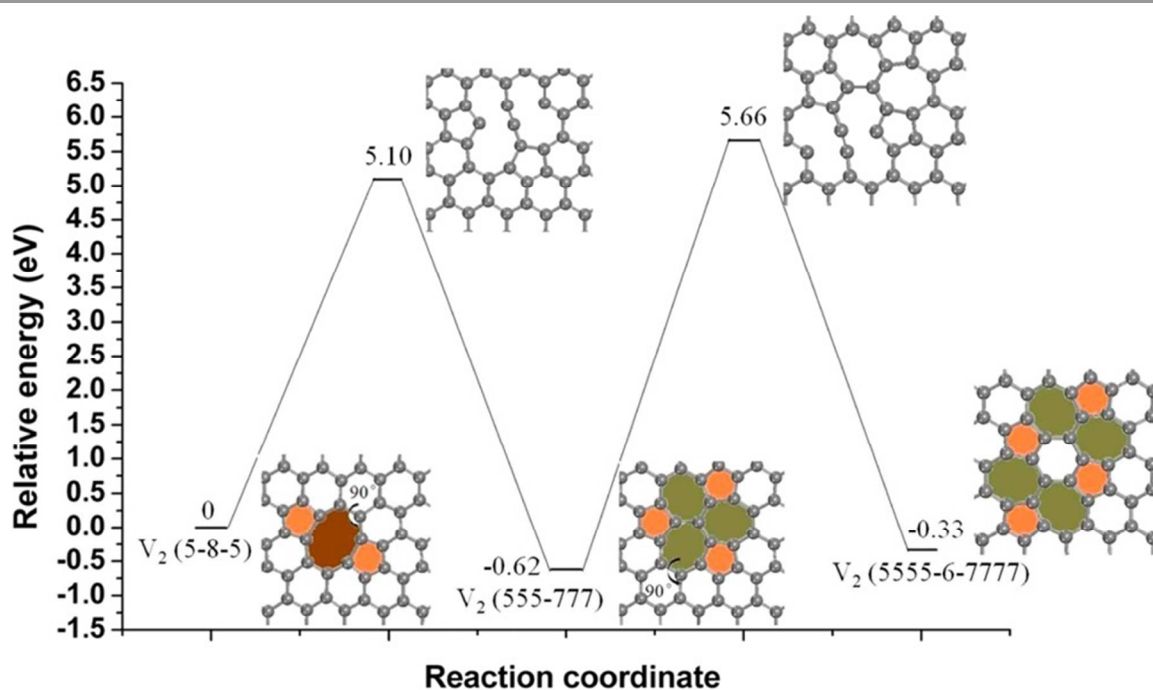
Figure 3. Schematic representation of the structure and energetics for three states of a divacancy in graphene: V_2(5-8-5) state, V_2(555-777) state and V_2(5555-6-7777) state, and transition states for transition between V_2(5-8-5) and V_2(555-777) states and between V_2(555-777) and V_2(5555-6-7777) states. Reprinted (adapted) with permission from ref. 162. Copyright (2013) American Chemical Society.
