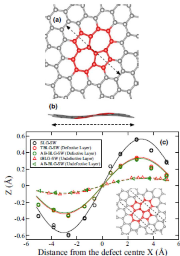
Figure 7. Structure of the SW defect in single-layer graphene (SLG): (a) top view and (b) side view showing the distortion of the defective graphene sheet. The side view in (b) is taken by viewing perpendicular to the dashed line in (a). (c) The distortion pattern for the SW defects in SLG, twisted bilayer graphene (TBLG) and bilayer with the AB stacking (AB-BLG). A distortion amplitude of zero corresponds to the centre of the SW defect. The dashed line in the inset encloses the atoms over which the deviations from zero are measured. Reprinted (adapted) from ref. 35. Copyright (2014) by the American Physical Society.
