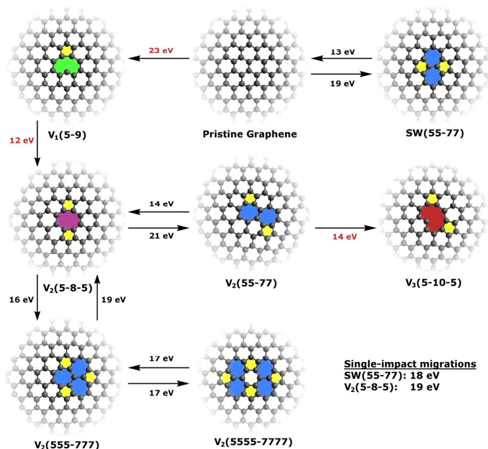
Figure 17. A summary of the threshold energies calculated for irradiation-induced processes in ref 266. Emission processes are labelled in red and bond rotations (SW rearrangements) in black. Rings are coloured according to their size: 5, yellow; 6, white; 7, blue; 8, purple; 9, green; 10, red. Threshold energies are also given for the direct migration of structures across the graphene lattice due to a single impact from the e-beam, only witnessed for a small number of combinations of angle space and transferred energy.
