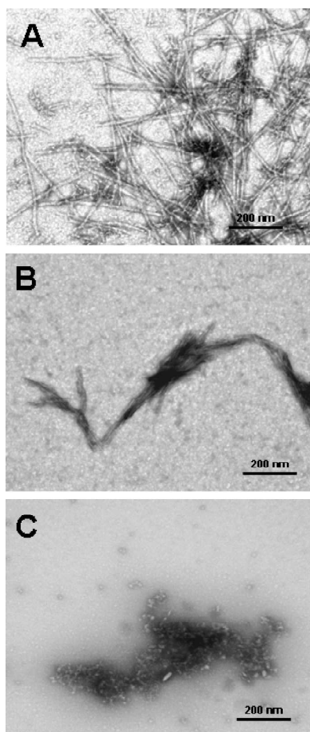
Fig. 15 Transmission electron micrographs of: A \beta (1-40) incubated at pH 7.4 (coexistence of fibrils and globular oligomers) ( A ); A \beta (1-40) incubated at pH 7.4 in the presence of minor PPI-DS-Mal G3 (detection of clumped fibrils) ( B ); A \beta (1-40) incubated at pH 7.4 in the presence of PPI-DS-Mal G4 (dendrimer-peptide ratio 1, detection of granular non-fibrillar, amorphous aggregates) ( C ). A \beta (1-40) and A \beta (1-40)-dendrimer complexes were incubated for 12 hours at pH 7.4 and 37°C before the preparation of the microscopy grids. Reproduced with permission from “O. Klementieva, N. Benseny-Cases, A. Gella, D. Appelhans, B. Voit, J. Cladera, Biomacromolecules 2011 , 12 , 3903–3909“. Copyright 2011 American Chemical Society.
