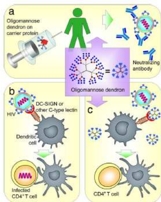
Fig. 2 Possible biologically molecular interactions of oligomannose dendrons as (anti-adhesive) dendritic glycoconjugate to suppress HIV-1 infection. (a) Possible conjugation to proteins and use as vaccines. (b) HIV-1 infection by HIV-1 binding to dendritic cell-surface DC-SIGN or other mannose-binding proteins to enhance CD4 + T cell infection. (c) Possible inhibition of the binding of HIV-1 to dendritic cell-surface DC-SIGN or other mannose-binding proteins to prevent dendritic cell-enhanced CD4 + T cell infection. Reproduced with permission from “S.-K. Wang, P.-H. Liang, R. D. Astronomo, T.-L. Hsu, S.-L. Hsieh, D. R. Burton, C.-H. Wong, Targeting the carbohydrates on HIV-1: Interaction of oligomannose dendrons with human monoclonal antibody 2G12 and DC-SIGN Proc. Natl. Acad. Sci. USA , 2008, 105 , 3690-3695“. Copyright 2008 National Academy of Sciences. U.S.A.
