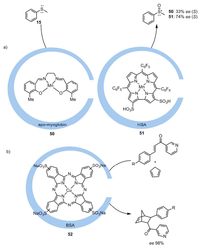
Fig. 27 Encapsulation of different metal complexes in protein environment and their use in catalysis (BSA = bovine serum albumin, HSA = human serum albumin).
