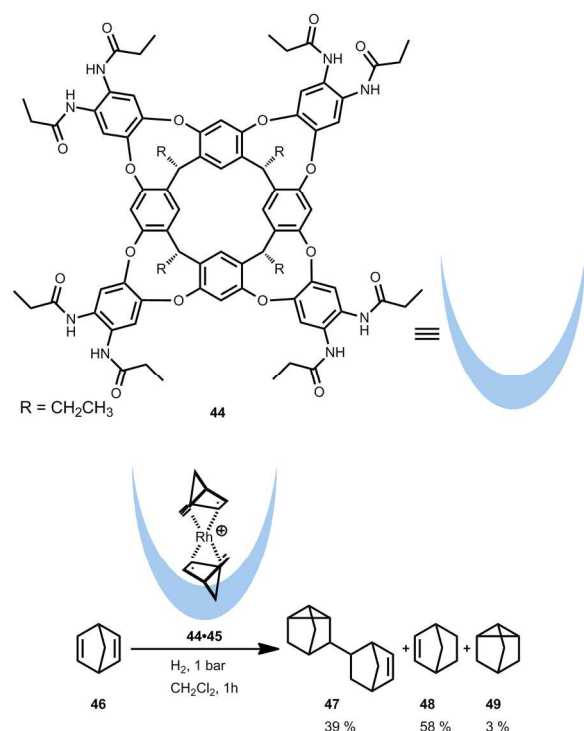
Fig. 25 Encapsulated 44 • 45 catalyst and its performance in hydrogenation of norbornadiene.
