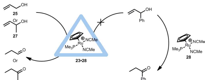
Fig. 19 Allylic isomerization within 23•28 compared to non-encapsulated ruthenium catalyst showing substrate selectivity.
