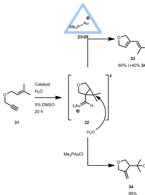
Fig. 21 Catalytic behavior of encapsulated 23•29 in the intramolecular cyclo-isomerization reaction of 31 compared to non-encapsulated gold catalysts.
