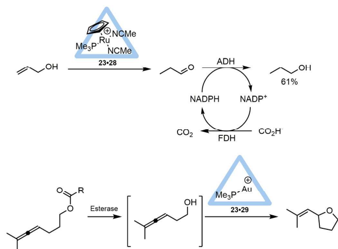
Fig. 22 Tandem reactions using combination of metal encapsulated and enzyme catalysts in water.
