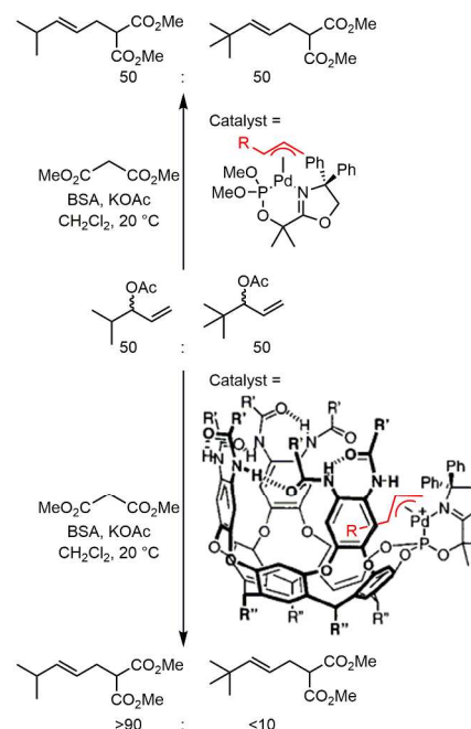
Fig. 1 Nucleophilic attack on the Pd-allylic species yielded new substrate selectivity when a cavitand was used to create a second coordination sphere around the catalyst. (BSA: N,O -bis(trimethylsilyl)acetamide)
