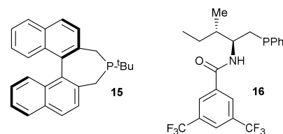
Figure 3. Chiral catalysts for enantioselective [4 + 2] cycloadditions between allenoates and imines.
