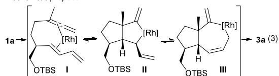
Scheme 1. Pioneering [4 + 2] cycloadditions by Wender. 9
