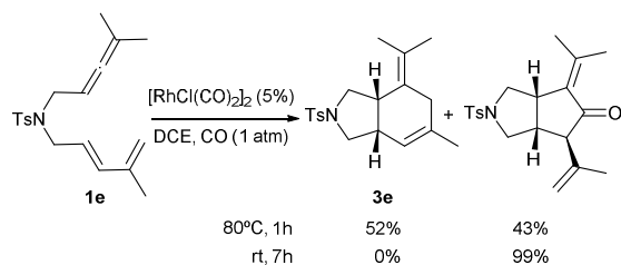
Scheme 3. [4 + 2] vs [2 + 2 + 1] allene-diene cycloadditions.
