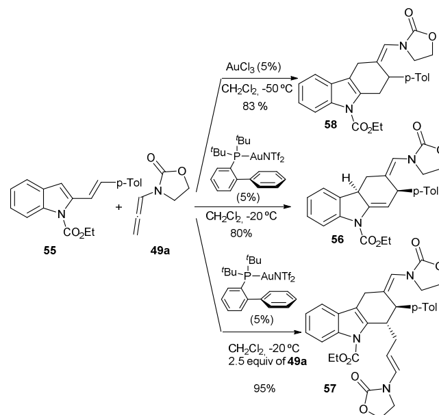
Scheme 30. Au-catalyzed [4 + 2] cycloaddition of allenamides and vinyl indoles.
