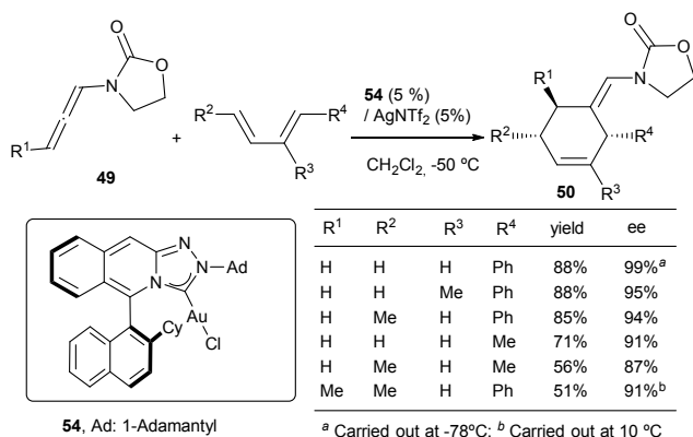
Scheme 29. Enantioselective Au-catalyzed [4 + 2] cycloaddition of allenamides and dienes.
