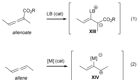
Figure 2. Types of zwitterionic intermediates proposed in catalytic [4 + 2] and [4 + 3] cycloadditions of allenes.
