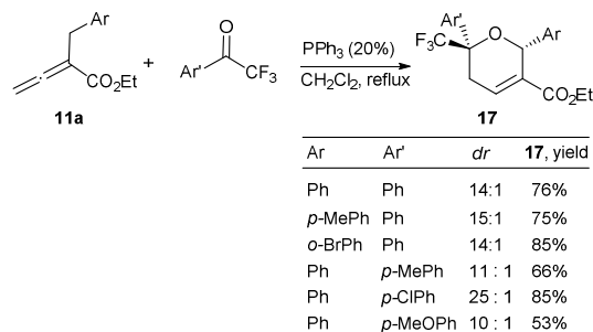
Scheme 10. [4 + 2] Cycloadditions of allenates and ketones.
