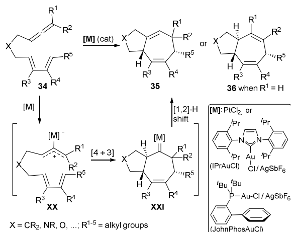
Scheme 19. Au and Pt-catalyzed [4 + 3] cycloadditions of allene-dienes 34 .
