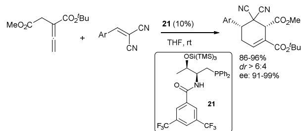
Scheme 13. Enantioselective [4 + 2] cycloadditions of allenates.
