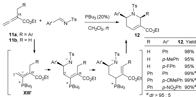
Scheme 8 [4 + 2] Cycloadditions between \alpha -substituted allenoates and imines.
