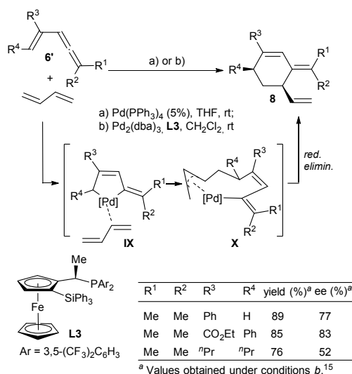
Scheme 6. Pd-catalyzed [4 + 2] cycloadditions of vinylallenes.
