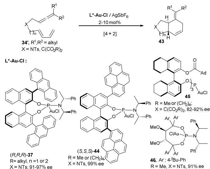
Scheme 24. Chiral gold catalysts for allene-diene enantioselective [4 + 2] cycloadditions.
