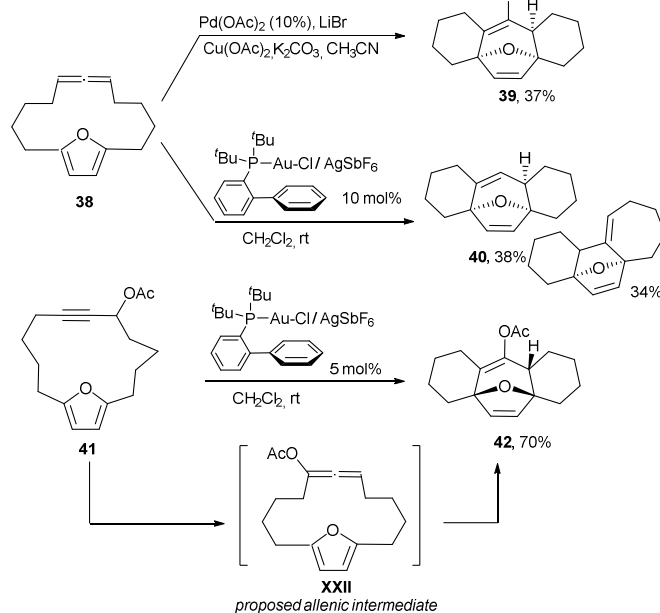
Scheme 21. Allene-diene transannular [4 + 3] cycloadditions.
