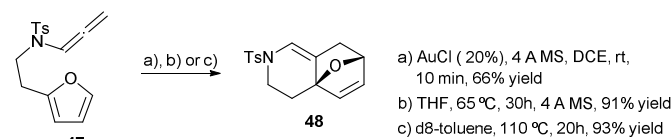
Scheme 25. Furan-allenamide intramolecular [4 + 2] cycloadditions.
