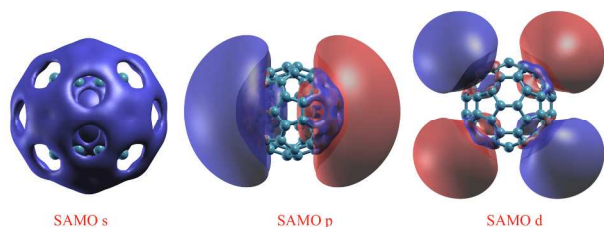
Figure 2. DFT-LDA calculated SAMOs, illustrating the typical Hydrogen-like s, p, and d symmetric shapes in C_{60} .
