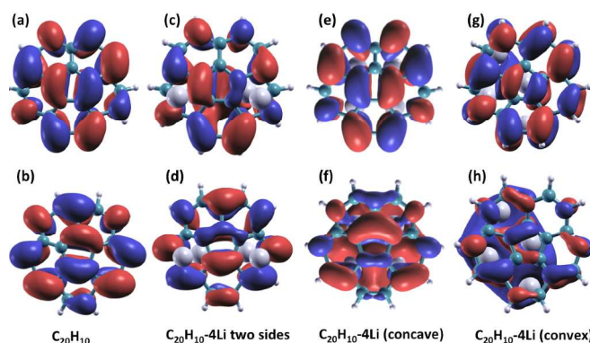
Figure 5. (a),(b) degenerate LUMOs in C_{20}H_{10} , (c),(d) HOMO and HOMO-1 in Li-doped C_{20}H_{10} , 2 Li convex side and 2 Li on concave side, (e),(f) HOMO and HOMO-1 in Li-doped C_{20}H_{10} 4 Li on concave side, (g),(h) HOMO and HOMO-1 in Li-doped C_{20}H_{10} 4 Li on convex side.
