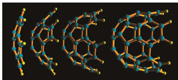
Figure 6. Curved aromatic bowl constructs of increasing size and depth, based on the smallest corannulene unit (left most).
