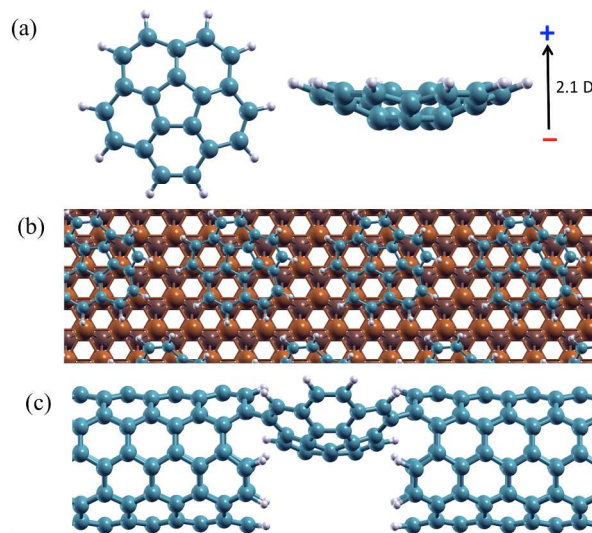
Figure 1. (a) C_{20}H_{10} molecular structure showing the shallow bowl and intrinsic dipole; (b) C_{20}H_{10} molecules arranged on a Cu(111) surface; (c) C_{20}H_{10} molecule assembled into a molecular junction.
