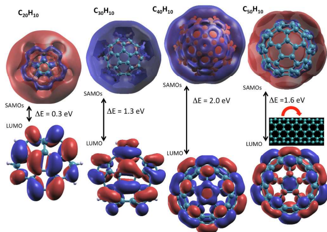
Figure 9. G_0W_0@LDA predicted trends across the series of bucky bowls, C_{20}H_{10} , C_{30}H_{10} , C_{40}H_{10} , C_{50}H_{10} .
