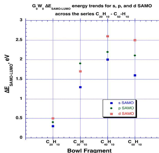
Figure 7. Trends in G_0W_0@LDA predicted \Delta E_{\text{SAMO-LUMO}} across the series of
