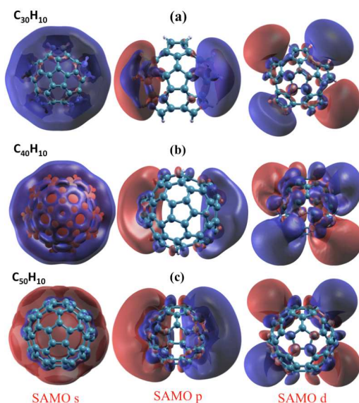
Figure 8. DFT-LDA representation of SAMOs illustrating the typical s, p, d-like symmetric shapes in (a) C_{30}H_{10} , (b) C_{40}H_{10} , (c) C_{50}H_{10} .
