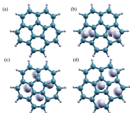
Figure 4. (a) Un-doped C_{20}H_{10} , (b) Li-doped C_{20}H_{10} , 2 Li convex side, 2 Li concave side, (c) Li-doped C_{20}H_{10} 4 Li concave side, (d) Li-doped C_{20}H_{10} 4 Li convex side.
