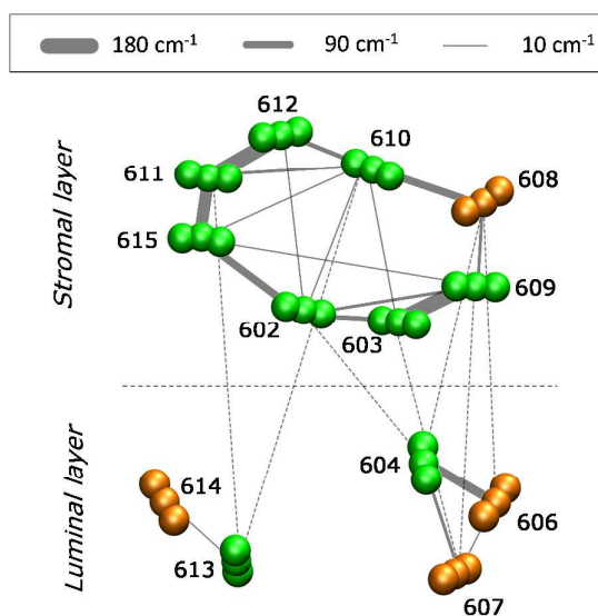
Figure 5. Schematic representation of the average MMPol@MD couplings. The thickness of the lines connecting the pigments are proportional to the coupling values. Dotted lines are referred to couplings between pigments facing on different side of the thylakoid membrane. Couplings < 10 \text{ cm}^{-1} are not reported.
