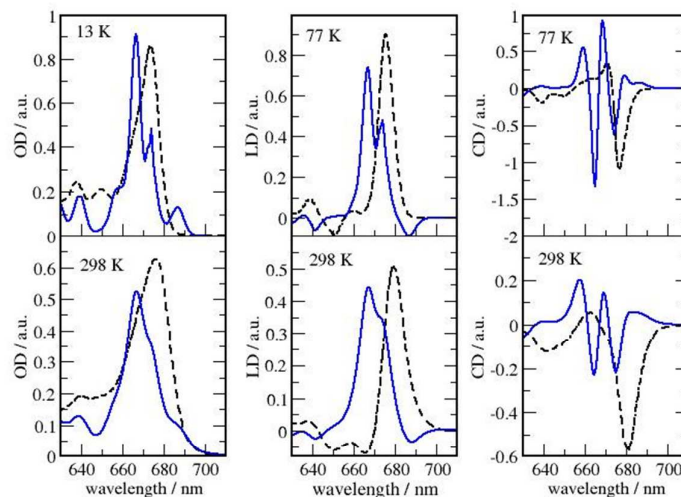
Figure 7. Comparison of optical spectra calculated with the MMPol@CRY exciton Hamiltonian (Table S4) (blue solid lines) with experimental data (Ref. 32, dashed lines). In the left panel the linear absorbance spectra at 13 K (upper part) and at 298 K (lower part) are shown. The middle panel contains the linear dichroism spectra at 77 K (upper part) and 298 K (lower part) and the right panel the circular dichroism spectra at 77 K (upper part) and 298 K (lower part).
