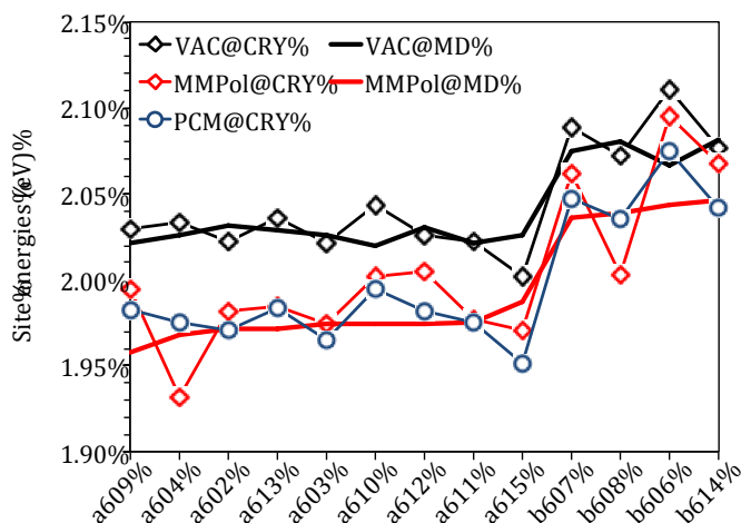
Figure 3. Site energies of Chls computed at cam-B3LYP/6-31G(d) level of theory. Data are referred to calculations on the crystalline structure (@CRY, lines with symbols) and averaged on MD configurations (@MD, lines without symbols), and with different environment descriptions.
