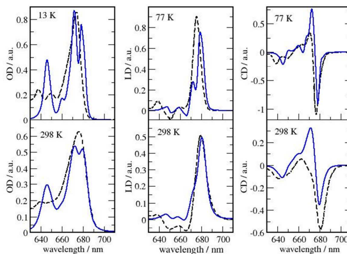
Figure 8. Comparison of optical spectra calculated with the MMPol@MD exciton Hamiltonian (Table S5) (blue solid lines) with experimental data (Ref. 32, dashed lines). In the left panel the linear absorbance spectra at 13 K (upper part) and at 298 K (lower part) are shown. The middle panel contains the linear dichroism spectra at 77 K (upper part) and 298 K (lower part) and the right panel the circular dichroism spectra at 77 K (upper part) and 298 K (lower part).
