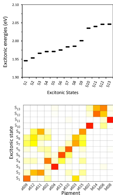
Figure 7. Upper Panel: energy progression of the excitonic states obtained from MMPol@MD data. Lower panel: excitonic state composition in terms of individual pigments (obtained through the probability coefficient |c_i^{(k)}|^2 ). Red squares mean high contribution, white negligible contribution.
