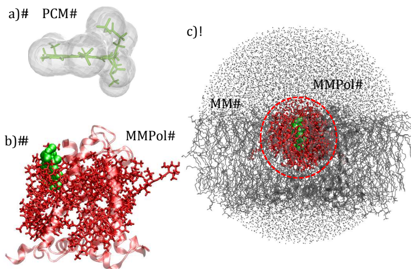
Figure 2. Schematic representation of the different environmental models used: a) QM/PCM; b) QM/MMPol in the case of crystal structure, all non-QM atoms are considered as polarizable sites; c) QM/MMPol in the case of a MD snapshot, a cut-off of 12 Å around QM atoms is applied for MM polarizability and a larger cut-off of 45 Å is set for MM charges.
