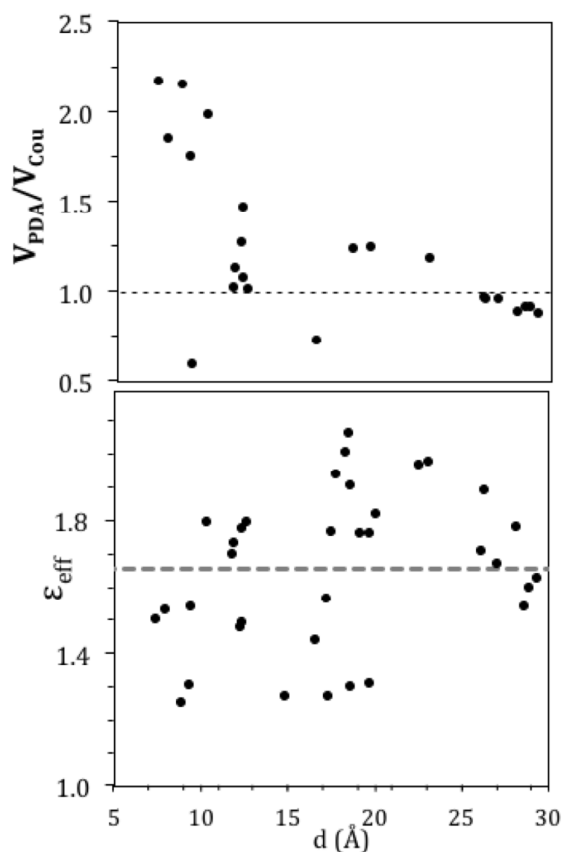
Figure 6. Upper panel: ratio between MMPol@MD couplings computed with point-dipole approximation and coulomb coupling computed with QM method. Lower panel: effective dielectric constant computed for MMPol@MD (filled black circle); the dotted grey line represents the average \epsilon_{\text{eff}} .
