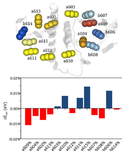
Figure 4: Upper panel: representation of the cluster of chlorophylls colored according to their site energies (from lowest, red, to highest, blue). Lower panel: Relative energy differences (in eV) between MMPol@MD and VAC@MD site energies (see eq.(13)).
