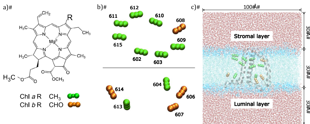
Figure 1. a) Molecular structure of Chl a and b . b) Simplified model of the crystal structure of CP29 with only the Chl molecules observed perpendicularly to the thylakoid membrane plane. Chl structures are represented by the central Mg atom and the two nitrogen atoms along the direction of Q_y transition dipole. c) Side view parallel to the membrane plane of the computational system; the dimensions of the lipid membrane and solvation water layers are also reported.
