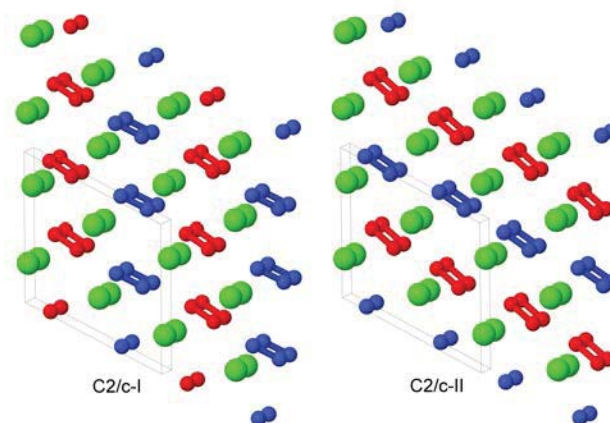
Fig. 2 2x2x2 slabs of the C2/c-I (left) and C2/c-II (right) structures, viewed almost down the b -axis. Both structures are very similar, with Ca atoms forming an almost-hexagonal motif when viewed from this angle. Green atoms correspond to Ca atoms, while red and blue correspond to O atoms. All O atoms in peroxide ions with parallel O-O axes are given the same colour.
