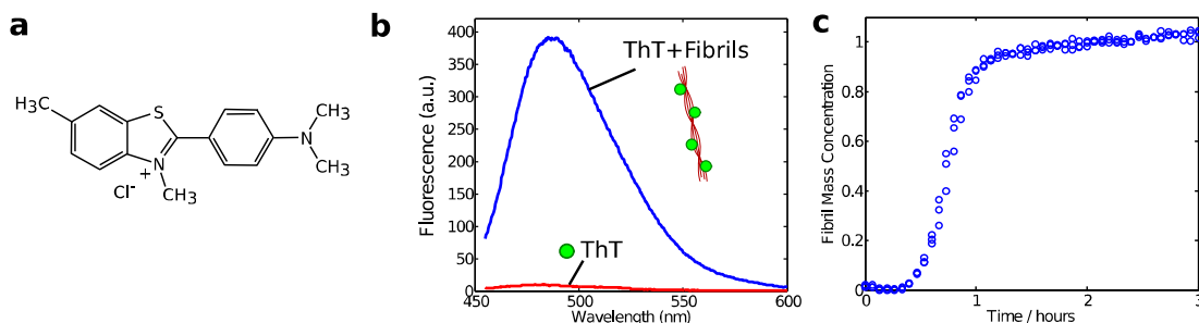
Figure 6. a) Structure of the ThT dye and b) change in the emission fluorescence spectrum upon binding to amyloid fibrils. Typical excitation wavelength is 440 nm; c) The fibril formation process is monitored by recording the relative changes in the fluorescence intensity during time with respect to the situation at time zero.
