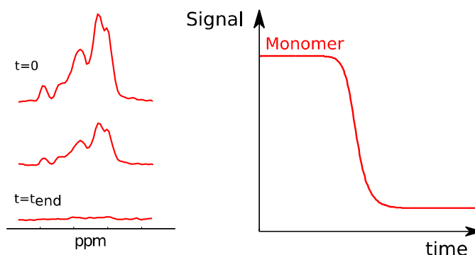
Figure 5. NMR spectra acquired during an ongoing reaction (left). The monomer concentration as a function of time (right) is extracted from the peak intensities.
