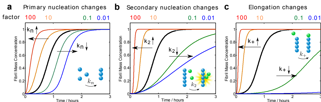
Figure 12. Effect of individual rate constants on macroscopic aggregation growth curves. In each panel the black curve represents the simulated time evolution of the fibril mass versus time for a 4 \mu\text{M} solution of A \beta 42 in 20 mM phosphate buffer, 0.2 mM EDTA, 0.02% NaN 3 at pH 8.0 under quiescent conditions according to the following rate constants: k_n k_+ = 900 \text{ M}^{-2} \text{ s}^{-2} ; k_2 k_+ = 4 \cdot 10^{10} \text{ M}^{-3} \text{ s}^{-2} , and nucleus size n_c = n_2 = 2 . a) The original calculated curve (black) and curves generated by increasing ( k_n k_+ = 9 \cdot 10^3 \text{ M}^{-2} \text{ s}^{-2} ; orange and k_n k_+ = 9 \cdot 10^4 \text{ M}^{-2} \text{ s}^{-2} ; red) or decreasing ( k_n k_+ = 90 \text{ M}^{-2} \text{ s}^{-2} , green; k_n k_+ = 9 \text{ M}^{-2} \text{ s}^{-2} , blue) the rate constant for primary nucleation by a factor of 10 or 100. b) The original curve (black) and curves generated by increasing ( k_2 k_+ = 4 \cdot 10^{11} \text{ M}^{-3} \text{ s}^{-2} orange; k_2 k_+ = 4 \cdot 10^{12} \text{ M}^{-3} \text{ s}^{-2} red) or decreasing ( k_2 k_+ = 4 \cdot 10^9 \text{ M}^{-3} \text{ s}^{-2} green; k_2 k_+ = 4 \cdot 10^8 \text{ M}^{-3} \text{ s}^{-2} blue) the rate constant for secondary nucleation by a factor of 10 or 100. c) The original curve (black) and curves generated by increasing ( k_n k_+ = 9 \cdot 10^3 \text{ M}^{-2} \text{ s}^{-2} and k_2 k_+ = 4 \cdot 10^{11} \text{ M}^{-3} \text{ s}^{-2} orange; k_n k_+ = 9 \cdot 10^4 \text{ M}^{-2} \text{ s}^{-2} and k_2 k_+ = 4 \cdot 10^{12} \text{ M}^{-3} \text{ s}^{-2} red) or decreasing ( k_n k_+ = 90 \text{ M}^{-2} \text{ s}^{-2} , k_2 k_+ = 4 \cdot 10^9 \text{ M}^{-3} \text{ s}^{-2} , green; k_n k_+ = 9 \text{ M}^{-2} \text{ s}^{-2} , k_2 k_+ = 4 \cdot 10^8 \text{ M}^{-3} \text{ s}^{-2} , blue) the rate constant for elongation by a factor of 10 or 100.
