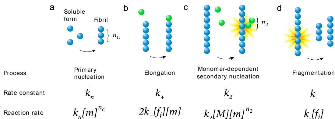
Figure 9. Microscopic processes underlying amyloid formation and associated rate constants and reaction rates: primary nucleation from monomers in solution (a), elongation (growth) by monomers addition to existing aggregates (b), surface catalyzed secondary nucleation from monomers on fibril surface (c) and fragmentation (d). In the expressions of the reaction rates in the last row, [m] refers to the free monomer concentration, [M] to the total fibril mass concentration and [f_i] to the fibril number concentration, while the rate constants are defined in the middle row.
