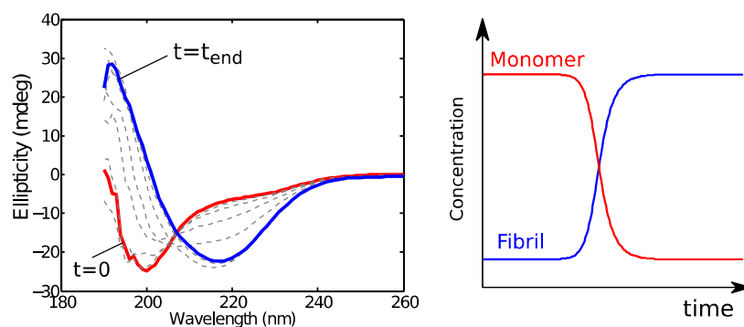
Figure 4. CD spectra acquired during an ongoing reaction (left). The first spectrum (red) shows the unfolded monomer and the last spectrum (blue) the \beta -sheet fibril. The monomer
