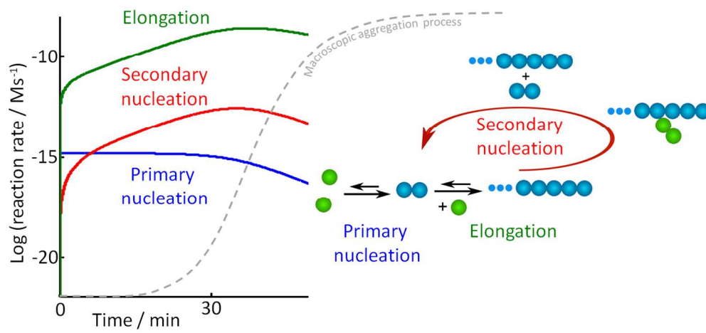
Rates of microscopic processes taking place during the lag phase of amyloid fibril formation for a reaction starting from an initially monomeric 4 \mu\text{M} solution of A \beta 42 400x200mm (96 x 96 DPI)
