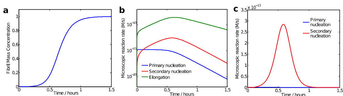
Figure 11. Model predictions of the aggregation reaction of a 4 \mu\text{M} solution of A \beta 42 using the rate constants as determined from kinetic analysis of a large body of data 17, 53 ; a) Macroscopic aggregation curve; b-c) Microscopic reaction rates: the maximum elongation (green line) and secondary nucleation rate (red line) occurs close to the half-time, while primary nucleation rate (blue line) is constant during the lag phase and decreases as monomers concentration is reduced. The reaction rates are shown with logarithmic y-axis in b and with linear y-axis in c.
