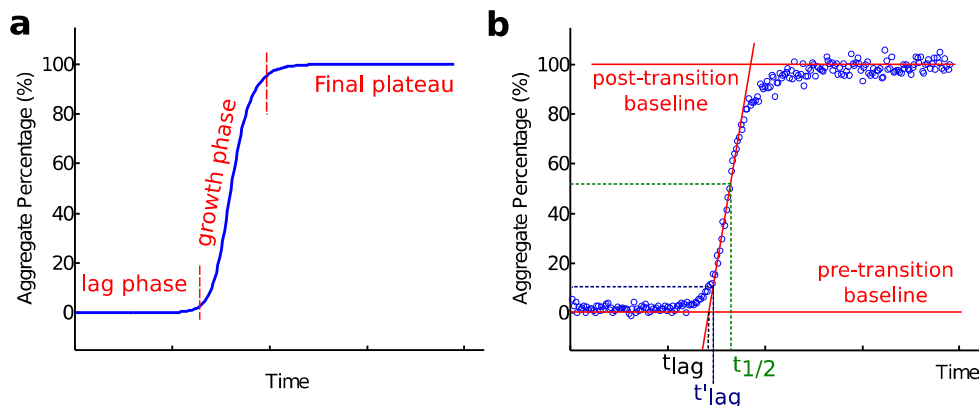
Figure 3. a) A characteristic macroscopic aggregation curve for amyloid fibril formation is displayed in terms of aggregate concentration (in monomer equivalents, % of total monomer) versus time. The curve is typically divided into a lag phase, a growth phase and a final plateau; b) Definition of t_{1/2} , and two alternative definitions of the lag time. Here t_{lag} is obtained by extrapolating the maximum derivative down to the intercept with the pre-transition base-line; while t'_{lag} and t_{1/2} are defined as the point in time where the signal relative to the pre-transition base line has reached 10% and 50% of the amplitude of the transition, respectively.
