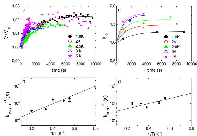
Fig. 6 Annealing of OX63 samples in the presence of TMA. a) Magnetic relaxation curves recorded, at \mu_0H = 3.5 T, after rapidly quenching to different temperatures. b) Temperature dependency of the electron magnetization relaxation rates. c) Annealing time dependency of the DNP enhanced steady-state polarization of 1M ^{13}\text{C} -TMA measured at 1.4K after annealing at the indicated temperatures. d) Temperature dependency of the rate constant for the increase of steady-state polarization with the annealing time. OX63 concentration was 30 mM in glycerol-water (1:1) with 1 M TMA (natural abundance or isotopically enriched). In a) and c) curves have been normalized by the initial magnetization M_0 or NMR intensity I_0 , respectively. Solid lines are least-squares exponential fits. The various time points in c) and d) were measured in independent samples over several months, confirming the robustness of the results.
