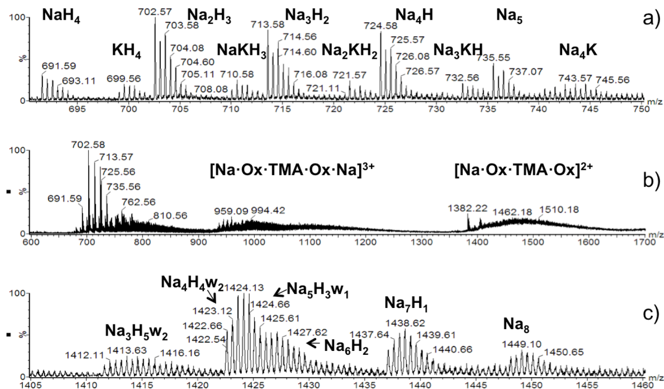
Fig. 2 ESI-MS spectra of OX63. a) Doubly charged monomers observed by injecting a 15 \mu\text{M} solution of OX63 in 7.5 \mu\text{M} TMA. The number and type of cations is indicated. b) Detail of TMA-stabilized dimers observed in the same sample. Dimers with +3 and +2 charges are indicated. Ox refers to the neutral species with 3 sodium ions. Thus the number of sodium ions in the 3+ species is 8 and in the 2+ species is 7. c) Doubly charged dimers extracted from ion-mobility edited ESI-MS spectra of a 1 mM OX63 solution in water. The number and type of cations and the presence of included water molecules (w) is indicated (see also Table 1).
