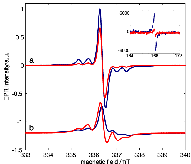
Fig. 5 X-band CW-EPR spectra of a 1:1 glycerol:D 2 O solution of 1M TMA and 30 mM OX63 measured at 2.8 K using a microwave power of (a) 1 \mu W and (b) 1 mW. The spectra were obtained directly after cooling to 2.8 K (blue), or after a 30 minutes annealing at 5 K and subsequent cooling to 2.8K (red) and are normalized with the maximum intensity of the non-annealed spectra set to unity. The high power spectra have been offset for clarity. The inset shows the corresponding half-field EPR signal recorded with a microwave power of 200 \mu W.
