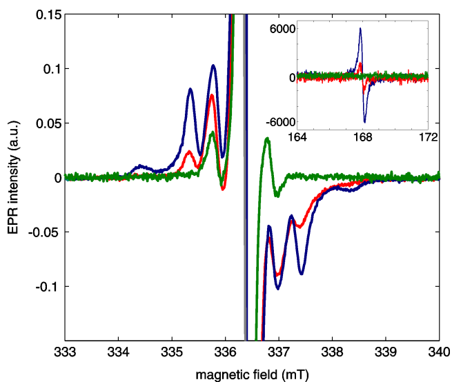
Fig. 3 X-band CW-EPR spectra of 1M TMA and 30 mM OX63 (blue), 15 mM OX63 (red) and 1.5 mM OX63 (green) solutions in 1:1 glycerol:D 2 O. The spectra were recorded with a microwave power of 250 nW. The spectra of the 30 mM OX63 and 15 mM OX63 are recorded at 2.8 K, while that of the 1.5 mM OX63 solution was recorded at 10K due to severe saturation effects at lower temperatures. The inset shows the corresponding half-field signal recorded for all solutions with a microwave power of 200 \mu W at 2.8 K. The spectra are shown normalized, with the intensity of the central band set to unity, and shifted to the same central magnetic field position such as to compensate differences in microwave frequency and facilitate comparison.
