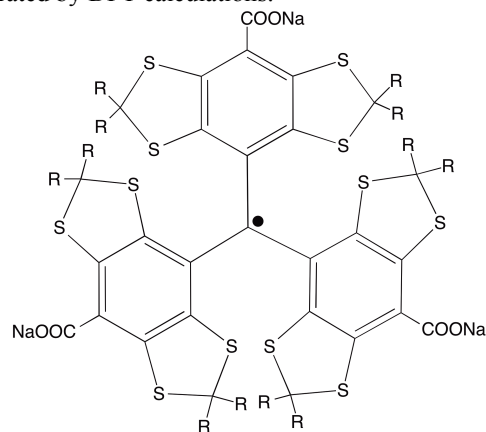
Scheme 1 Structure of OX63 radical (R=CH 2 CH 2 OH).
