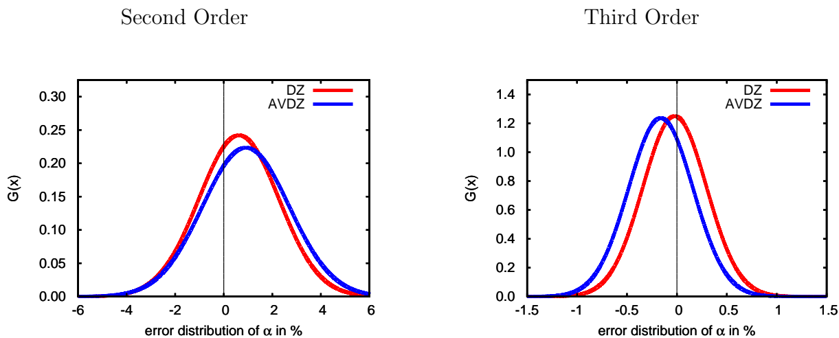
Figure 4: Comparison of the errors due to the incremental expansion of the CCSD polarizabilities for the cc-pVDZ (DZ) and aug-cc-pVDZ (AVDZ) basis sets using Gaussian distributions for the small-molecule test set. The inclusion of diffuse basis functions shifts the second-order errors up by 0.27% and the third-order down by 0.14%.
