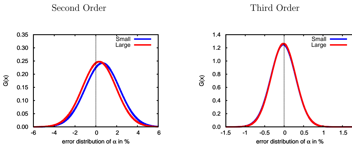
Figure 3: Gaussian distributions of the errors in the second-order (left) and third-order (right) incremental scheme in the CCSD/cc-pVDZ polarizabilities for the full test set of 47 molecules and for a subset of 23 smaller molecules. The distributions are very similar for both test sets indicating that the smaller set may be used to study basis-set effects.
