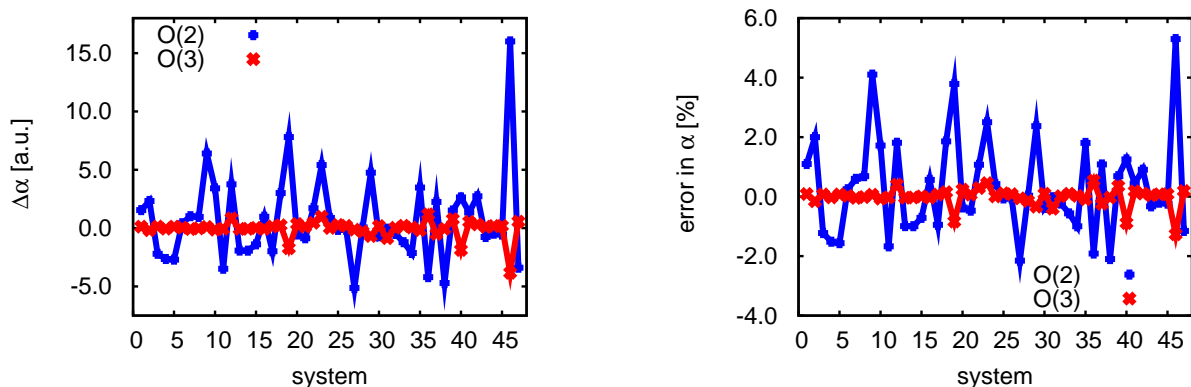
Figure 2: Absolute errors (a.u., left) and relative errors (% , right) in the CCSD/cc-pVDZ polarizabilities of the full test set of 47 systems, ordered by increasing correlation energy. Errors in the second- and third-order expansions are given in blue and red, respectively.
