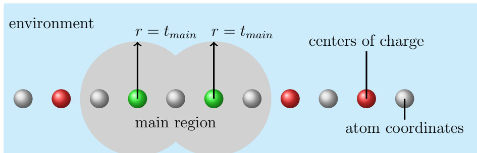
Figure 1: Construction of the domain-specific basis set. The centers of charge of a domain are given in green, and the most important region of a domain is given by the grey area. The area is defined by the union of the circles with the radius t_{\text{main}} around every center of charge in a domain (green circles). The large basis set is applied in the main region and the small basis set in the rest of the system.
