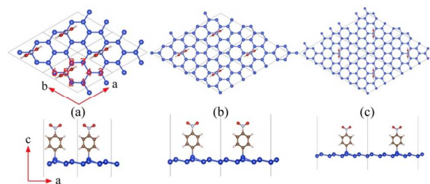
Fig. 1. Optimized structure of (a) NPD-1/8, (b) NPD-1/18, and (c) NPD-1/32 systems. The blue, brown, silver, red and pink spheres denote silicon, carbon, nitrogen, oxygen and hydrogen atoms, respectively.
