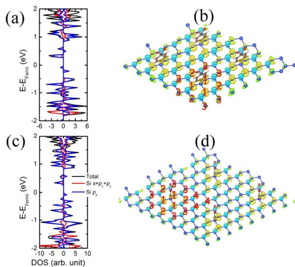
Fig. 3. (a) Computed spin-polarized projected density of states (pDOS) of NPD-1/18, and (b) isosurface of the spin density of NPD-1/18 with an isovalue of 0.003 \text{ e/Bohr}^3 . (c) Computed spin-polarized projected density of states (pDOS) of NPD-1/32, and (d) isosurface of the spin density of NPD-1/32 with an isovalue of 0.003 \text{ e/Bohr}^3 . Number 1-4 labeled in the spin density plot (d) refer to the nearest, second-, third- and fourth-nearest neighboring Si sites from the Si-site bonded with a NPD functional group.
