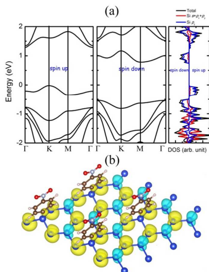
Fig. 2. (a) Computed spin-polarized band structures and density of states (DOS) for the NPD-1/8 system, where \Gamma = (0.0, 0.0, 0.0) , K = (1/3, 1/3, 0) , M = (0.5, 0.0, 0.0) refer to the special points in the first Brillouin zone. The Fermi level is set to 0 eV. (b) Iso-surface of spin-density of NPD-1/8, with an isovalue of 0.003 e/Bohr 3 . The yellow and cyan colors refer to spin-up and spin-down density, respectively.
