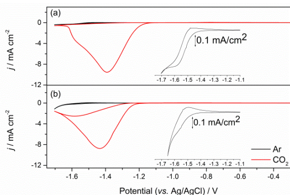
Figure 2: CV of ca. 1 mM solutions of 1 (a) and 2 (b) recorded in 0.1 M NaClO 4 at pH 5 purged with either argon (black line) or CO 2 (red line) recorded at 100 mV s -1 using a HMDE electrode (0.023 cm 2 ). The inset shows an expansion of the Ni II/I couple under argon, see also figure S4.
