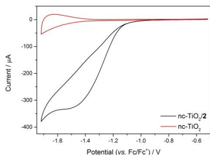
Figure 4: Cyclic voltammograms of nc-TiO 2 (red) and nc-TiO 2 /2 (black) under argon in 0.1 M (But) 4 NPF 6 /MeCN. v = 100 \text{ mV s}^{-1} .
