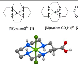
Figure 1: (a) [Ni(cyclam)] 2+ (1) was functionalised on the carbon backbone with a carboxylic acid group to yield (2) for anchoring to metal oxide electrodes. (b) X-ray structure of 2. H atoms, except for those bound to N or O, are omitted for clarity (details in ESI).
