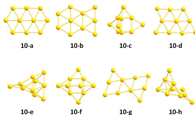
Fig. 10 Structures of Au 10 below 0.4 eV from the predicted GM ( 10-a ) as obtained from the DFT-based pool-GA global optimisation approach. The nomenclature of the individual isomers is sorted by increasing energy at the pwSCF/PBE level of theory.
