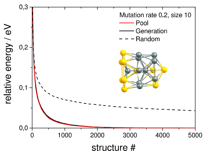
Fig. 5 Comparison of averaged evolutionary progress plots for the generation based GA and the single pool-GA for a population size of 10 using a mutation rate of 0.2 and an exchange rate of 0.5. The GM structure of the \text{Au}_{10}\text{Pd}_{10} cluster at the Gupta potential level is embedded.
