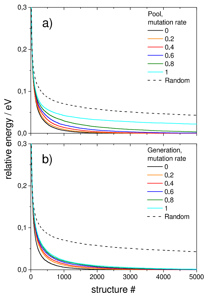
Fig. 7 Influence of the mutation rate on the averaged evolutionary progress plots averaged over 1000 GA runs for of a) A single pool-GA subprocess and b) The generation based GA for a constant size of 10 compared to a random structure search as an internal standard. Mutation reduces the efficiency of finding the GM.
