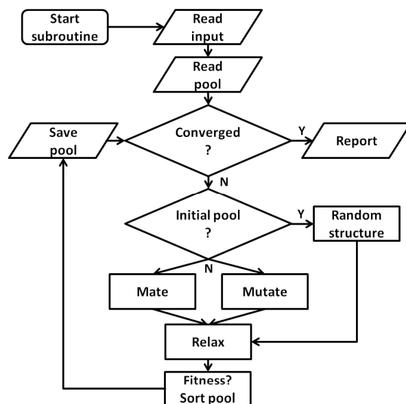
Fig. 3 The genetic operators are applied by the subprocesses on the members of this pool. The flowchart diagram shows how a single pool subprocess works independently from other instances, while all subprocesses communicate with the global database.
