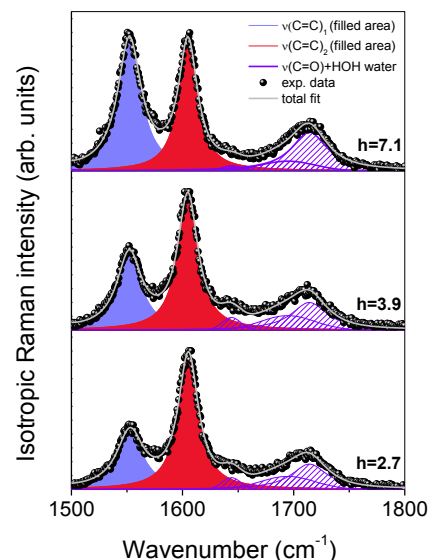
Figure 3: Some representative results of fitting procedure of isotropic Raman profile for \beta -CDPMA14 hydrogel at different hydration levels h (black symbols). The total fit curve (grey line) is reported, together with the single components: nanosponge stretching modes \nu(\text{C}=\text{C})_1 (periwinkle filled area) and \nu(\text{C}=\text{C})_2 (red filled area), stretching mode of polymer carbonyl groups and HOH bending mode of water (violet).
