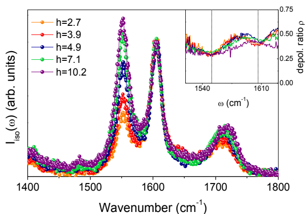
Figure 2: Isotropic Raman profiles of \beta -CDPMA14 hydrogel at different hydration levels h in the spectral range 1400\text{--}1800\text{ cm}^{-1} . Inset: depolarization ratio \rho reported in the restricted spectral range 1520\text{--}1630\text{ cm}^{-1} .
