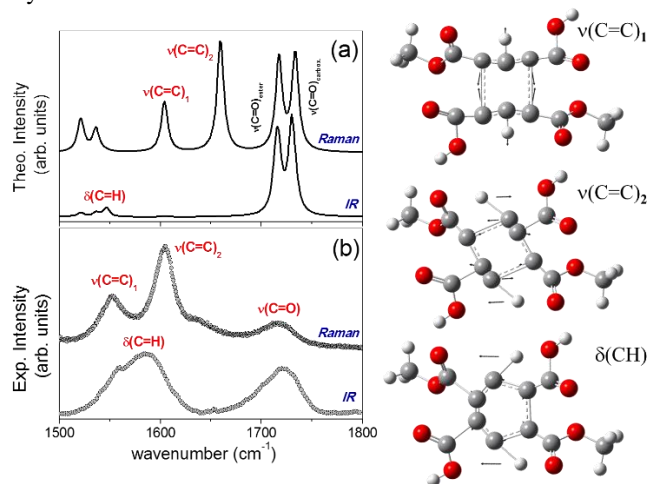
Figure 1: Theoretical (a) and experimental (b) Raman and IR profiles of \beta -CDPMA14 nanosponge in the dry state and in the spectral range 1500-1800 \text{cm}^{-1} . Right Panel: schematic picture of the vibrational modes obtained for simulated bridging molecule, namely \nu(\text{C}=\text{C})_1 , \nu(\text{C}=\text{C})_2 , and \delta(\text{C}=\text{H}) .
