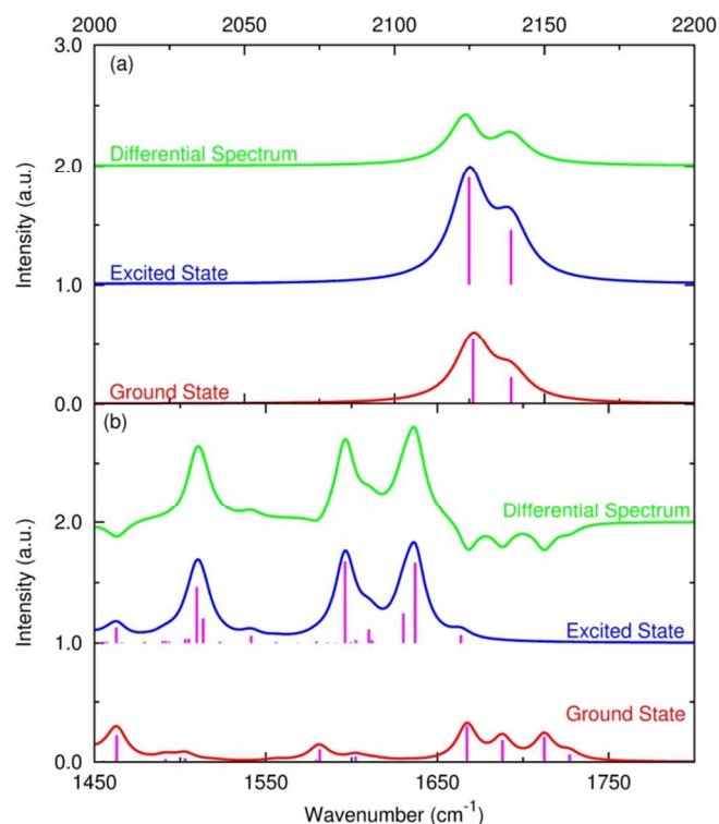
Figure 11. Calculated IR spectra of ground singlet and lowest triplet state of 1 , including TRIR spectrum. Panel (a) shows the acetylide stretch region (scaling 0.97). Intensity scaled by 500 for ease of presentation. Panel (b): Fingerprint region between 1450 and 1800 \text{cm}^{-1} (scaling 0.98). Intensity scaled by 3000 for ease of presentation.
