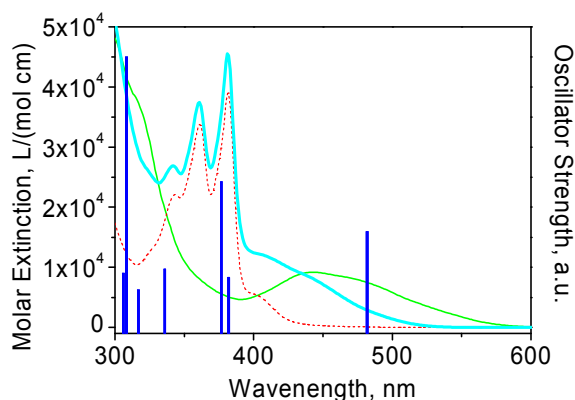
Figure 1. Ground state electronic absorption spectra of 1 (thick solid blue line), 2 (thin solid green line), and 3 (dashed red line) in \text{CH}_2\text{Cl}_2 at r. t. Blue vertical bars represent main transitions of calculated absorption spectrum for 1 .
