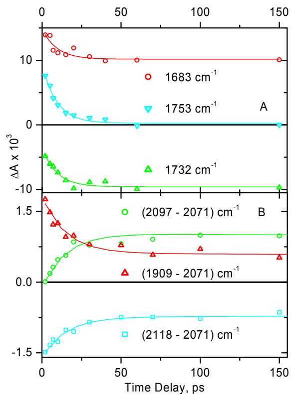
Figure 7. Representative decay traces obtained in time-resolved infrared experiments for 2 in \text{CH}_2\text{Cl}_2 . Markers show the experimental data, the corresponding fitting curves are shown by solid lines. Panel A: spectral data in the region of \nu(\text{C}=\text{O}) stretch. The data were fitted with a single-exponential function (plus a long-lived signal) with a lifetime 9.3 \pm 1.0 ps. Panel B: spectral data in the region of \nu(\text{C}\equiv\text{C}) . The decay traces shown are plotted as a difference between the indicated spectral points to emphasize the charge separation step. The data were fitted with a dual-exponential function with lifetimes \tau_1 = 15 \pm 2 ps and \tau_2 = 4.8 \pm 2.0 ns.
