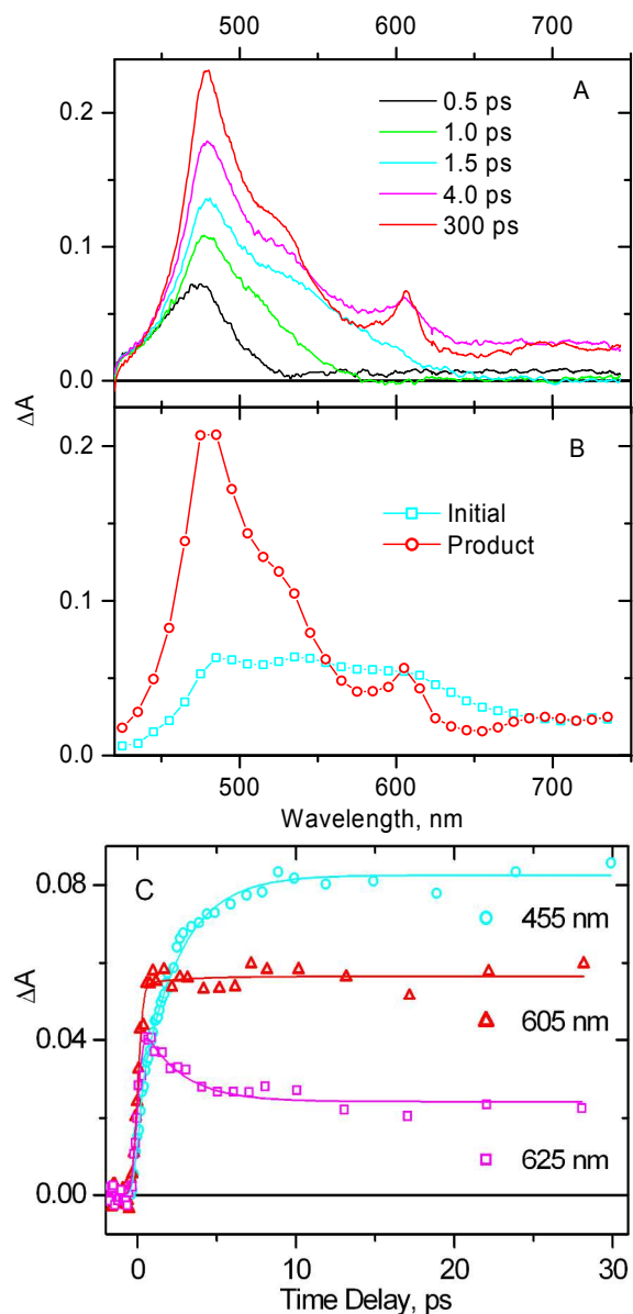
Figure 9. (A) Representative transient absorption spectra at selected time delays obtained for 1 in \text{CH}_2\text{Cl}_2 , following excitation with a 395 nm, 150 fs laser pulse. The observed spectral dynamics is convolved with the chirp of a probe pulse, that was corrected by the data analysis with the results shown on Panel B. (B) Reconstructed transient spectra of the two excited states involved into the spectral evolution, assuming a consecutive reaction scheme “A→B”. (□) the initial excited state populated immediately after the photoexcitation, (○) the successor excited state populated from the former one. (C) Representative transient absorption decay traces. Markers show the experimental data, the corresponding fitting curves are shown by solid lines. The lifetime obtained in single-exponential (plus long-lived component) global fit is 2.5 \pm 0.3 ps.
