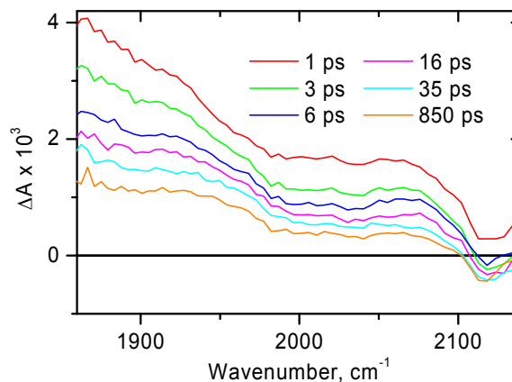
Figure 8. Time-resolved infrared spectra at selected time delays for 4 in \text{CH}_2\text{Cl}_2 following excitation with a 400 nm, 150 fs laser pulse in the region of \text{C}\equiv\text{C} stretch.
