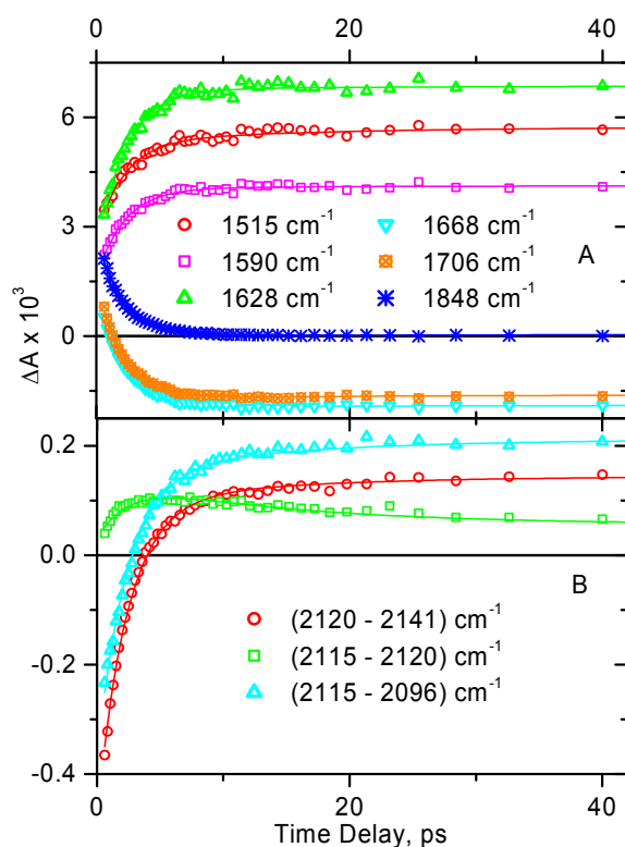
Figure 4. Representative decay traces obtained in time-resolved infrared experiments for 1 in \text{CH}_2\text{Cl}_2 . Markers show the experimental data, the corresponding fitting curves are shown by solid lines. Panel A: in the spectral window 1450-2000 \text{cm}^{-1} . The data were globally fitted with a bi-exponential function (plus a long-lived signal) with lifetimes \tau_1=2.0\pm0.5 ps and \tau_2=15\pm3 ps. Panel B: spectral data in the region of \nu(\text{C}\equiv\text{C}) . The decay traces shown are plotted as a difference between the indicated spectral points to emphasize the charge separation step. The data were globally fitted with a bi-exponential function (plus a long-lived signal) with lifetimes \tau_1=2.3\pm0.5 ps and \tau_2=14\pm2 ps.
