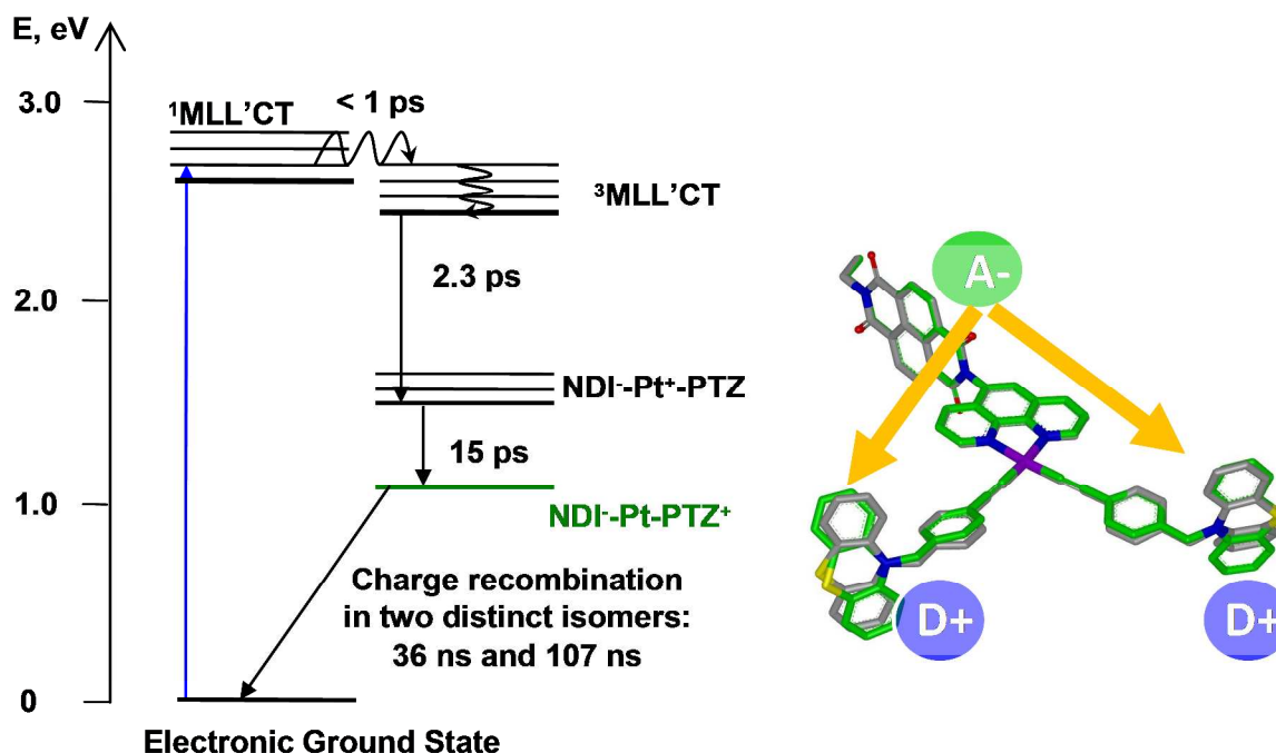
Scheme 2. Photophysical diagram for 1 in \text{CH}_2\text{Cl}_2 , following excitation with 400 nm, 50 – 150 fs laser pulse. Shown on the right-hand side is the overlay of the T_1 (grey bonds) and T_2 (green bonds) triplet states in 1 .
