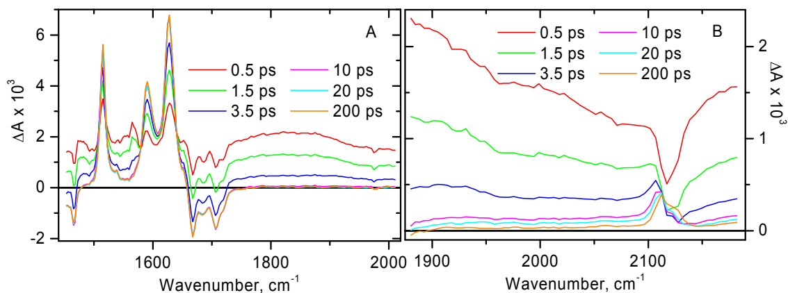
Figure 3. Time resolved infra-red spectra at selected time delays for 1 in \text{CH}_2\text{Cl}_2 after excitation with a 400 nm, 50 fs laser pulse. A: spectral data in the region of C=O stretch. B: spectral data in the region of C≡C stretch. Note the different intensity scales of Panels A & B.
