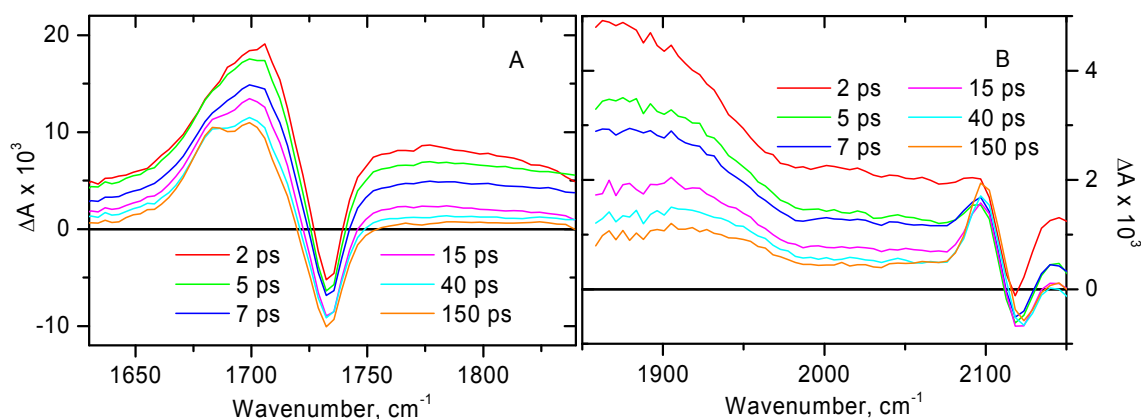
Figure 6. Time-resolved infrared spectra at selected time delays for 2 in CH 2 Cl 2 following excitation with a 400 nm, 150 fs laser pulse. Panel A: spectral data in the region of ν(C=O). Panel B: spectral data in the region of ν(C≡C). Note the different intensity scales of A & B.
