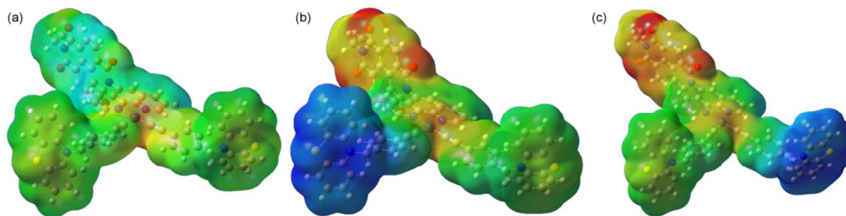
Figure 12. Electrostatic Potential Map for the ground singlet [panel (a)] and lowest triplet state with the hole localised either on one PTZ group [panel (b)] or the other PTZ group [panel (c)]. The configuration shown in (b) is 1.118 \text{kJ mol}^{-1} lower in energy than the one in (c). Colours correspond to charges with red being -0.1 and blue being +0.1.
