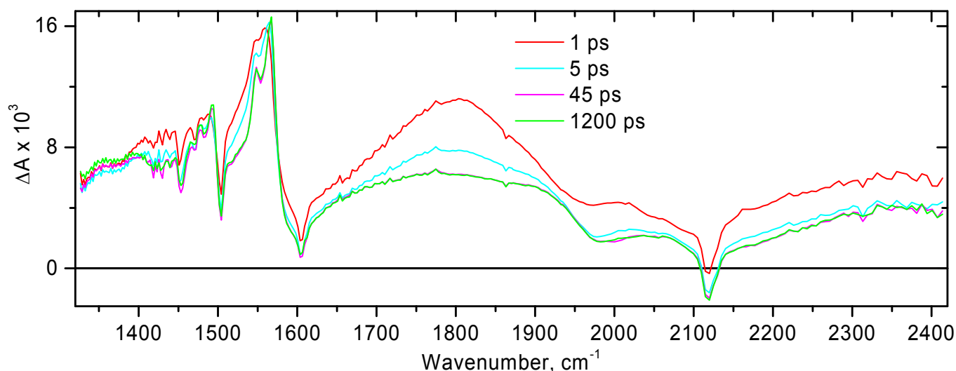
Figure 5. Time resolved infra-red spectra at selected time delays for (bpy)Pt(C≡C-C 7 H 15 ) 2 in CH 2 Cl 2 after excitation with a 400 nm, 50 fs laser pulse. Presented spectra were obtained in separate spectral windows over the range 1300-2450 cm -1 and combined afterwards.
