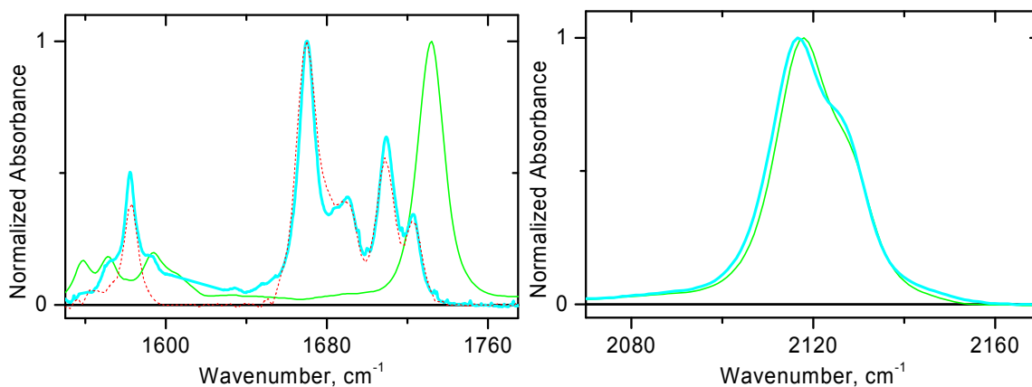
Figure 2. FTIR spectra in \text{CH}_2\text{Cl}_2 at r. t. Left panel: 1550\text{--}1775\text{ cm}^{-1} region for 1 (thick solid blue line), 2 (thin solid green line), and 3 (dashed red line). Right panel: 2070\text{--}2170\text{ cm}^{-1} region for 1 (thick solid blue line) and 2 (thin solid green line).
