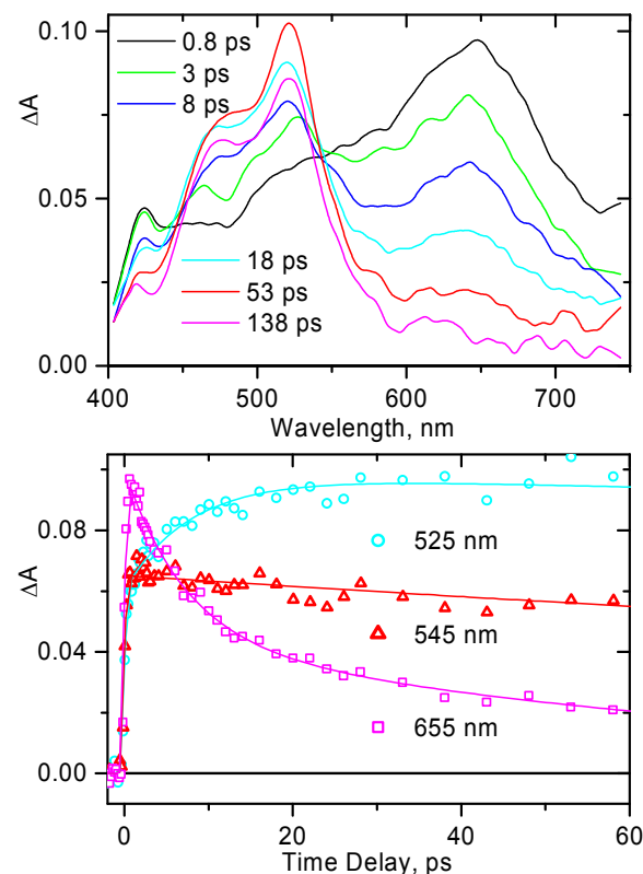
Figure 10. Representative transient absorption spectra (top) and selected decay traces (bottom) obtained for 2 in \text{CH}_2\text{Cl}_2 , following excitation with a 395 nm, 150 fs laser pulse. For kinetic traces, markers show the experimental data, the corresponding fitting curves are shown by solid lines. The rise of the signal of PTZ anion at 525 nm and main decay component of ^3\text{MLL}^{\text{CT}} band at 655 nm occur with identical lifetime of 8 \pm 2 ps.
