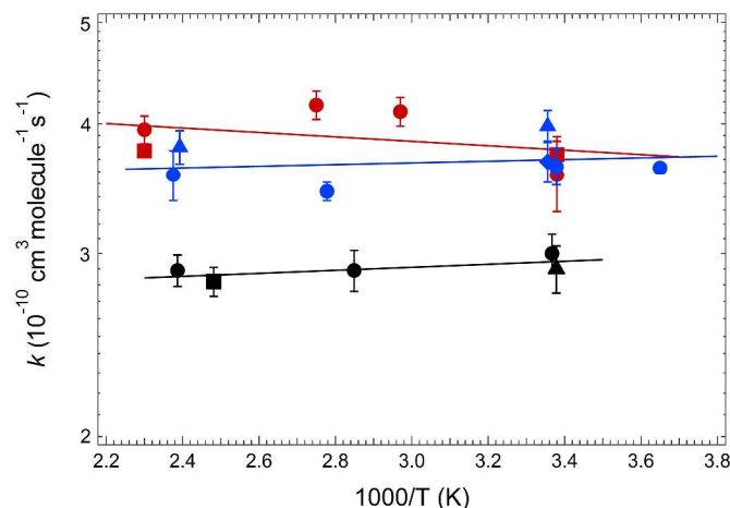
Figure 3. Arrhenius plots for \text{Cl}(^2\text{P}_j) reactions with \text{CH}_3\text{NH}_2 (R1, black), (\text{CH}_3)_2\text{NH} (R2, red), and (\text{CH}_3)_3\text{N} (R3, blue). Solid lines are obtained from linear least-squares analyses of the unweighted \ln k_{\text{Ri}} versus T^{-1} data; the best fit Arrhenius expressions in units of 10^{-10} \text{ cm}^3 \text{ molecule}^{-1} \text{ s}^{-1} are k_{\text{R1}} = 2.63 \exp(+33/T) , k_{\text{R2}} = 4.46 \exp(-49/T) , and k_{\text{R3}} = 3.47 \exp(+18/T) . Error bars are 2\sigma , precision only.
