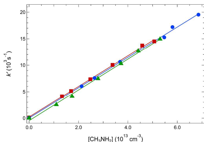
Figure 2. Plots of k' versus [\text{CH}_3\text{NH}_2] for data obtained at different temperatures and pressures. Solid lines are obtained from linear least-squares analyses and
