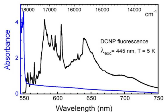
Figure 2. Absorption (blue line) and fluorescence (black line) spectra of a ~2.5 mm thick single crystal of DCNP recorded at 5 K. No correction of absorbance due to light reflection from sample surface has been applied.
