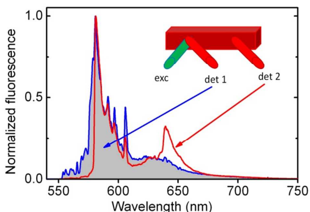
Figure 4. Fluorescence spectra of DCNP single crystal recorded at T = 5 K "on-spot" (blue line, det 1) and "off-spot" 1 mm aside (red line, det 2). The DCNP crystal was excited by a 445 nm laser light; both spectra were normalized at maximum.
