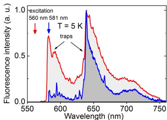
Figure 3. Fluorescence spectra of DCNP crystal at 5 K obtained with the excitation wavelengths of 560 and 581 nm, respectively.
