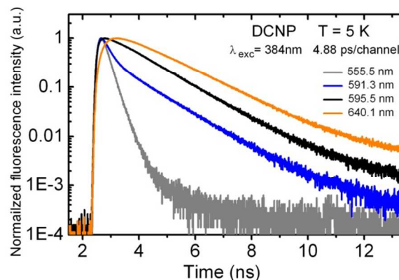
Figure 5. Fluorescence decay profiles of DCNP single crystal at temperature 5 K excited with 384 nm picosecond laser pulses and measured at 555.5 nm (excitonic emission region), 591.3, 595.5 nm (shallow trap 875\text{ cm}^{-1} emission region) and 640.1 nm (deeper trap 2465\text{ cm}^{-1} emission region).
