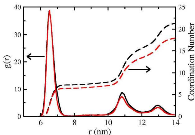
Figure 4. Radial distribution functions (solid lines) and coordination numbers (dashed lines) for the center of mass of the NPs. The black lines stand for
