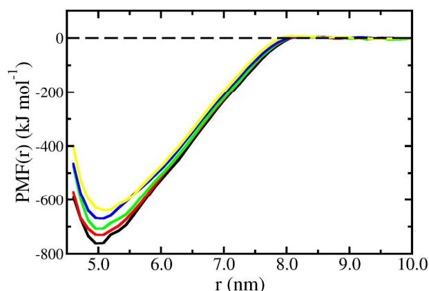
Figure 11. Jarzynski average for the PMF along the association/dissociation profile for a pair of NPs in vacuum at different temperatures. (black line) 290 K; (red line) 295 K; (green line) 300 K; (blue line) 305 K; (yellow line) 310 K.
