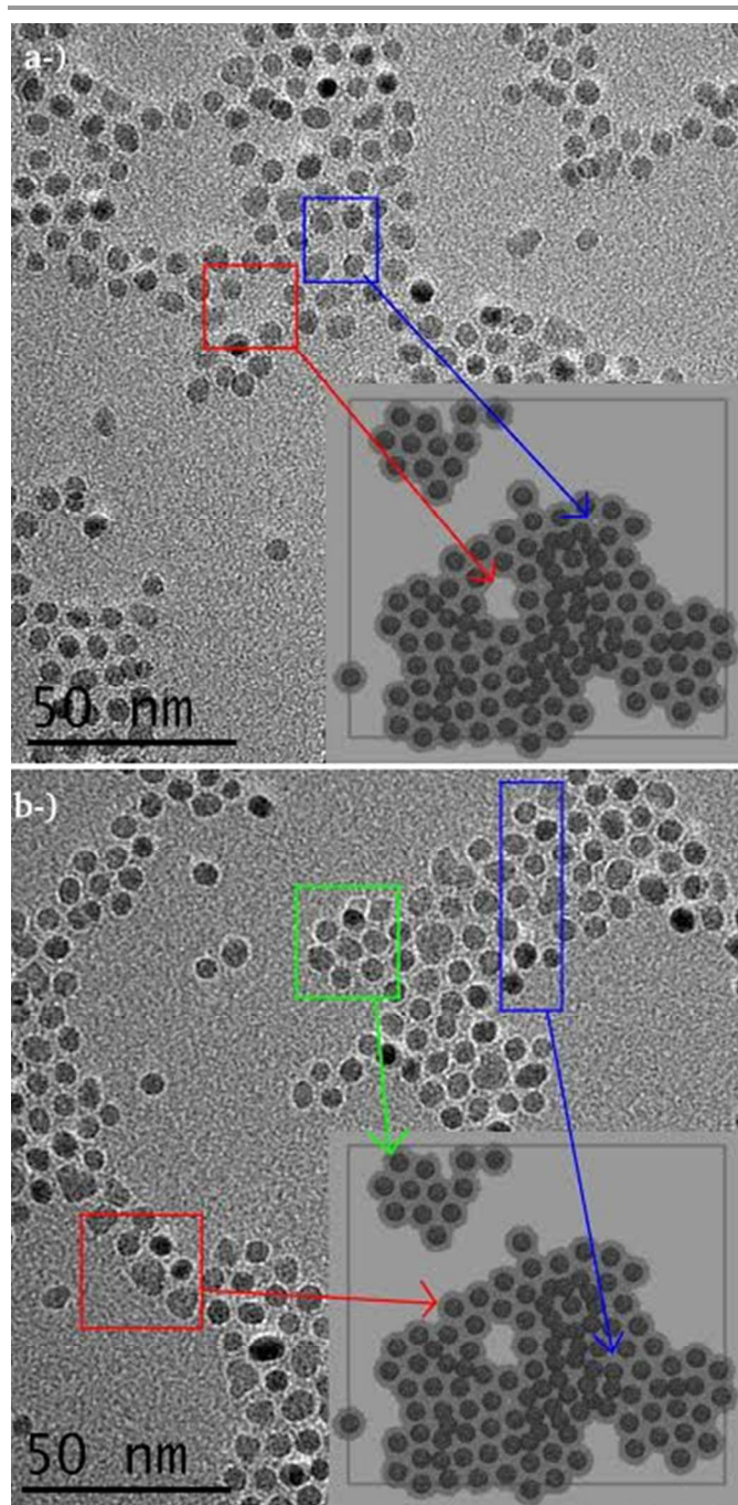
Figure 7. Comparison between the TEM analysis (larger background images) and the final structure obtained in the thin film simulation (smaller inset images), highlighting similar patterns (all images are drawn in the same scale). (a) holes in the main structure; and (b) filaments of similar size and shape. Simulation images depict the NPs cores as solid spheres and the organic capping as shaded areas around the cores.
