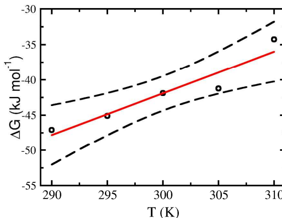
Figure 10. Gibbs energy of aggregation for a pair of NPs in chloroform. The solid red line stands for the linear regression whereas the dashed black lines stand for the confidence interval of the regression.
