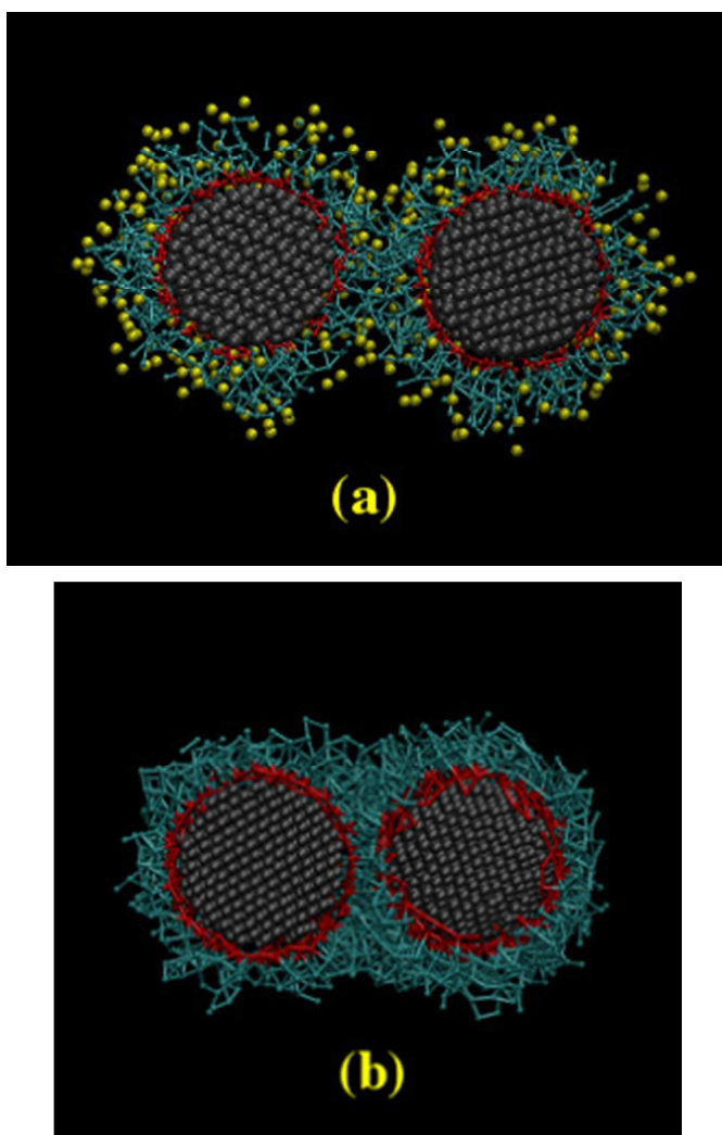
Figure 12. Cross section view of the NP pair at the distance of minimum Gibbs energy along the PMF profile ( T=300 \text{ K} ) in chloroform (a) and in vacuum (b). Solvent molecules within 0.5 nm of any NP site are shown in yellow at (a).
