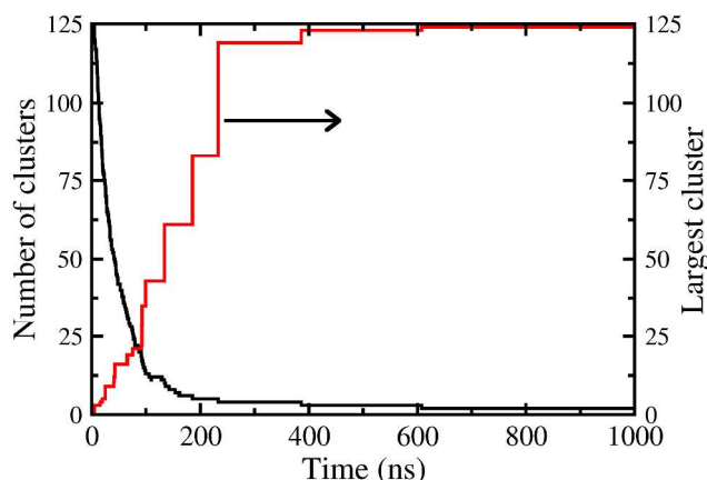
Figure 3. Time evolution of the number of clusters (black line) and the size of the largest cluster (red line).
