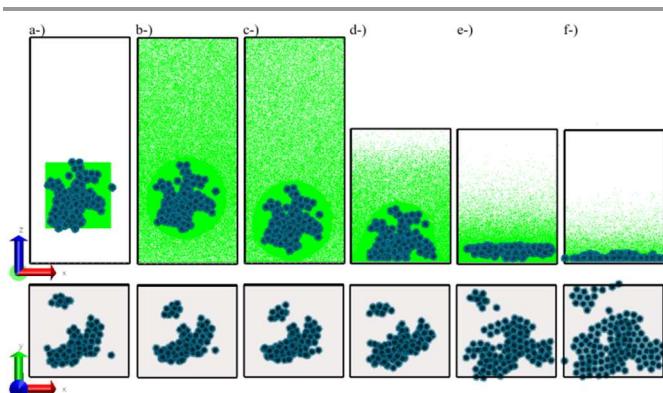
Figure 6. Graphical representations of selected structures along the relaxation of the liquid suspension droplet and the drying process of the solvent. Solvent molecules are rendered in green in the top view, along with nanoparticles (blue) and the solid substrate (silver). The bottom representations omit the solvent for clarity and present the nanoparticles rendered as solids spheres (solid core) surrounded by a shaded area (capping organic ligands). a-) final structure obtained from the bulk simulation placed in the middle of the larger box; b-) droplet relaxation and initial solvent evaporation; c-) first contact of the droplet with the substrate and starting point for the drying process; d-) intermediate point of droplet spreading over the substrate; e-) complete spreading of the liquid suspension; f-) removal of most of the solvent. The edge length of the simulation box in the z -direction was decreased after the start of the drying process in order to improve the computational efficiency.
