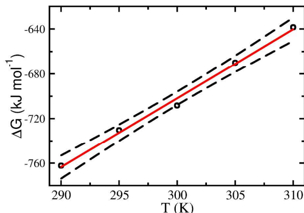
Figure 13. Gibbs energy of aggregation for a pair of NPs in vacuum. The solid red line stands for the linear regression whereas the dashed black lines stand for the confidence interval of the regression.
