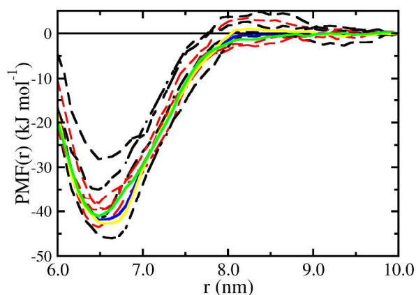
Figure 8. Work profiles for the association (dashed black curves) and the dissociation (dashed red curves) of a pair of NPs in chloroform. Solid lines stand for the Jarzynski average of the association processes (yellow curve), the dissociation processes (green curve) and the overall average (blue curve).
