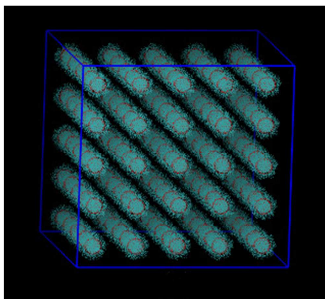
Figure 2. Initial structure for the colloidal suspension model system. Solvent molecules are not shown for clarity.
