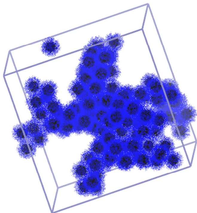
Figure 5. Structure of the NPs after 1000 ns (solvent molecules are not shown for clarity).
