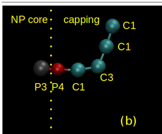
Figure 1. (a) Graphical representation of the NP cross section. The NP core is 4.0 nm wide (dark gray sites) and the surface is completely covered by a dense monolayer of oleic acid molecules (polar heads are shown in red, whereas the apolar tail sites are shown in gray). (b) Type of interaction for each site comprising the NP core and the organic capping.
