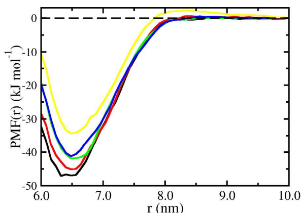
Figure 9. Jarzynski average for the PMF along the association/dissociation profile for a pair of NPs in chloroform at different temperatures. (black line) 290 K; (red line) 295 K; (green line) 300 K; (blue line) 305 K; (yellow line) 310 K.
