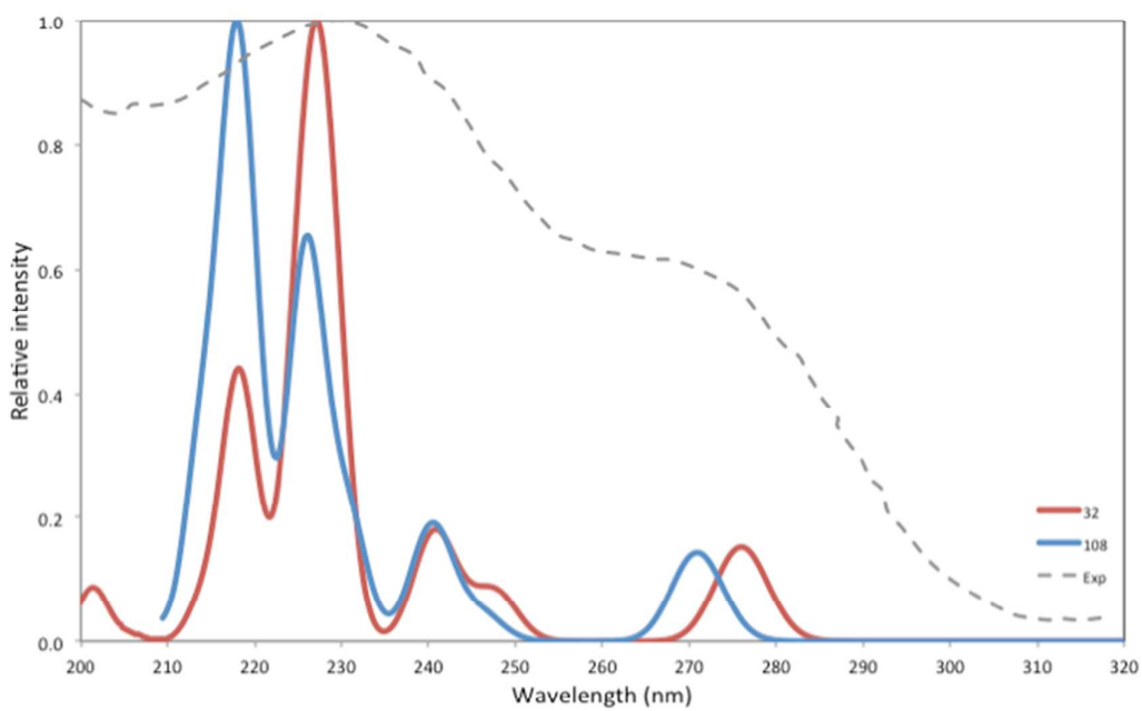
Fig. 8 TD-BHLYP/DZ(D)P calculated absorption spectra (including the 0.5 eV rigid red-shift discussed in the text) of (\text{MgO})_{32} and (\text{MgO})_{108} . Experimental absorption spectrum of 3 nm particles, taken from ref. 5, included for comparison.
