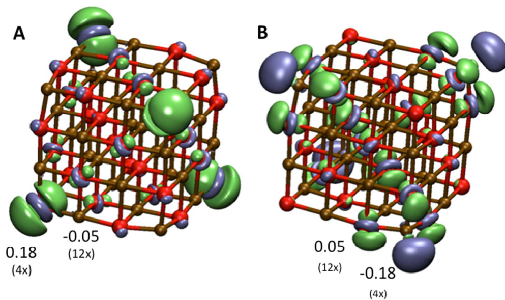
Fig. 9 TD-BHLYP excited state – ground state density difference for the excitations corresponding to the 270 (A) and 230 (B) nm peaks of (\text{MgO})_{32} (blue, excess of electrons in the excited state; excited electron/ green, deficit of electrons in the excited state; hole). The numbers indicate the most significant differences in NBO charge of the excited state and ground state charge, as well as the multiplicity of each site.
