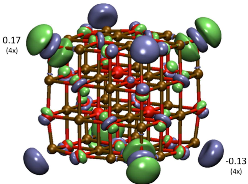
Fig. 10 TD-B3LYP excited state – ground state density difference for the excitations corresponding to the 350 nm charge-transfer peak of (MgO) 32 (blue, excess of electrons in the excited state; excited electron/ green, deficit of electrons in the excited state; hole). The numbers indicate the most significant differences in NBO charge of the excited state and ground state charge, as well as the multiplicity of each site.
