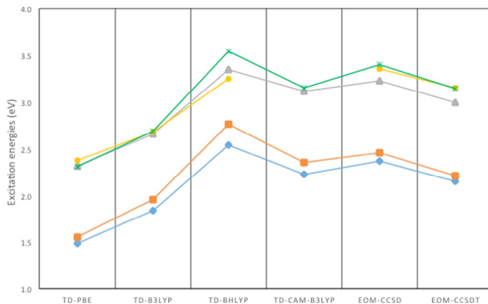
Fig. 2 Excitation energies of the five lowest excitations of the (\text{MgO})_2 cluster as calculated using TD-DFT and EOM-CC. Blue diamonds 1-^1b_{1g} state, orange square 1-^1b_{3u} state, green crosses 1-^1b_{1u} state, yellow circles 1-^1a_{1u} state, and grey 1-^1b_{1g} state.
