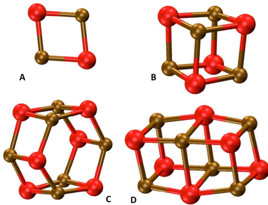
Fig. 1 DFT optimised structures of A (MgO) 2 , B (MgO) 4 , C hexagonal (MgO) 6 and D hexagonal (MgO) 6 particles.
