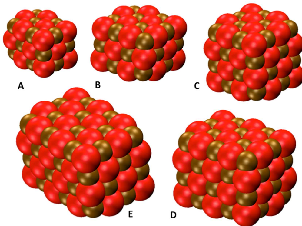
Fig. 4 DFT optimised structures of A (MgO) 18 , B (MgO) 24 , C (MgO) 32 , D (MgO) 40 and E (MgO) 48 particles.
