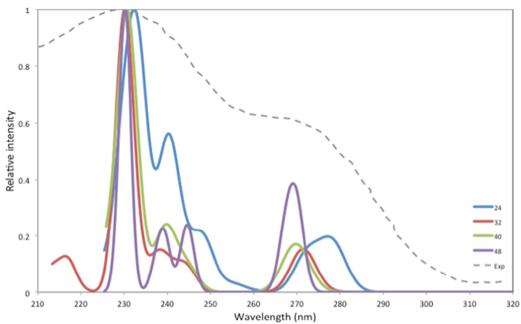
Fig. 7 TD-BHLYP calculated absorption spectra (including the 0.5 eV rigid red-shift discussed in the text) of (\text{MgO})_{24} , (\text{MgO})_{32} , (\text{MgO})_{40} and (\text{MgO})_{48} . Experimental absorption spectrum of 3 nm particles, taken from ref. 5, included for comparison.
