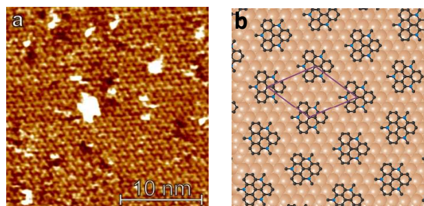
Figure 5. (a) STM image ( 25 \times 25 nm 2 ) of a methoxy-azo-TATA adlayer on Au(111), (b) schematic model of a (\sqrt{19} \times \sqrt{19})R23.4^\circ superstructure, where the C (black) and N (blue) atoms of the platform are shown (hydrogen atoms omitted, only first C atoms of octyl side-chains shown).
