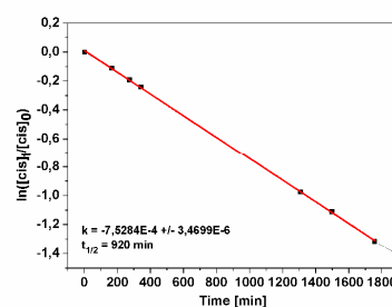
Figure 4. Plot of the natural logarithm of the cis concentration as a function of time to determine the half-life of methoxy-azo-TATA in toluene.
