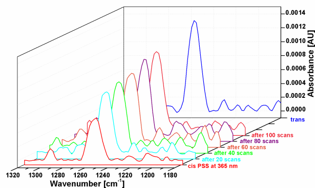
Figure 10. C_{(\text{phenyl})}\text{-O}(\text{Me}) stretching band data of methoxy-azo-TATA monolayer on Au(111) obtained with PM-IRRAS under continuous irradiation with 365 nm (red) and after 20, 40, 60, 80 and 100 scans (cyan, green, brown, violet and orange, respectively) with the LED switched off. The spectrum of trans is shown for comparison (blue).
