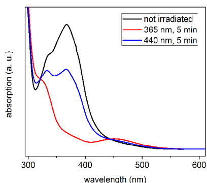
Figure 2. UV spectra of methoxy-azo-TATA in toluene at ambient conditions. Upon irradiation with UV light (365 nm) the \pi\pi^* transition band decreases and the n\pi^* transition band increases in intensity.
