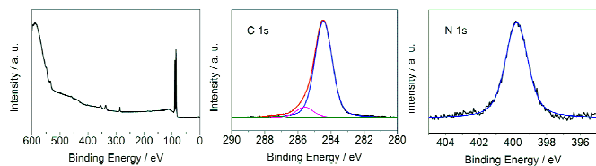
Figure 6. XPS spectra of methoxy-azo-TATA monolayer. Left: survey-spectrum; middle: C 1s- spectrum along with fit (blue: aliphatic and aromatic C, magenta: C connected to N, green: C connected to O); right: N 1s spectrum with fit (blue).
