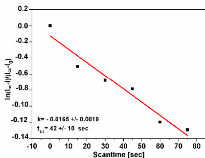
Figure 11. Plot of \ln[(I_c - I)/(I_c - I_0)] vs. time, showing a monoexponential decay of cis to trans with a half-life of 42 \pm 10 sec.
