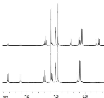
Figure 3. Aromatic region of the 1 H-NMR spectra of methoxy-azo-TATA in trans (bottom) and after irradiation with UV light (365 nm) in cis (top) configuration in toluene at ambient conditions.
