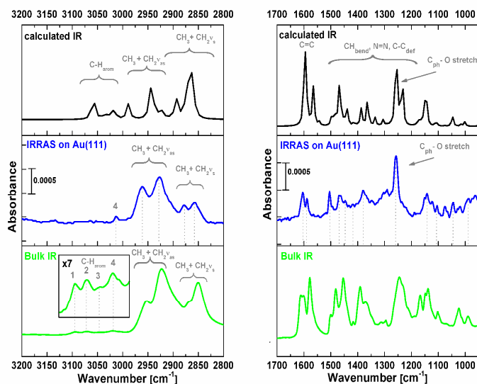
Figure 8. IR data of methoxy-azo-TATA. Left: CH-stretching vibration region, right: fingerprint region. The spectra in the top panels show the calculated, the spectra in the middle in blue the IRRAS of the surface-adsorbed monolayer and the green spectra at the bottom the bulk data. Band numbers correspond to Table S3.
