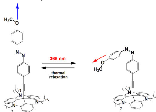
Figure 9. Different orientations of the transition dipole moment of the C-O stretching vibration in trans and cis conformation.
