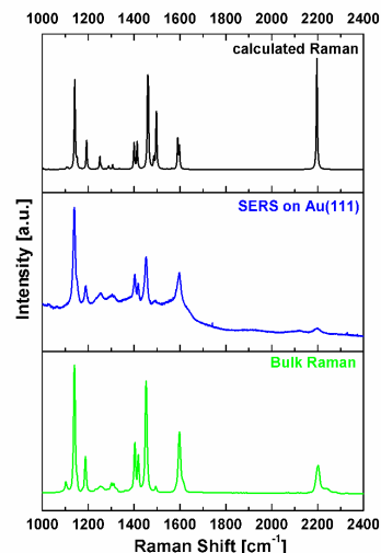
Figure 7. Calculated Raman spectrum (B3LYP/6-31++G** level of DFT) of methoxy-azo-TATA (black), SERS spectrum of methoxy-azo-TATA on Au(111) (blue) and bulk Raman spectrum of methoxy-azo-TATA (green).
