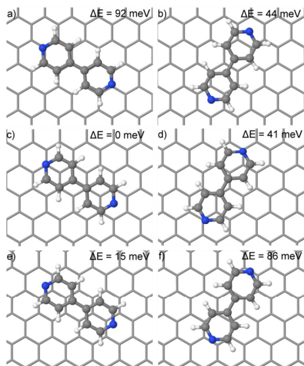
Figure 9. Optimized structures of BPY on graphene. Relative adsorption energies ( \Delta E ) are reported. The most stable adsorption site (c) is for BPY adsorbed with the centre of each ring atop a carbon atom of the substrate.
