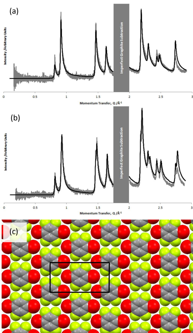
Figure 5. (a) The overlayer diffraction pattern of DBTFB at 0.497 ML coverage and a temperature of 130 - 160 K. The experimental pattern is shown in grey, and the calculated fit in black. (b) The overlayer diffraction pattern of DBTFB at 0.497 ML coverage and a temperature of 100 K. The experimental pattern is shown in grey, and the calculated fit in black. (c) The structure corresponding to the fit in part (a).
