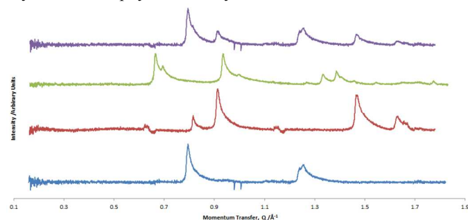
Figure 2. Overlayer diffraction patterns of BPY (blue – bottom), DBTFB (red – second from bottom), the 1:1 mixed co-layer (green – second from top). The pattern expected for phase separation of BPY and DBTFB is shown in purple at the top. All patterns were recorded at a similar coverage and temperature.
