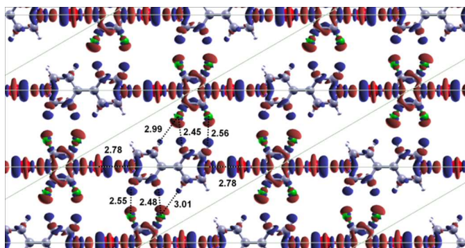
Figure 7. DFT electron density difference for the hypothetical BPY/DBTFB linear monolayer. Red regions show increase of electron density relative to the separate molecules and blue indicates a decrease of electron density relative to the separate molecules (the isosurface level is set to 0.005 \text{ e}/\text{Å}^3 ).
