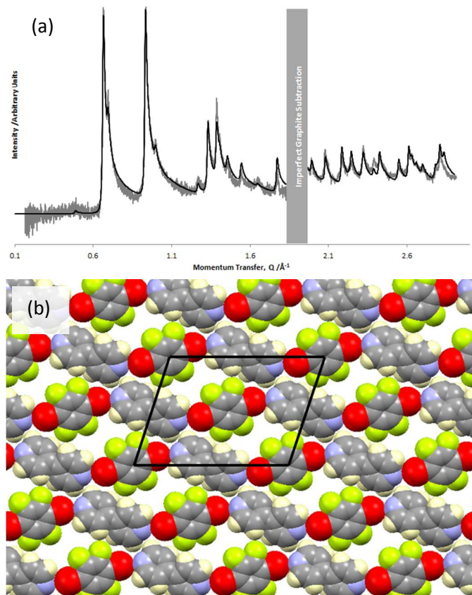
Figure 3. (a) The overlayer diffraction pattern of the 1:1 stoichiometry co-layer of BPY and DBTFB at a coverage of 0.519 ML and a temperature of 200 K. The experimental pattern is shown in grey, and the calculated fit in black. (b) The overlayer structure corresponding to this fit. In this and subsequent figures, atom colours are: grey = carbon, blue = nitrogen, white = hydrogen, green = fluorine, bronze = bromine. The unit cell is shown in black.
