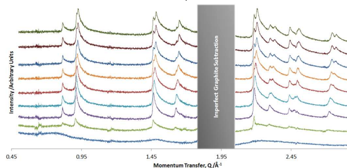
Figure 4. The overlayer diffraction pattern of DBTFB at 0.497 ML coverage at selected temperatures. Temperatures from bottom to top are: 202 K, 177 K, 154 K, 137 K, 125 K, 115 K, 108 K, 103 K, 100 K.
