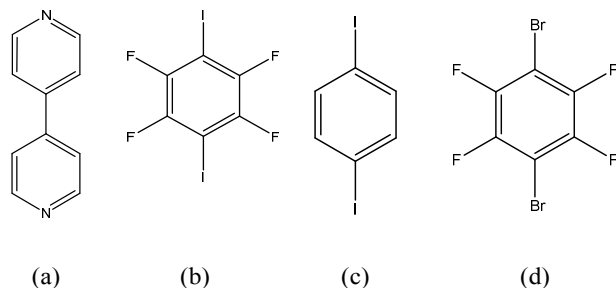
Figure 1. The molecular structure of (a) 4,4'-bipyridine (BPY); (b) 1,4 diiodotetrafluorobenzene (DITFB); (c) 1,4-diiodobenzene (DIB); and (d) 1,4-dibromotetrafluorobenzene (DBTFB).
