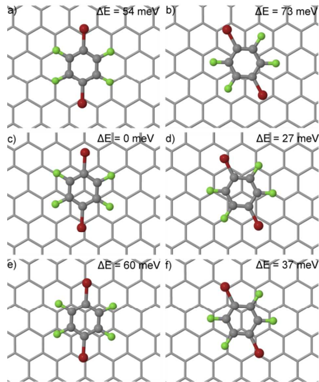
Figure 8. Optimized structures of DBTFB on graphene. Relative adsorption energies ( \Delta E ) are reported. The most stable adsorption site (c) is for DBTFB
