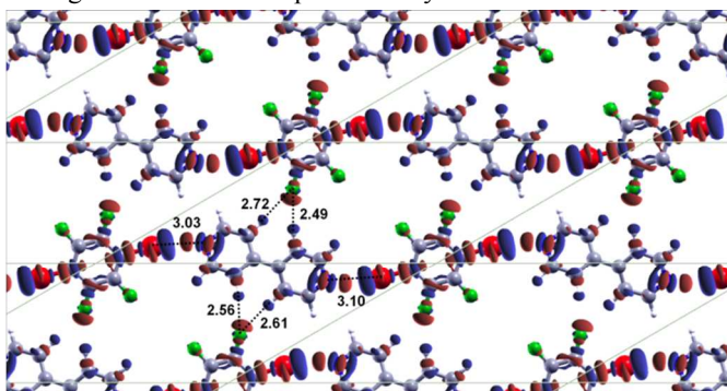
Figure 6 DFT electron density difference for BPY/DBTFB monolayer. Red regions show increase of electron density relative to the separate molecules and blue indicates a decrease of electron density relative to the separate molecules (the isosurface level is set to 0.005 \text{ e/\AA}^3 ). The lines indicate the unit cell.
