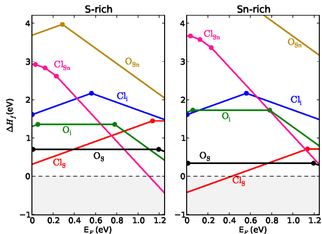
FIG. 5. Calculated defect formation enthalpies for extrinsic defects formed from the elements Cl and O, under S-rich (left) and Sn-rich (right) conditions.
