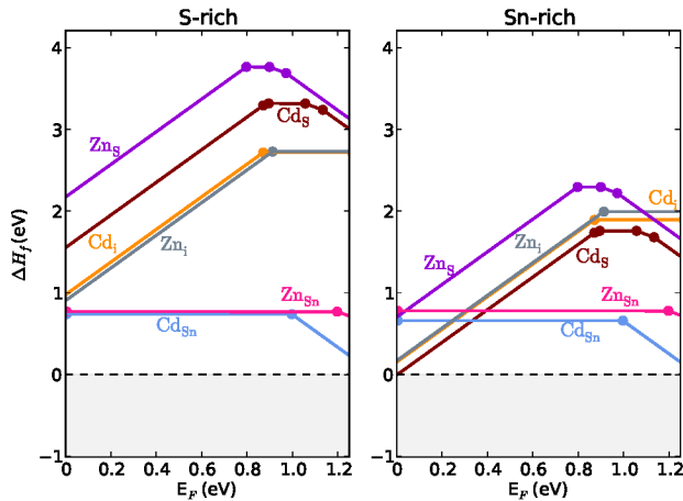
FIG. 8. Calculated defect formation enthalpies for extrinsic defects formed from the elements Zn and Cd, under S-rich (left) and Sn-rich (right) conditions.
