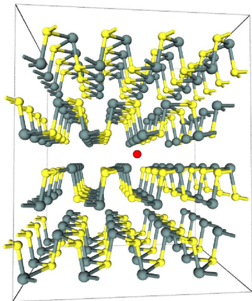
FIG. 1. The SnS supercell, outlined in black lines and containing a total of 256 bulk atoms, used for the calculation of the defect formation energies. Sn atoms are shown in gray, S in yellow, and the site of the interstitial defect is shown in red.
