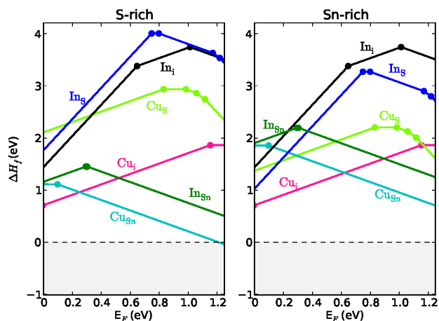
FIG. 7. Calculated defect formation enthalpies for extrinsic defects formed from the elements Cu and In, under S-rich (left) and Sn-rich (right) conditions.
