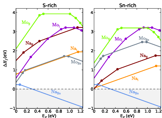
FIG. 6. Calculated defect formation enthalpies for extrinsic defects formed from the elements Na and Mo, under S-rich (left) and Sn-rich (right) conditions.
