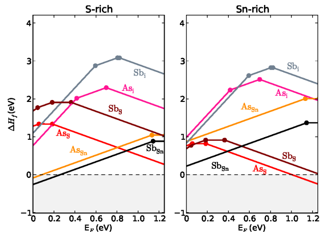
FIG. 4. Calculated defect formation enthalpies for extrinsic defects formed from the group V elements As and Sb, under S-rich (left) and Sn-rich (right) conditions.
