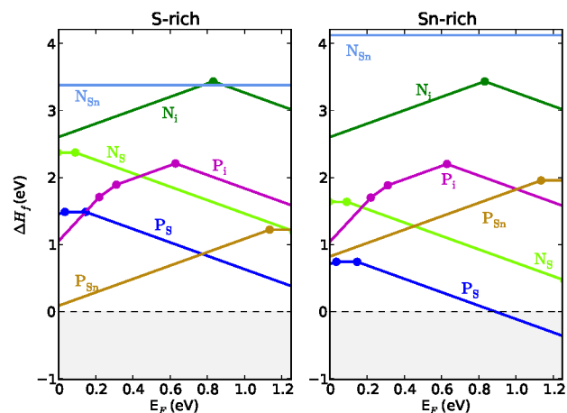
FIG. 3. Calculated defect formation enthalpies for extrinsic defects formed from the group V elements P and N, under S-rich (left) and Sn-rich (right) conditions.
