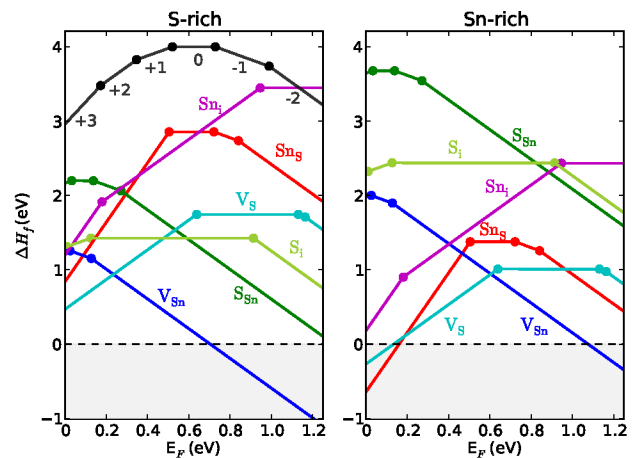
FIG. 2. Calculated defect formation enthalpies for the intrinsic defects under S-rich (left) and Sn-rich (right) conditions. The black segments near the top of the S-rich panel, labeled +3, +2, +1, 0, -1, -2, illustrate how the charge at a particular position of the Fermi energy can be inferred from the slope of the formation enthalpy at that position.
