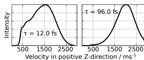
Fig. 7 Final averaged velocity distributions of the desorbed CO molecule for \tau = 12.0 fs and \tau = 96.0 fs, respectively.
