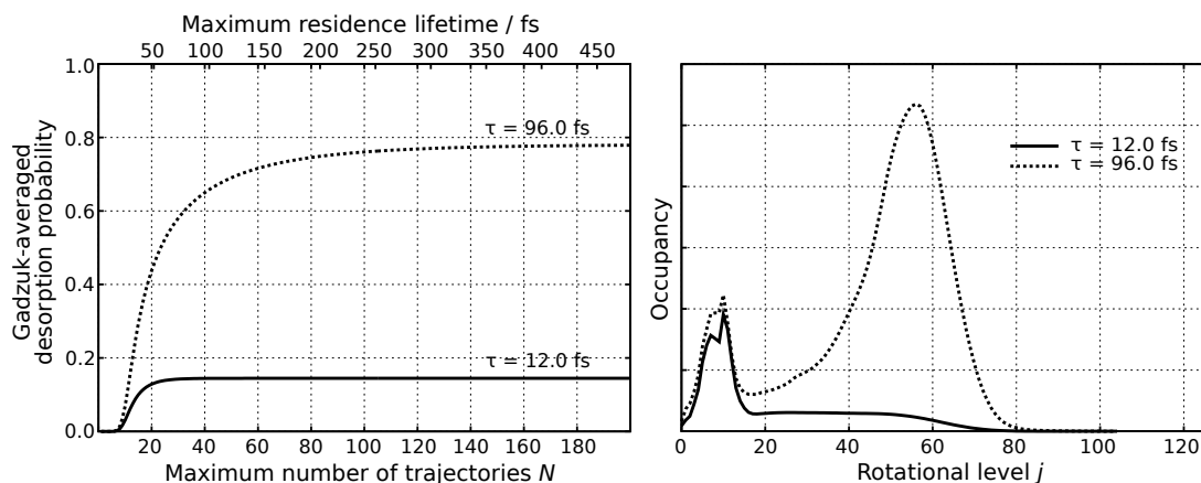
Fig. 3 Lifetime averaged desorption probability for specific resonance lifetimes \tau in dependence of the maximum residence lifetime on the excited state PES (left panel) and corresponding final asymptotic occupancy of the rotational levels (right panel).
