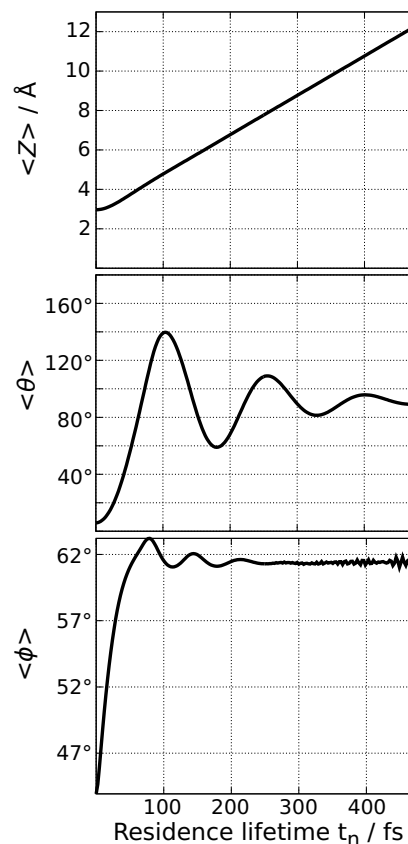
Fig. 4 Expectation values of the three examined geometrical degrees of freedom of the wave function during the propagation on the excited state PES.
