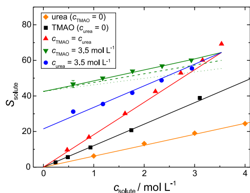
Fig. 6 Solute relaxation amplitude, S_{\text{solute}} (symbols). The solid lines show the value that would be expected if TMAO·3H 2 O ( \mu_{\text{eff,TMAO}\cdot 3\text{H}_2\text{O}} = 11.5\text{ D} ) complexes and urea ( \mu_{\text{eff,urea}} = 8.2\text{ D} ) molecules contribute independently to the solute relaxation mode. The dotted and dashed line correspond to what would be expected for the formation of long-lived TMAO:urea complexes for stoichiometric (1:1) association and for an association constant of K = 0.14\text{ L mol}^{-1} (see Ref. 12), respectively, assuming \mu_{\text{eff,TMAO:urea}} = 13.1\text{ D} (see text). The error bar represents the typical reproducibility \Delta S_{\text{solute}} = 2 .
