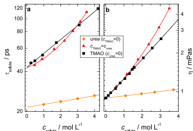
Fig. 7 (a) Solute relaxation time, \tau_{\text{solute}} , for solutions of urea, TMAO and equimolar TMAO+urea solutions obtained from fits of eq 2 to the dielectric spectra (symbols). (b) Dynamic viscosities, \eta , of the corresponding aqueous solutions (symbols). Viscosities for solutions of urea 44 and TMAO 45 were taken from the literature. Lines are guides to the eye.
