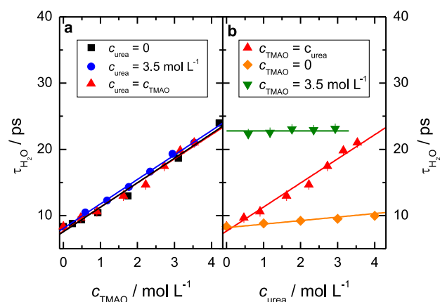
Fig. 5 Relaxation time of the water mode, \tau_{\text{water}} for samples with varying concentration of TMAO ( a ) and urea ( b ), respectively. Symbols correspond to values extracted from fits of eq 2 to the experimental spectra, lines show linear fits. Error bars correspond to the typical reproducibility \Delta\tau_{\text{H}_2\text{O}} = 0.3 \text{ ps} .
