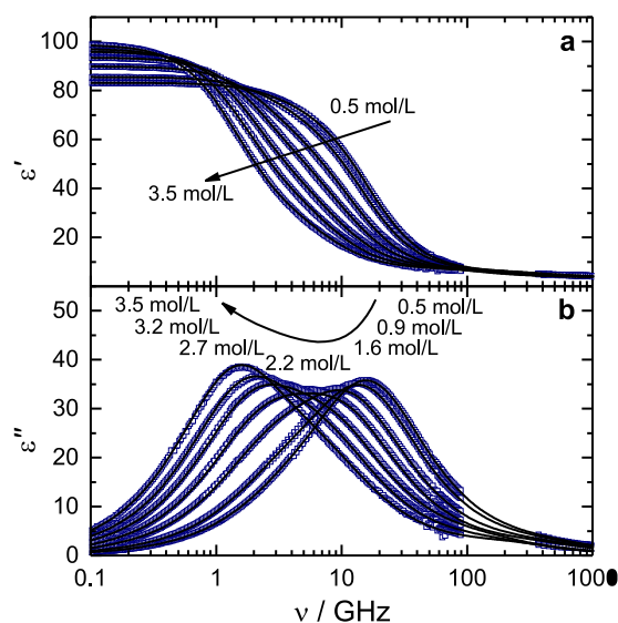
Fig. 3 Dielectric permittivity spectra, \epsilon'(v) (a), and dielectric loss spectra, \epsilon''(v) (b) for equimolar solutions of TMAO and urea in water. Symbols show experimental spectra, solid lines show the fits according to eq 2. The arrows indicate increasing concentration of TMAO and urea.
