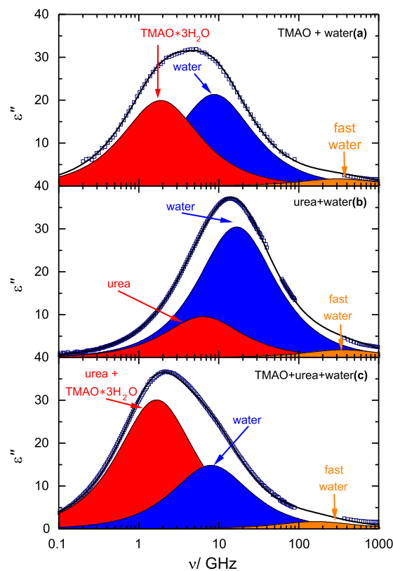
Fig. 2 Dielectric loss spectra for 3 \text{mol L}^{-1} solutions of TMAO in water (a), urea in water (b), and an equimolar solution of TMAO + urea in water (c). Symbols correspond to experimental data and the solid lines show the fits of eq 2 to the spectra. Shaded areas indicate the contributions of the solute (red), water (blue), and the fast water mode (orange) to the spectra. Data for TMAO in water are taken from Ref. 18.
