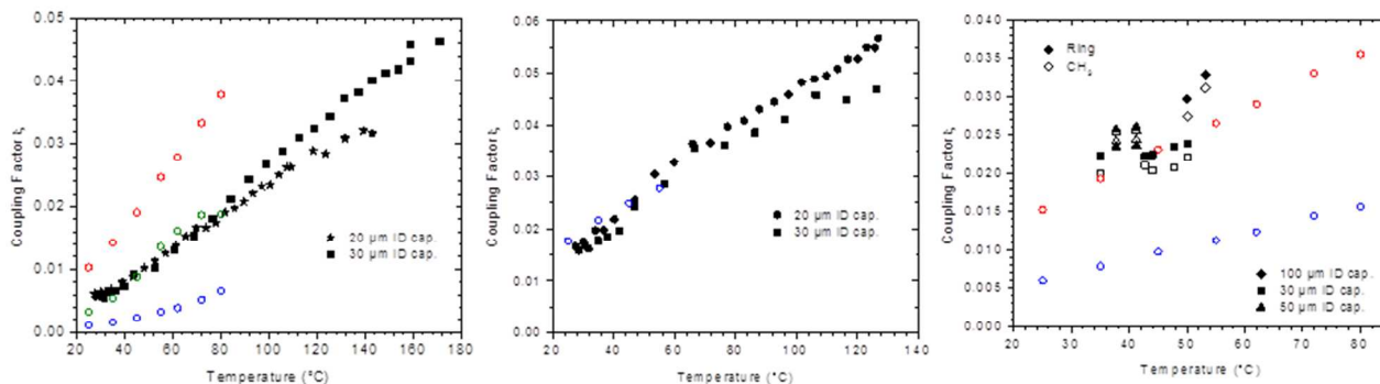
Figure 5 Comparison of coupling factors \xi calculated from DNP enhancement (in black) and from NMRD (outer-sphere model A in blue, outer-sphere and inner-sphere model B in red, model C as explained in the text in green) as a function of temperature. Left: DMSO, Middle: Acetone, Right: Toluene.
