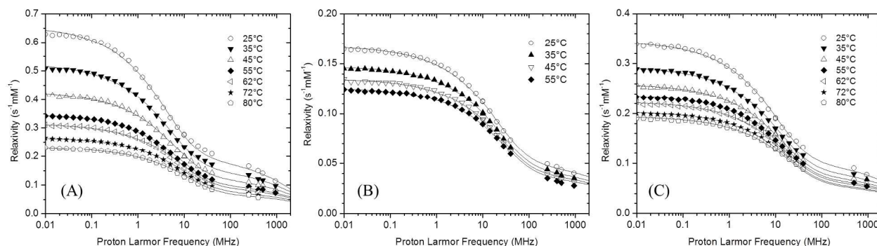
Figure 4 Solvents ^1\text{H} relaxivity profiles for solutions of ^{14}\text{N} -TEMPOL in DMSO (A), acetone (B) and toluene (C) are shown at different temperatures ranging from 25 to 80 ^{\circ}\text{C} . Best fit profiles from the outer-sphere model are also shown as lines.
