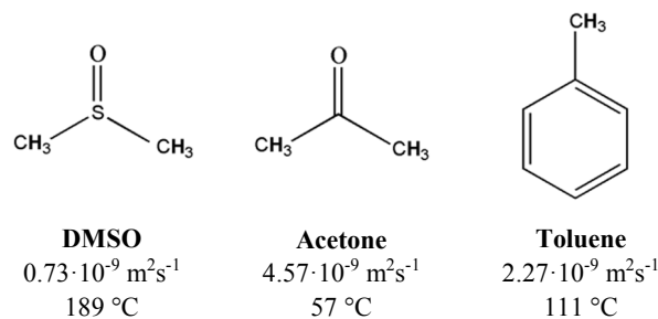
Scheme 1 Solvent molecules used in this study together with their diffusion coefficients at 25 °C and their boiling points in °C.
