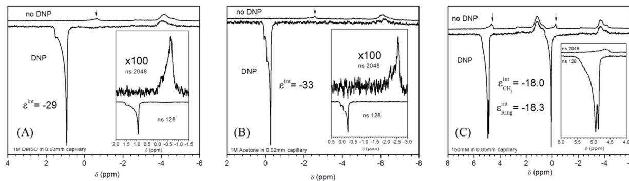
Figure 2 Normalized ^1\text{H} -NMR spectra to single scan of 1 M ^{14}\text{N} -TEMPOL in DMSO (A), acetone (B) and toluene (C) with (lower spectrum – 128 scans) and without (upper spectrum – 2048 scans) MW irradiation of the sample, respectively. Spectral intensities are normalized to number of scans, respectively. An integrated enhancement of -29, -33 and -18.3 can be observed on the corresponding proton signals. The inset shows the reference spectrum without irradiation enlarged by a factor of 100 for comparison, except toluene (C) where detail of the enhanced aromatic ring is shown. The peak at -4 ppm arises from solvent outside of the MW-resonator and is therefore not enhanced.
