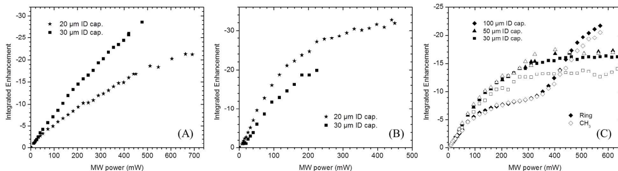
Figure 3 The DNP enhancement plotted against the incident MW power for a 1 M ^{14}\text{N} -TEMPOL in DMSO (A) and acetone (B), and 200 mM ^{14}\text{N} -TEMPOL in toluene (C) samples. Capillary sizes: 100 ( \blacklozenge ), 50 ( \blacktriangle ), 30 ( \blacksquare ) and 20 \mu\text{m} ( \star ).
