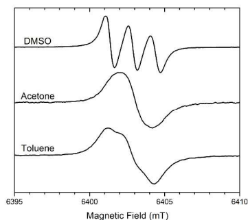
Figure 1 180 GHz CW-EPR spectra of 40 mM ^{14}\text{N} -TEMPOL in DMSO, acetone and toluene samples (not degassed) recorded at room temperature. The picture shows the varied line shape broadening for all three solvents, due to the different Heisenberg exchange rates.
