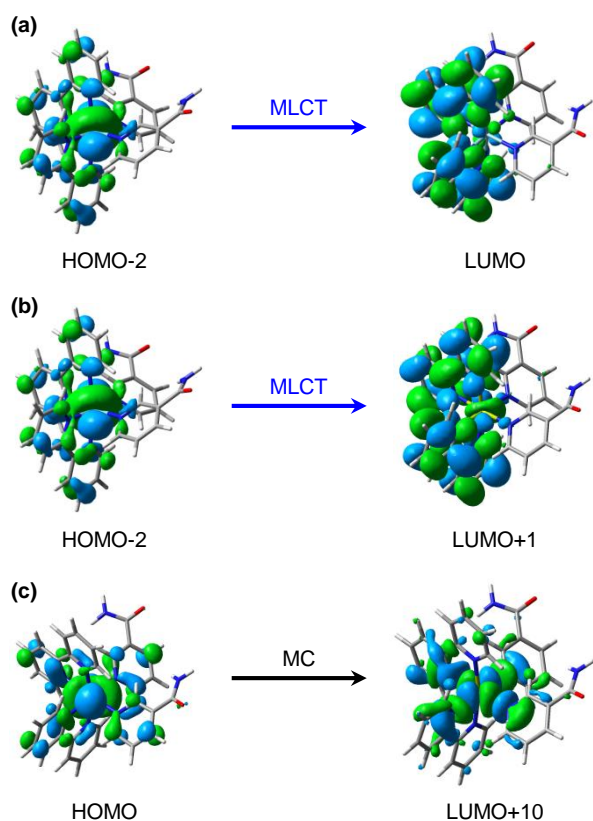
Figure 7. Calculated (major) orbital transitions associated with (a, b) the ^1\text{MLCT}/^3\text{MLCT} states and (c) ^1\text{MC}/^3\text{MC} states for complex 1 using the TD-B3LYP method – see Table 1.
