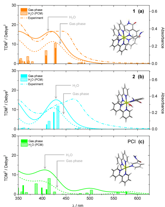
Figure 2. Calculated static UV/Vis absorption spectra for (a) 1 , (b) 2 and (c) PCI, both in the gas phase (dotted lines) and with a H 2 O PCM (solid lines). Calculated ground state structures shown inset. Spectra were calculated at the TD-B3LYP level of theory using a 28 electron SDD ECP for Ru and a cc-pVTZ basis set for C, O, N and H atoms. Calculated spectra were generated by convolution of the calculated squared transition dipole moments ( TDM^2 ) for singlet excitations with Gaussian functions (50 nm FWHM). Experimentally measured spectra for 1 and 2 from Figure 1 are shown in panels (a) and (b), respectively, for comparison (dashed lines).
