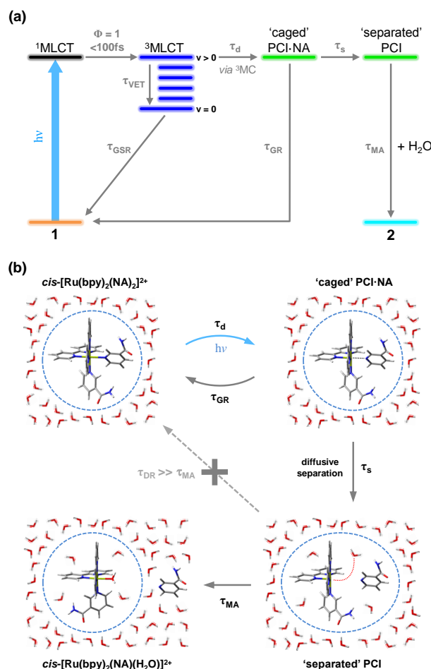
Figure 6. (a) Kinetic scheme illustrating the major pathways and associated time constants ( \tau ), used to model the photodissociation dynamics of 1 in \text{H}_2\text{O} . The individual steps involved in this kinetic scheme are discussed further in the main text (Section 3.3). (b) Pictorial schematic of the post-dissociation processes involving the PCI and formation of the photoproduct 2.
