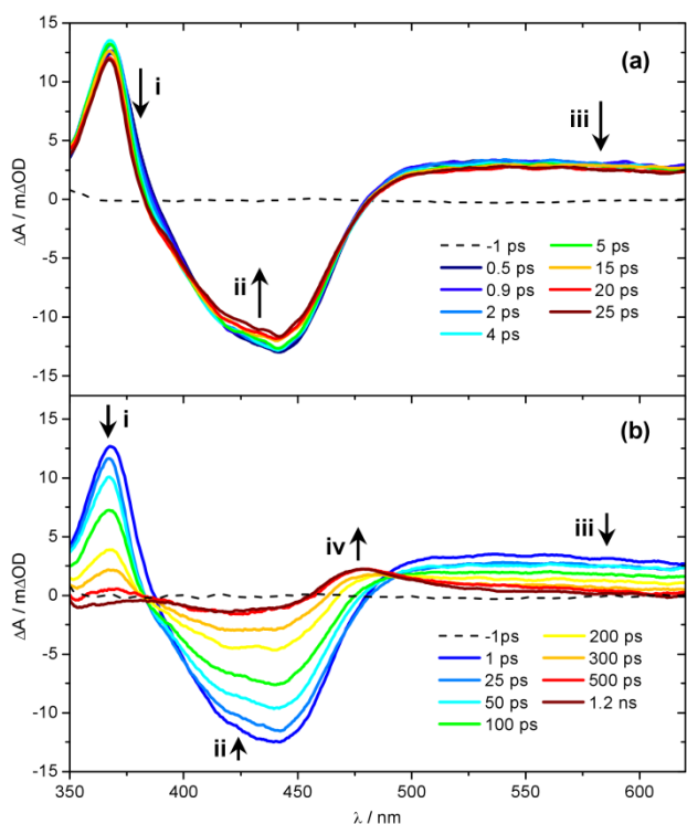
Figure 3. UV/Vis TAS of 890 \mu\text{M} aqueous solution of 1 over pump-probe delay ranges (a) t = -1 to 25 ps and (b) t = -1 ps to 1.2 ns, following photoexcitation at 340 nm. Growth/decay features i – iv highlighted indicate the spectral location assigned to the ^3\text{MLCT} ESA, GSB of 1 , absorption of the PCI and, finally, photoproduct 2 , respectively. See main text for further details.
