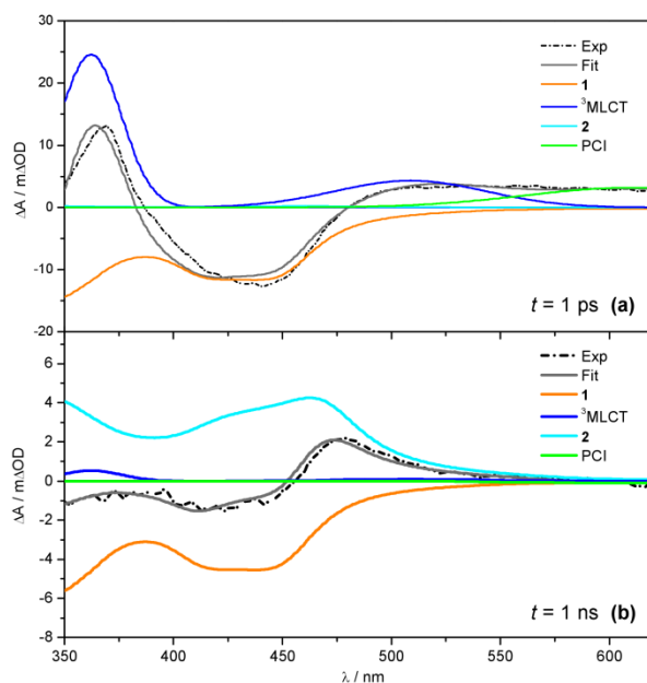
Figure 4. Representative fits (grey) to transient absorption spectra (black dashed) at (a) t = 1 ps and (b) t = 1 ns, showing the individual basis functions used in the ‘target analysis’ of the TAS in Figure 2. Basis functions have been assigned to the ^3\text{MLCT} ESA (blue), PCI complex (green), GSB recovery of 1 (orange) and formation of the photoproduct 2 (cyan). Static UV/Vis absorption spectra in Figure 1 are used as basis functions for 1 and 2 – see text for further details.
