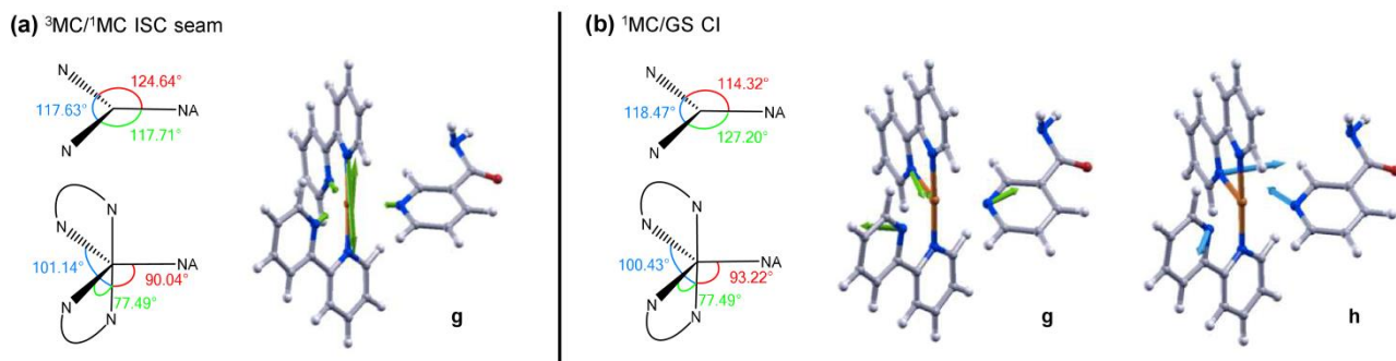
Figure 9. (a) MECP of the CASSCF calculated ^3\text{MC}/^1\text{MC} ISC seam. Equatorial and axial angles of this geometry as well as the gradient difference motion ( g ) are presented. (b) MECP of the CASSCF calculated ^1\text{MC}/\text{GS} CI, of quasi -JT type, and branching space. Equatorial and axial angles of this geometry as well as the gradient difference ( g ) and derivative coupling motions ( h ) are presented.
