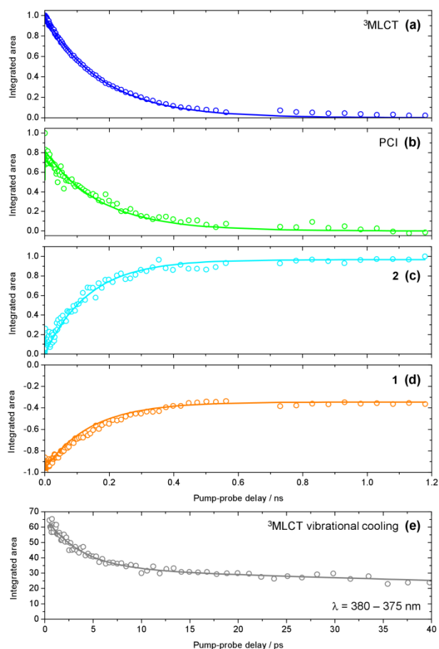
Figure 5. (a – d) Kinetic traces for the time-dependent evolution of the ^3\text{MLCT} state population (blue), PCI (green), photoproduct 2 (cyan) and GSB recovery of 1 (orange), obtained by integration of the basis functions (see Figure 4) used in the ‘target analysis’ of the TAS in Figure 3. Kinetic fits to these traces, in accordance with the scheme in Figure 6a, are shown by the solid lines – see main text for details. (e) Kinetic trace reflecting the vibrational cooling of the ^3\text{MLCT} state at t < 25 ps (grey squares), obtained by integration of the ‘red edge’ of the ^3\text{MLCT} feature i in Figure 3a over a range \lambda = 375 - 380 nm. The solid grey line represents a fit to the trace with a bi-exponential decay function.
