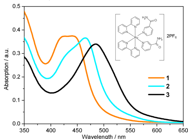
Figure 1. Static UV/Vis absorption spectra of [\text{Ru}(\text{bpy})_2(\text{NA})_2]^{2+} ( 1 , orange), [\text{Ru}(\text{bpy})_2(\text{NA})(\text{H}_2\text{O})]^{2+} ( 2 , cyan) and [\text{Ru}(\text{bpy})_2(\text{H}_2\text{O})_2]^{2+} ( 3 , black). Irradiation of 1 with 465 nm for 50 s yields 2 . Further irradiation of 2 for 1 h 50 min yields 3 . Molecular structure of 1 is shown inset.
