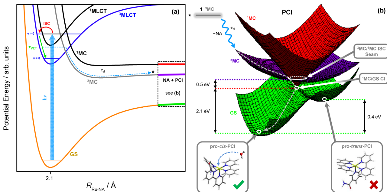
Figure 8. (a) Schematic potential energy profiles of the ^1\text{MLCT} , ^3\text{MLCT} , ^3\text{MC} , ^1\text{MC} and singlet ground state (GS) along the Ru–NA bond dissociation coordinate in 1 , including the major relaxation channels after excitation ( h\nu ) to the ‘bright’ ^1\text{MLCT} state. (b) Schematic potential energy surfaces for the significant electronic states in the PCI complex. From the top left, downwards: excited state population from the ^3\text{MC} of 1 (black) may land on the ^3\text{MC} PCI (purple) following NA ligand elimination; displacement through the ^3\text{MC}/^1\text{MC} ISC seam minimum (Figure 9a) to the ^1\text{MC} PCI (red); and then through the ^1\text{MC}/\text{GS} CI minimum (Figure 9b) leading to the GS of the PCI (green). On the GS, two possible isomers of PCI exist, labelled pro- cis and pro- trans (see SI, Table S6, for enlarged structures), into which a solvent molecule may be accommodated to complete the formation of 2 .
