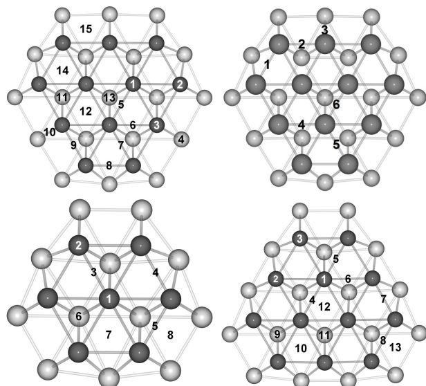
Fig. 1 Top view of the surface (dark grey) and subsurface (light grey) metal atoms at a (111) facet showing non-symmetry equivalent adsorption sites [Top Left] and bond numbering [Top Right] for TO Pt 116 . For reference, the numbering used for Pt 38 [Bottom Left] and Pt 79 [Bottom Right], is also shown.
