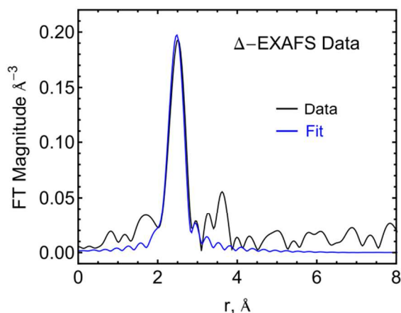
Fig. 4 Fourier transform magnitude of k^2 -weighted \chi(k) for the \Delta -EXAFS spectrum (black) and the fit of the data (blue) using the model in Eq. (4).
