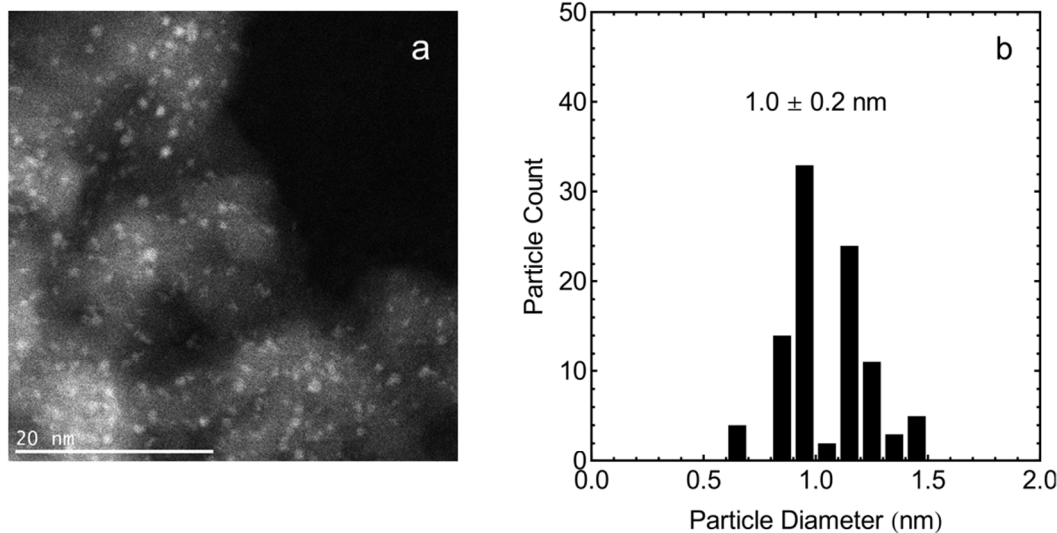
Fig. 2 (a) STEM image of Pd/SiO 2 nanoclusters and (b) particle size distribution of Pd/SiO 2 catalyst. The calculated number average particle diameter is 1.0 \pm 0.2 nm.
