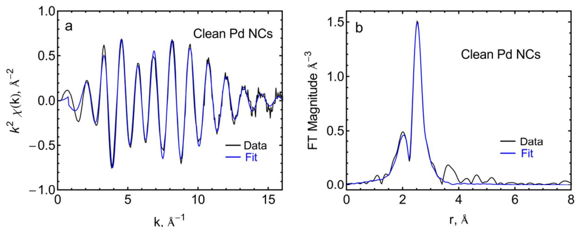
Fig. 1 (a) Edge-step normalized and background-subtracted k^2 -weighted \chi(k) EXAFS data and (b) Fourier transform magnitude of k^2 -weighted \chi(k) for the clean Pd NCs in He atmosphere at 77 K at the Pd K-edge. The first-shell fit of the data is shown in blue.
