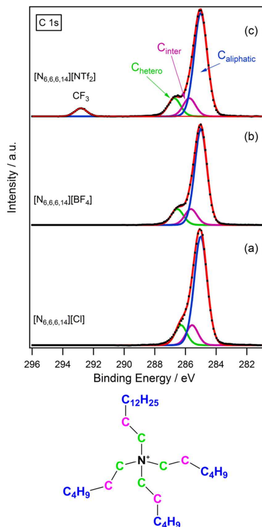
Fig. 2 High resolution XP spectra of the C 1s region with component fittings for (a) [\text{N}_{6,6,6,14}][\text{Cl}] , (b) [\text{N}_{6,6,6,14}][\text{BF}_4] and (c) [\text{N}_{6,6,6,14}][\text{NTf}_2] . Areas are normalised to the \text{N}_{\text{cation}} 1s photoemission peak for [\text{N}_{6,6,6,14}][\text{BF}_4] . All XP spectra charge corrected to \text{C}_{\text{aliphatic}} = 285.0 eV.
