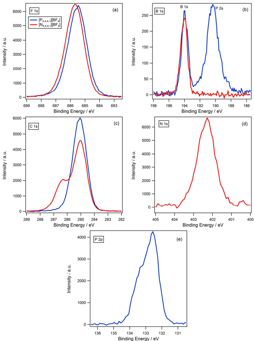
Fig. 7 XPS spectra of [\text{N}_{4,4,4,1}][\text{BF}_4] and [\text{P}_{4,4,4,1}][\text{BF}_4] for: (a) F 1s, (b) B 1s, (c) C 1s, (d) N 1s and (e) P 2p. Areas normalised to area of F 1s peak for [\text{N}_{4,4,4,1}][\text{BF}_4] . [\text{N}_{4,4,4,1}][\text{BF}_4] XPS spectra are charge corrected by setting N_{\text{cation}} 1s to 402.3 eV. [\text{P}_{4,4,4,1}][\text{BF}_4] XPS spectra are charge corrected by setting P_{\text{cation}} 2p_{3/2} to 132.6 eV.
