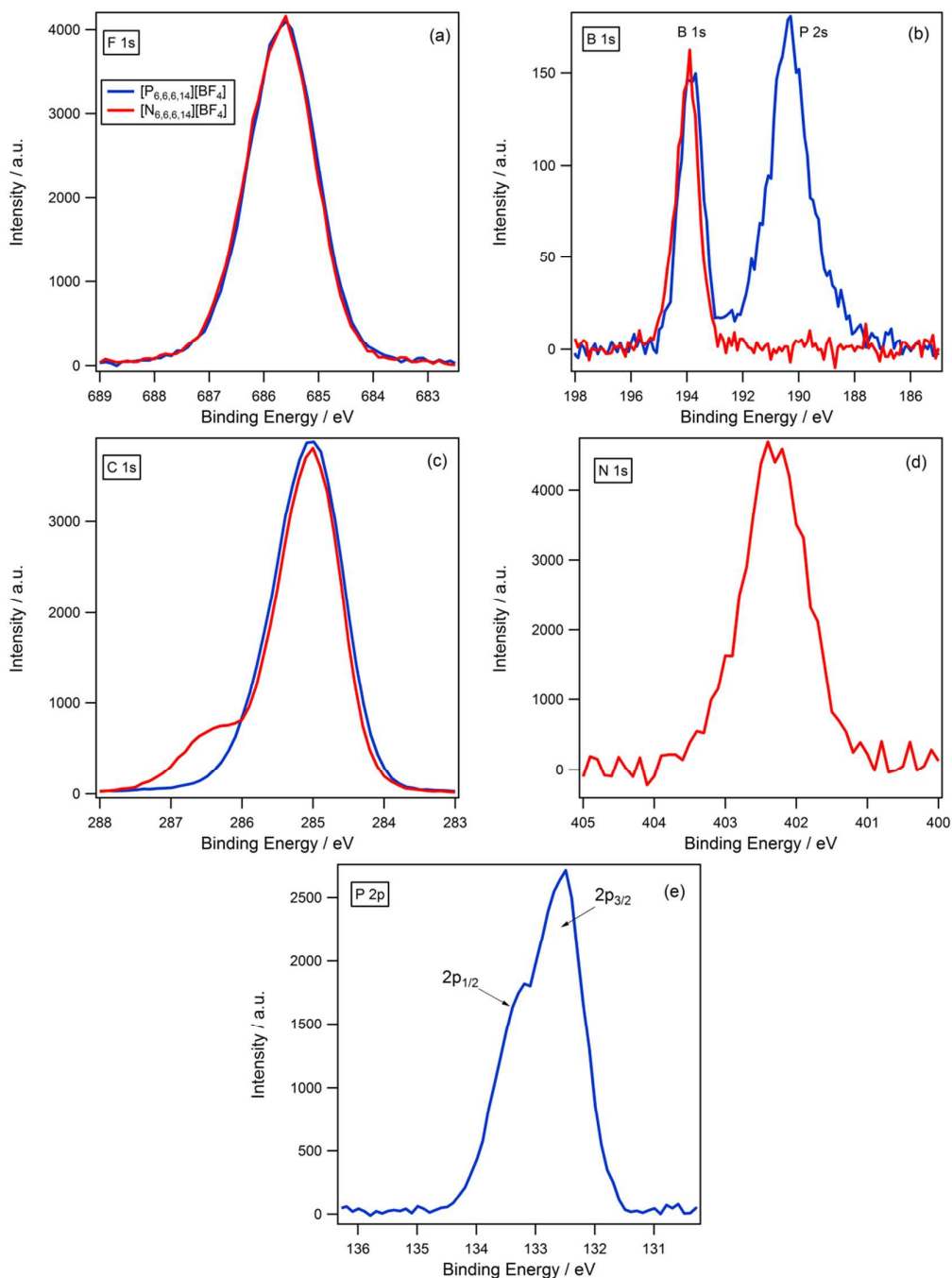
Fig. 6 XPS spectra of [\text{N}_{6,6,6,14}][\text{BF}_4] and [\text{P}_{6,6,6,14}][\text{BF}_4] for: (a) F 1s, (b) B 1s, (c) C 1s, (d) N 1s and (e) P 2p. Areas normalised to area of F 1s peak for [\text{N}_{6,6,6,14}][\text{BF}_4] . All XPS spectra were charge corrected by setting C_{\text{aliphatic}} 1s = 285.0 eV.
