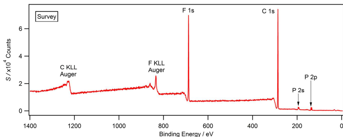
Fig. 1 Survey XPS spectrum for [P_{6,6,6,14}][PF_6] . The absence of photoelectron lines corresponding to other elements, especially oxygen and silicon, highlights the high purity of the compounds used in this study.
