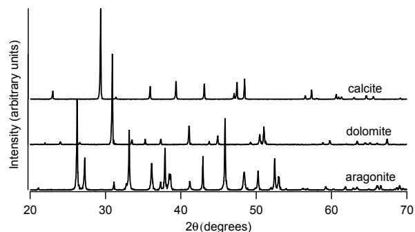
Fig. 1 Representative powder X-ray diffraction spectra at room temperature for spar calcite, geogenic dolomite, and spar aragonite. Lattice constant refinements of these data yield values in good agreement with JCPDS 14 standard patterns.
