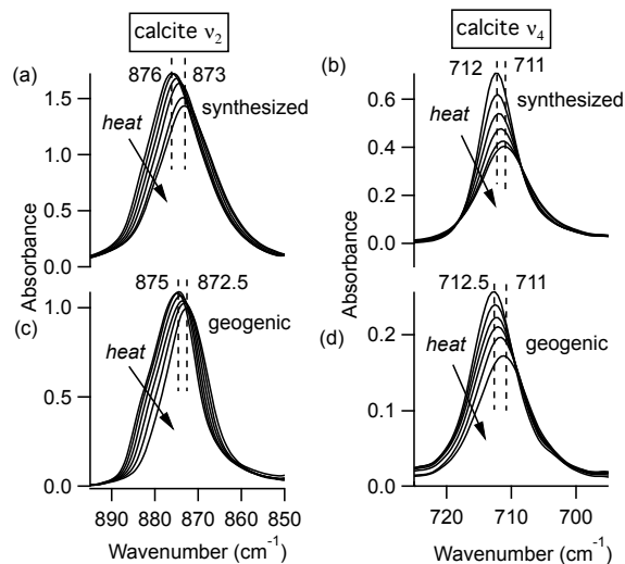
Fig. 3 FTIR spectra for lab-synthesized calcite (a,b) and geogenic spar calcite (c,d) at different temperatures. The arrows indicate that the v_2 and v_4 peaks shift to lower wavenumber values and have smaller amplitudes at higher temperatures.
