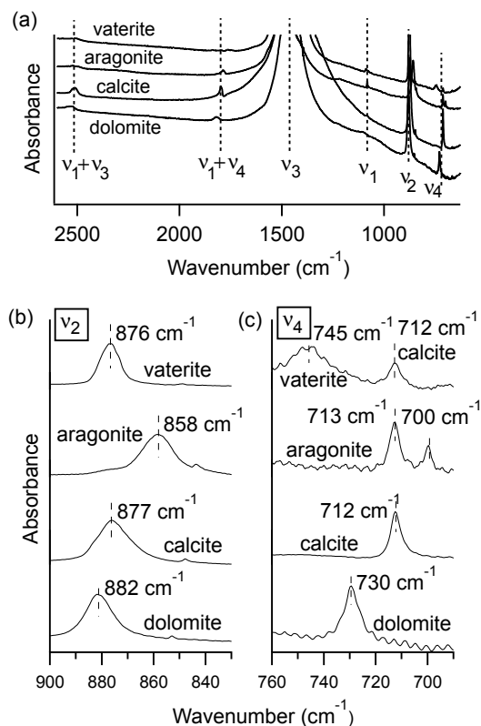
Fig. 2 Representative FTIR spectra at room temperature for lab-synthesized vaterite, spar calcite, spar aragonite and geogenic dolomite, showing (a) full spectra, (b) the v_2 modes, and (c) v_4 modes. Spectra are scaled and shifted along the vertical axis for clarity. High amounts of sample were used to boost the signal to noise for the v_2 and v_4 peaks, which leads to saturated absorbance unit values for the strongest ( v_3 ) peak; for this reason the full v_3 peak is not shown in (a).
