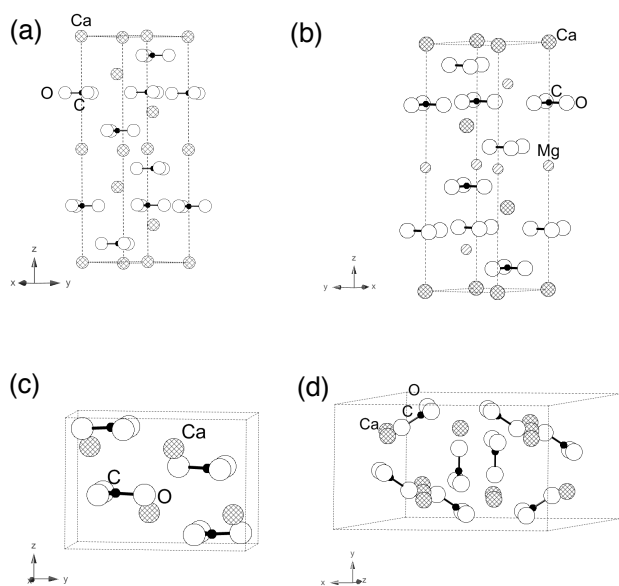
Fig. 6 Schematic representations of crystallographic unit cells for (a) calcite and (b) isostructural dolomite, as well as (c) aragonite and (d) vaterite.
