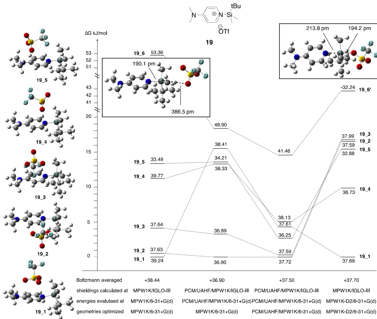
Figure 5. Relative free energies and chemical shifts of individual conformers of ion pair system 19 at different theory levels.
