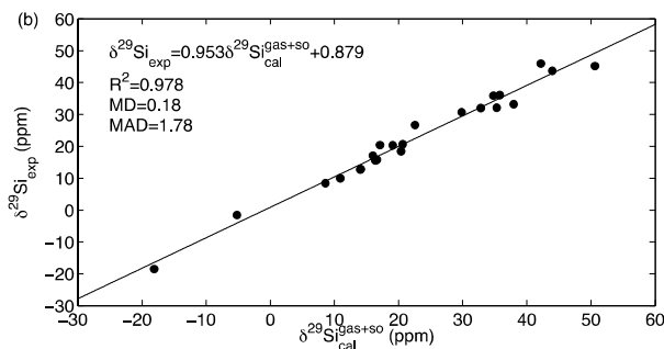
Figure 3. Comparison between experimentally measured and theoretically calculated shift values at MPW1K/IGLO-III//MPW1K/6-31+G(d) level for alkylchlorosilanes \text{SiMe}_{4-x}\text{Cl}_x with x = 1-4 . SO corrections are obtained from ZORA-SO-PBE0/TZ2P single-point calculations. Geometries are obtained at MPW1K/6-31+G(d) level in gas phase.
