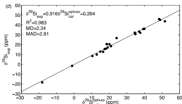
Figure 4. Theoretically calculated vs experimentally measured 29 Si chemical shifts for the data set collected in Table 5. (a) \delta(^{29}\text{Si}) calculated at MPW1K/IGLO-III//MPW1K/6-31+G(d) level. (b) \delta(^{29}\text{Si}) calculated at MPW1K/IGLO-III(+ZORA-SO)//MPW1K/6-31+G(d). (c) \delta(^{29}\text{Si}) calculated at PCM(UAHF)/MPW1K/IGLO-III(+ZORA-SO)//MPW1K/6-31+G(d) level using gas phase structures. (d) \delta(^{29}\text{Si}) calculated at PCM(UAHF)/MPW1K/IGLO-III(+ZORA-SO)//PCM(UAHF)MPW1K/6-31+G(d) level using solution phase structures.
