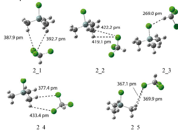
Figure 2. Structures of \text{SiMe}_3\text{Cl} ( 2 ) complexed to \text{CHCl}_3 obtained at MPW1K/6-31+G(d) level in the gas phase (dashed lines show shortest contacts between solvent and solute molecules).
