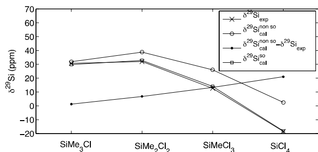
Figure 3. Comparison between experimentally measured and theoretically calculated shift values at MPW1K/IGLO-III//MPW1K/6-31+G(d) level for alkylchlorosilanes \text{SiMe}_{4-x}\text{Cl}_x with x = 1-4 . SO corrections are obtained from ZORA-SO-PBE0/TZ2P single-point calculations. Geometries are obtained at MPW1K/6-31+G(d) level in gas phase.
