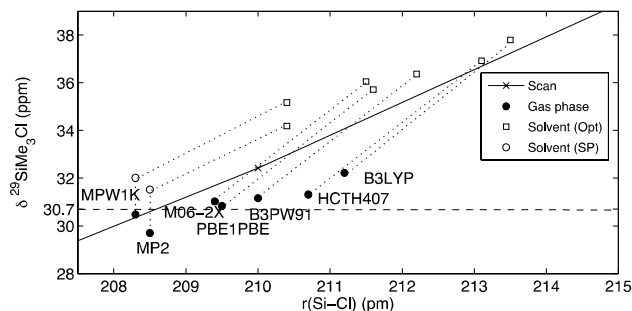
Figure 1. Calculated \delta(^{29}\text{Si}) values for \text{SiMe}_3\text{Cl} ( 2 ) (MP2: solid circles and PCM/MP2: empty symbols; IGLO-III basis set) using molecular structures optimized at various levels of theory using the 6-31+G(d) basis set. Dashed line: experimental value in \text{CDCl}_3 ; solid line: relaxed scan along the Si-Cl bond (gas phase, MPW1K structures). Empty circles: PCM/MP2 shifts on gas phase structures; empty squares: PCM/MP2 shifts on solution-phase geometries (all solvent calculations: \text{CHCl}_3 , UAHF radii).
