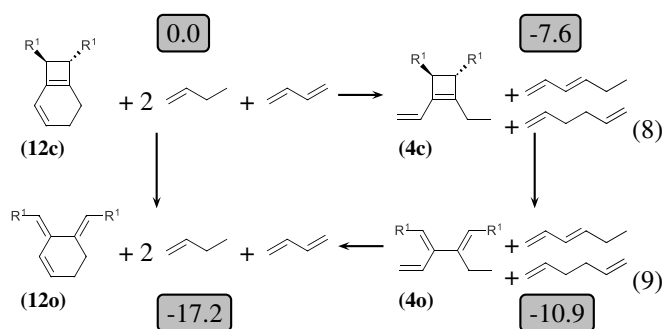
Fig. 4 Thermodynamic cycle which decomposes the opening of ( 12c ) into three steps. Relative energies in kcal/mol are indicated in gray boxes for R^1=OTMS . Reactions (8) and (9) are homodesmotic.
