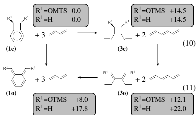
Fig. 5 Thermodynamic cycle which decomposes the opening of (1c) into three steps. Relative energies in kcal/mol are indicated in gray boxes for R^1=OTMS and R^1=H . Reactions (10) and (11) are homodesmotic.
