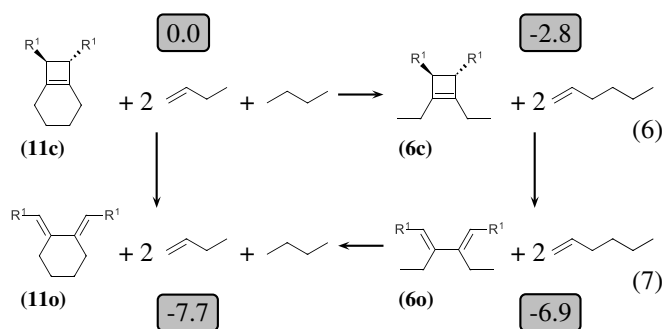
Fig. 3 Thermodynamic cycle which decomposes the opening of ( 11c ) into three steps. Relative energies in kcal/mol are indicated in gray boxes for R^1=OTMS . Reactions (6) and (7) are homodesmotic.
