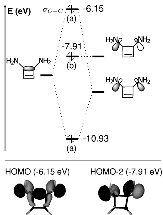
Fig. 8 Schematic representation of the interaction between lone pairs and the \sigma_{C-C} orbital, in the disubstituted cyclobutene R^1=NH_2 . Symmetry labels are given in parentheses in the C_2 point group of symmetry. The HOMO and HOMO-2 orbitals are represented below the orbital interaction diagram. The HOMO (-6.15 eV), is the \sigma_{C-C} bond, the HOMO-2 (-7.91 eV) is localized on the N atoms and the lowest energetic orbital is delocalized on the cycle. Energies are in eV (PBE0/def2-TZVP level). The energy of the not represented \pi orbital (the HOMO-1) is of -7.45 eV. Energies before interaction are arbitrary.
