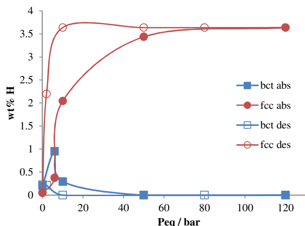
Fig. 5 Atomic hydrogen wt% in the sample contributed by the bct and fcc phases on absorption and desorption at variable hydrogen pressures (i.e. takes into account the occupancy per metal atom, and the phase fraction in the sample). The lines are shown as a guide to the eye.
