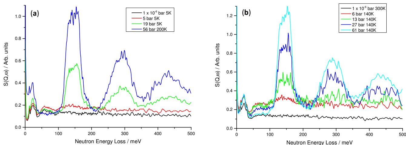
Fig. 9 INS spectra for (a) V_{20} 1 cycle at 5 – 200 K – the rise at low energy transfers for the 56 bar hydrogen P_{\text{eq}} is due to the higher collection temperature; (b) V_{20} 10 cycles at 140 – 300 K – the 1 \times 10^{-6} bar hydrogen P_{\text{eq}} dataset shows less intensity owing to the higher collection temperature (see Figure S2, ESI).
