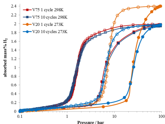
Fig. 1 Hydrogen pressure-composition isotherm for \text{Ti}_{25}\text{Cr}_{50}\text{V}_{20}\text{Mo}_5 ( \text{V}_{20} ) at 273K and \text{Ti}_{10}\text{Cr}_{10}\text{V}_{75}\text{Mo}_5 ( \text{V}_{75} ) at 298K for 1 cycle and 10 cycle samples during hydrogen absorption (filled data points) and desorption (empty data points). At 298K and 273K the \text{V}_{75} and \text{V}_{20} samples respectively achieve their maximum \text{H}_2 absorption at approximately 100 bar P_{\text{eq}} . The higher dissociation pressure and reduced capacity on cycling can be observed for \text{V}_{20} .
