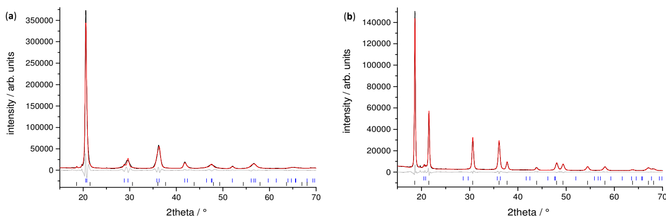
Fig. 2 XRD data and fit for \text{V}_{75} (a) 1 cycle sample at 1 \times 10^{-6} bar P_{\text{eq}} , and (b) 1 cycle sample at 100 bar hydrogen P_{\text{eq}} . At 1 \times 10^{-6} bar P_{\text{eq}} the sample predominantly consists of the bct phase, while at 100 bar the sample is mainly the fcc phase. Data are shown in black, the calculated pattern from the refined model in red, the difference in grey and tic marks for bct and fcc in blue and black respectively.
