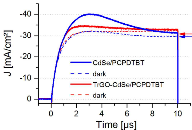
Figure 8. CELIV measurement results for a CdSe QD/polymer and a TrGO-CdSe QD/polymer solar cell, executed with a slope A of 400 \text{ mV}/\mu\text{s} under illumination and in dark. Respective capacitive current ( j(0) ) values calculated from capacitance-voltage measurements are indicated by arrows (red arrow for TrGO containing cell and blue arrow for a cell without TrGO).
