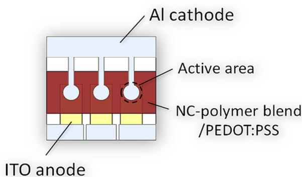
Figure 5. Top view of the design of the utilized hybrid BHJ device containing three individual solar cells (left, middle, right) on one substrate. The active layer consists either of a blend of CdSe NCs and PCPDTBT polymer or of a blend out of the CdSe NC-TrGO hybrid plus PCPDTBT.
