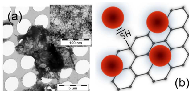
Figure 1. (a): TEM image of a TrGO flake decorated with CdSe QDs. Upper right inset: zoom in on the same CdSe QD-TrGO hybrid revealing the individual QDs. (b): Schematic of the CdSe QD-TrGO hybrid material.
