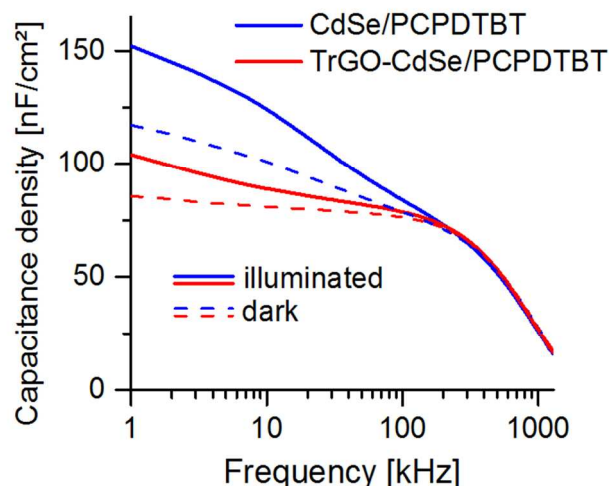
Figure 9. Capacitance density vs. frequency of CdSe/polymer and TrGO-CdSe/polymer solar cells from CdSe QDs under illumination and in dark.
