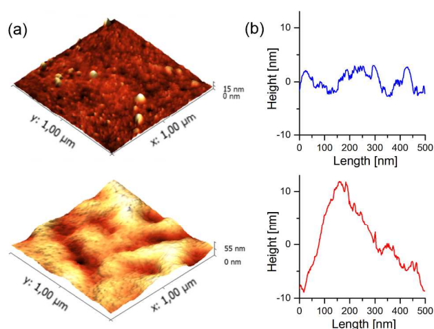
Figure 3. (a): AFM topographical images of the active layer surface of a CdSe/PCPDTBT (top) and of a TrGO-CdSe/PCPDTBT solar cell (bottom) recorded in tapping mode. (b): Representative extracted AFM height profiles of CdSe/PCPDTBT (top) and of TrGO-CdSe/PCPDTBT (bottom) films.
