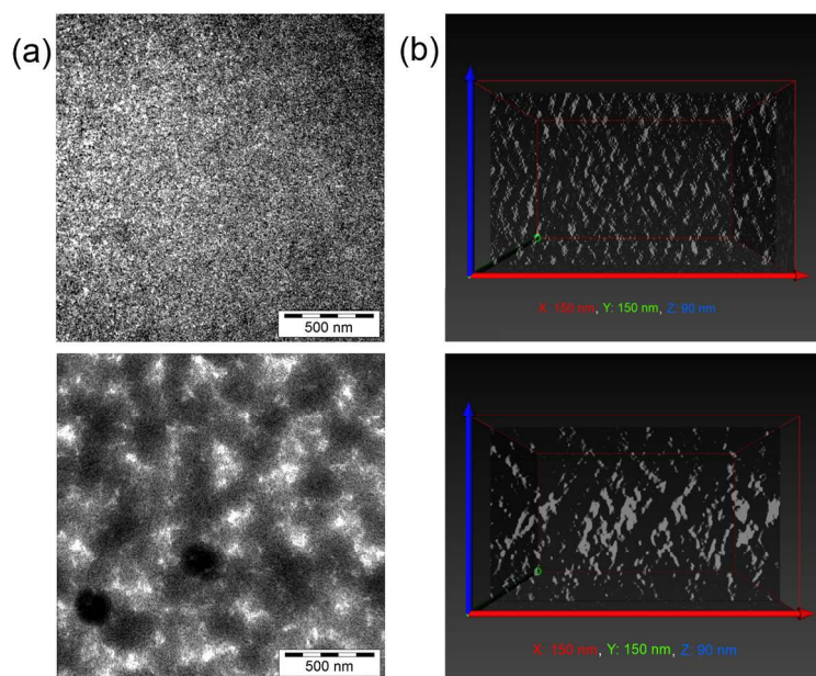
Figure 4. (a): TEM images of the active layer of a CdSe/PCPDTBT (upper image) and of a TrGO-CdSe/PCPDTBT solar cell (lower image). The dark regions represent CdSe QDs and the bright regions the polymer phase. (b): X-z-cut through 3D reconstructions of the respective active layers obtained by TEM tomography. The bright regions correspond to the volume filled with CdSe. The dimensions of the reconstructed volume were 150 nm parallel to the film (x- and y-direction) and 90 nm perpendicular to the film (z-direction).
