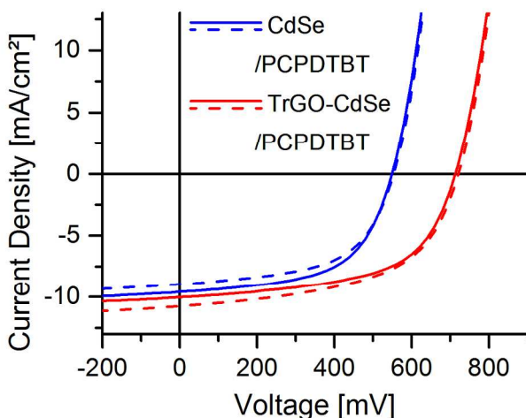
Figure 6. Current-density/voltage diagram for the best CdSe QD/PCPDTBT and TrGO-CdSe QD/PCPDTBT solar cell measured under AM 1.5G illumination in our laboratory (solid lines), and for comparison in the external laboratory 20 days later at the group of dye and organic solar cells of the Fraunhofer Institute for Solar Energy Systems (ISE) (dashed lines).
