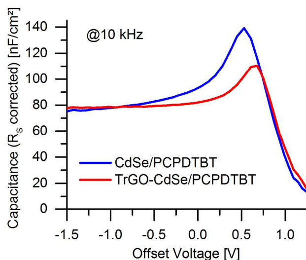
Figure 10. Capacitance vs. DC offset voltage at a modulation frequency of 10 kHz for the CdSe QD/PCPDTBT, and for the TrGO-CdSe QD/PCPDTBT solar cell respectively.
