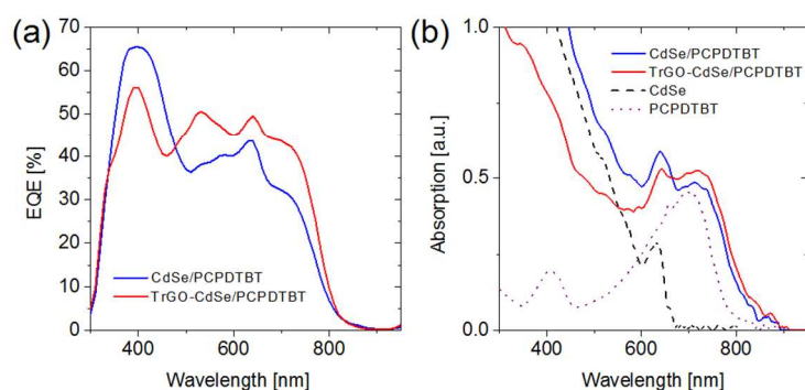
Figure 7. (a): External quantum efficiency (EQE) spectra from which spectral mismatch factors of 0.956 for the TrGO solar cell and 1.017 for our standard solar cell were determined. (b): Absorption spectra of the active layers out of CdSe QD/PCPDTBT with a 88:12 weight ratio, TrGO-CdSe QD/PCPDTBT with a 85:15 weight ratio of CdSe:PCPDTBT, and of solutions in chloroform from CdSe QDs and PCPDTBT.
