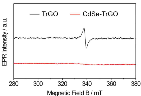
Figure 2. X-band electron paramagnetic resonance (EPR) spectra of illuminated TrGO (black graph) and the CdSe-TrGO hybrid (red graph) recorded at 9.86 GHz at room temperature.
