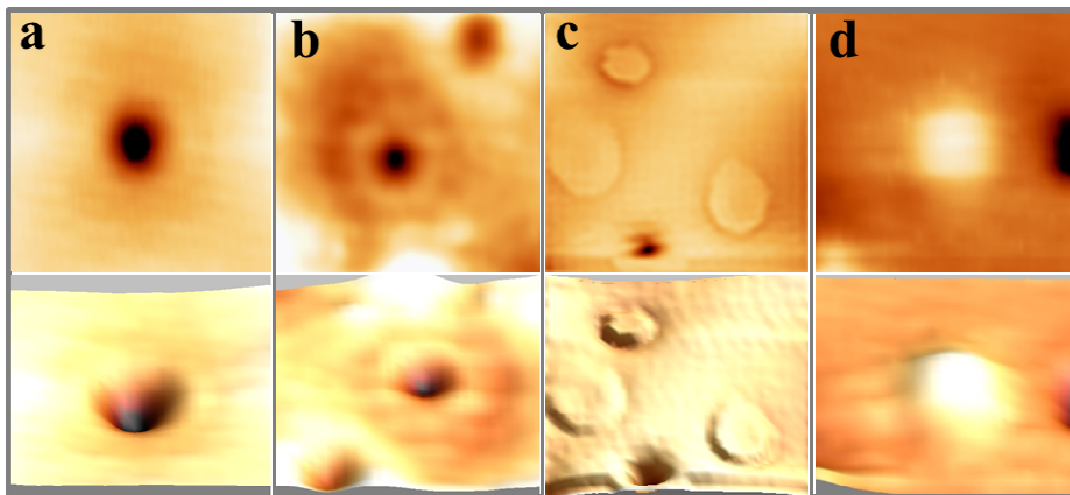
Fig.2. Close-up images of the four typical defects on the surface of \text{CaO}_{\text{Mo}} films (a, b and d: 50 \times 50 \text{ \AA}^2 , c: 100 \times 100 \text{ \AA}^2 ). (a) Minimum of 0.8 Å depth (A-defect). (b) Shallow depression surrounded by concentric rings (B-defect). (c) Ring features with up to 50 Å diameters (C-defect) and (d) shallow protrusions of 0.15 Å height (D-defect). Top and bottom images are 2D and pseudo 3D representations of the same defect type.
