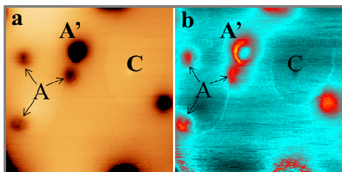
Fig. 3: (a) STM topographic and (b) corresponding dI/dV image of a 30 ML thick CaO film. Note the spatial proximity between the A and C defects. The latter is best seen in the conductance image gives its small apparent height ( 200 \times 200 \text{ \AA}^2 ).
