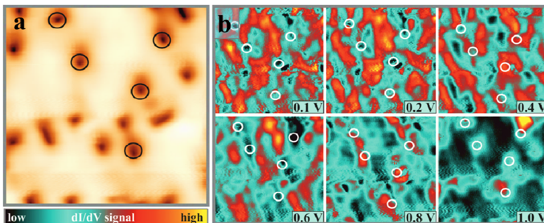
Fig.5. (a) STM topographic image and (b) corresponding dI/dV maps taken on 15 ML thick \text{CaO}_{\text{Mo}} films at the indicated bias voltages ( 200 \times 200 \text{ \AA}^2 ). The inhomogeneity of the electronic structure reflects the uneven spatial distribution of Mo ions inside the oxide lattice.
