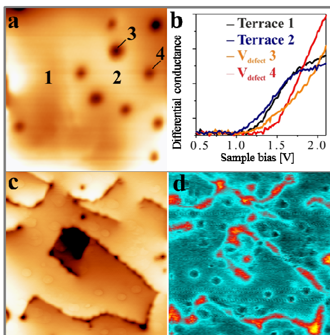
Fig.6: (a) STM topographic image of a 15 ML CaO_{Mo} film ( 200 \times 200 \text{ \AA}^2 ) and (b) dI/dV spectra taken at the indicated surface positions. The set-point bias was set to 2.0 V in all four cases. (c,d) Topographic image and corresponding dI/dV map taken at 3.5 V on a 30 ML thick CaO_{Mo} film ( 450 \times 450 \text{ \AA}^2 ). The most prominent defects in the image are the Mo dopants (C-defects) and the dislocation lines.
