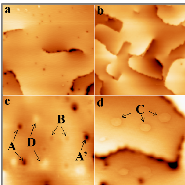
Fig. 1: STM topographic images of two 30 \text{ ML} thick \text{CaO} films annealed to (a) 1200 \text{ K} and (b) 1000 \text{ K} ( 500 \times 500 \text{ \AA}^2 ). Note the different defect concentrations. (c,d) High resolution images showing the four different defect types discussed in the text ( 200 \times 200 \text{ \AA}^2 ).
