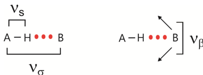
Scheme I: Stretching ( \nu_{\sigma} ) and bending ( \nu_{\beta} ) vibrational modes of two hydrogen bonded molecules along the bond A-H...B.
