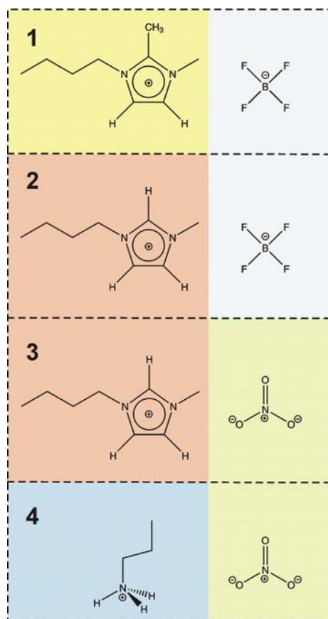
Fig. 13 The imidazolium-based aprotic ionic liquids [C 4 C 1 mim][BF 4 ] ( 1 ), [C 4 mim][BF 4 ] ( 2 ), [C 4 mim][NO 3 ] ( 3 ) and the protic ionic liquid [PrAm][NO 3 ] ( 4 ). Similar colors indicate like cations and anions, respectively. Reprinted from ref 76 with permission. Copyright 2009 The Royal Society of Chemistry.
