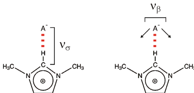
Scheme II: The stretching ( \nu_{\sigma} ) and bending ( \nu_{\beta} ) modes of the cation-anion interaction for the {}^+\text{C}(2)\text{-H}\cdots\text{A}^- interaction within 1,3-dimethyl-imidazolium cation.
