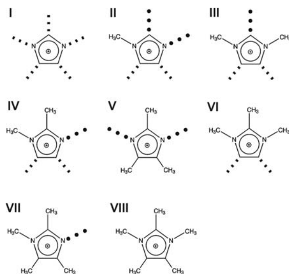
Fig. 30 Structures of imidazolium-based cations of imidazolium ( I ), 1-methyl-imidazolium ( II ), 1,3-dimethyl-imidazolium ( III ), 1,2-dimethyl-imidazolium ( IV ), 2,4,5-trimethyl-imidazolium ( V ), 1,2,3-trimethyl-imidazolium ( VI ), 1,2,4,5-tetramethyl-imidazolium ( VII ), and 1,2,3,4,5-pentamethyl-imidazolium ( VIII ). The different positions of H-bond abilities are indicated by bold dots and the remaining interaction sites as dotted lines. Reprinted from ref 144 with permission. Copyright 2011 Wiley VCH.
