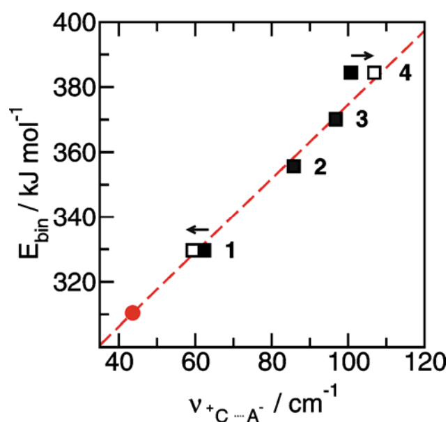
Fig. 7 Average binding energies E_{\text{bin}} per ion pair in tetramers of the ionic liquids 1-4 plotted versus the measured H-bond frequencies \tilde{\nu}_{+C...A^-} . Using the obtained linear relationship we can predict the H-bond frequency for ionic liquid ([1,2,3,4,5-pentamethyl-im][NTf 2 ]) (filled circle). The filled symbols represent the measured frequencies and the open symbols give the
