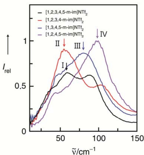
Fig. 9 Far infrared spectra of imidazolium-based ionic liquids I-IV . The maxima in the spectra indicate the anion-cation interaction as supported by the subsequent experimental and theoretical analysis. Reprinted from ref 119 with permission. Copyright 2011 The Royal Society of Chemistry.
