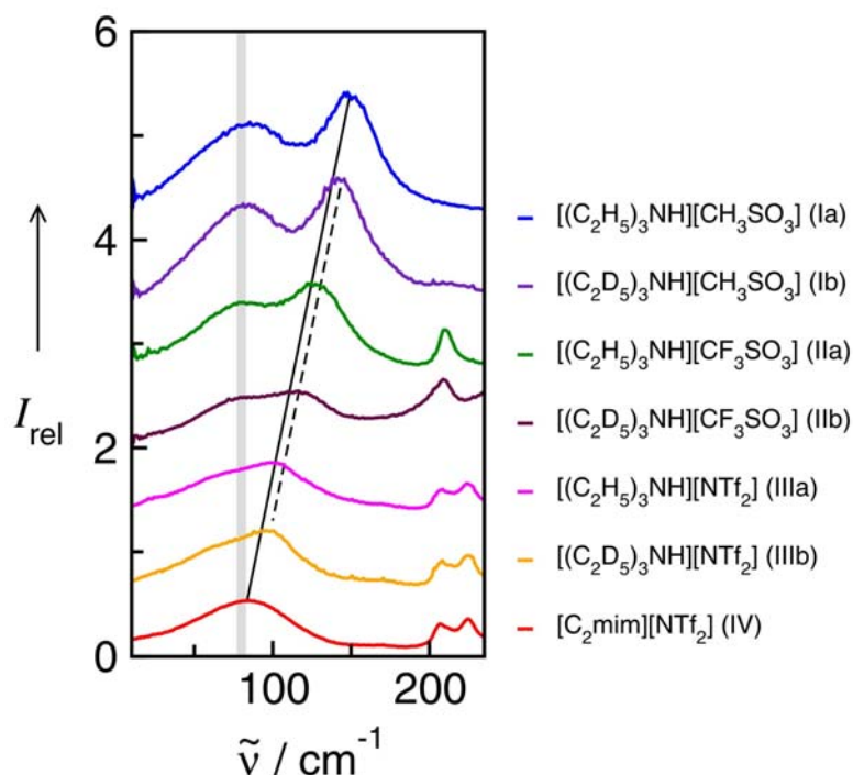
Fig. 18 Far infrared spectra of [(\text{C}_2\text{H}_5)_3\text{NH}][\text{CH}_3\text{SO}_3] ( Ia ), [(\text{C}_2\text{H}_5)_3\text{NH}][\text{CF}_3\text{SO}_3] ( IIa ), [(\text{C}_2\text{H}_5)_3\text{NH}][\text{NTf}_2] ( IIIa ), and [(\text{C}_2\text{mim})][\text{NTf}_2] ( IV ) and the corresponding protic ionic liquids for the fully deuterated ethyl groups of the ammonium cation ( Ib-IIIb ). The vibrational band at 149\text{ cm}^{-1} for Ia can be assigned to the ^+\text{N-H}\cdots\text{CH}_3\text{SO}_3^- intermolecular interaction. This interaction strength is decreasing with the series of Ia-IIIa as indicated by the straight line. For the deuterated PILs the reduced mass effect is shown by the dotted line. Reprinted from ref 135 with permission. Copyright 2013 Wiley VCH.
