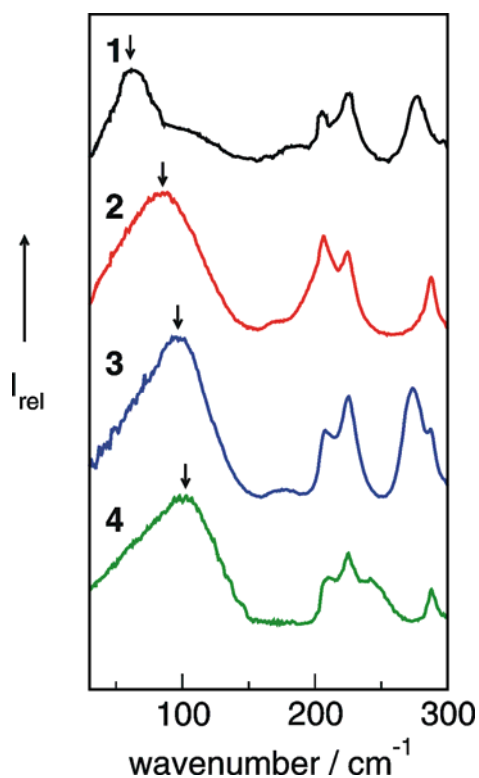
Fig. 6 Far infrared spectra of [1,2,3-trimethyl-im][NTf 2 ] ( 1 ), [1,3-dimethyl-im][NTf 2 ] ( 2 ), [1,2-dimethyl-im][NTf 2 ] ( 3 ), [1-methyl-im][NTf 2 ] ( 4 ) at 323 K for 2-4 and 383 K for 1 . Reprinted from ref 52 with permission. Copyright 2010 Wiley VCH.
