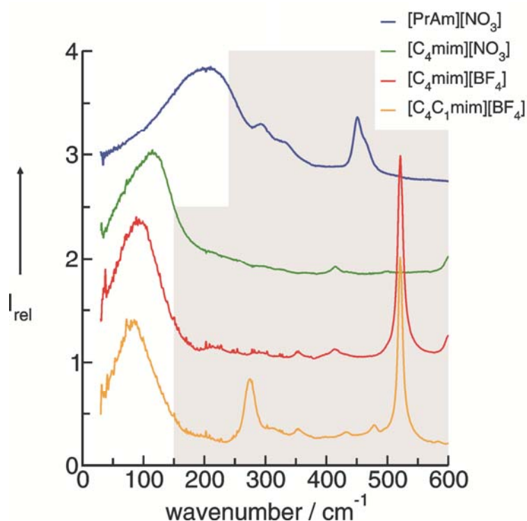
Fig. 14 FIR spectra of [\text{C}_4\text{C}_1\text{mim}][\text{BF}_4] , [\text{C}_4\text{mim}][\text{BF}_4] , [\text{C}_4\text{mim}][\text{NO}_3] and [\text{PrAm}][\text{NO}_3] at 353 K. Reprinted from ref 76 with permission. Copyright 2009 The Royal Society of Chemistry.
