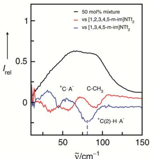
Fig. 10 Far infrared spectra for a 50 mol% mixture of the ILs I and III (black line) along with the difference spectra obtained from measurements of this mixture versus the background spectrum of IL I (red line) and IL III (blue line), respectively. The negative contribution at about 77\text{ cm}^{-1} can be assigned to the {}^+\text{C}(2)\text{-H}\cdots\text{A}^- interaction in IL III and is indicated by the dotted line. Reprinted from ref 120 with permission. Copyright 2011 The Royal Society of Chemistry.
