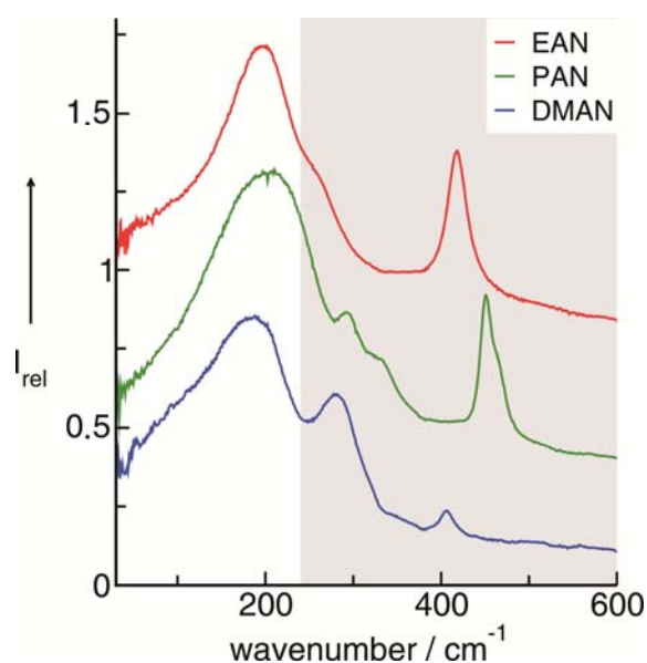
Fig. 24 FIR spectra of ethylammonium nitrate (EAN), propylammonium nitrate (PAN), and dimethylammonium nitrate (DMAN) measured at 353 K. Reprinted from ref 51 with permission. Copyright 2009 Wiley VCH.
