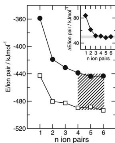
Fig. 17 DFT calculated cluster energies per ion-pair for [(\text{CH}_3)_4\text{N}][\text{NO}_3]_n (filled circles) and [(\text{CH}_3)_3\text{NH}][\text{NO}_3]_n (open squares) with n=1-6 . The energy difference between clusters of similar size of these protic ionic liquids are shown in the inlay and represent the H-bond strength of the ^+\text{N-H} \cdots \text{NO}_3^- interaction in [(\text{CH}_3)_3\text{NH}][\text{NO}_3] . The H-bond energy is quantified to be 49.4 \text{ kJmol}^{-1} . The slightly higher dispersion energies in clusters [(\text{CH}_3)_4\text{N}][\text{NO}_3]_n due to
