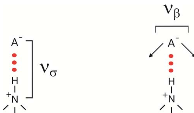
Scheme III: The stretching ( \nu_s ) and bending ( \nu_\beta ) frequencies of the cation-anion interaction for the {}^+\text{N}-\text{H}\cdots\text{A}^- interaction including a trimethyl ammonium cation.
