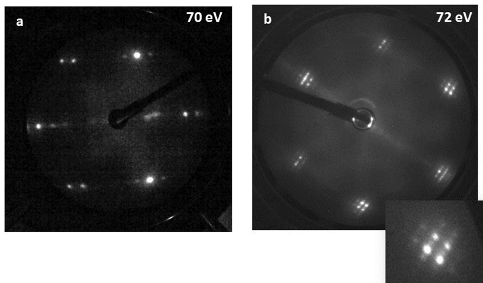
Figure 2. LEED patterns for clean Au(332) (a) and Au(887) (b). Inset: magnification of the region within the grey circle in b showing the spot splitting on Au(887).
