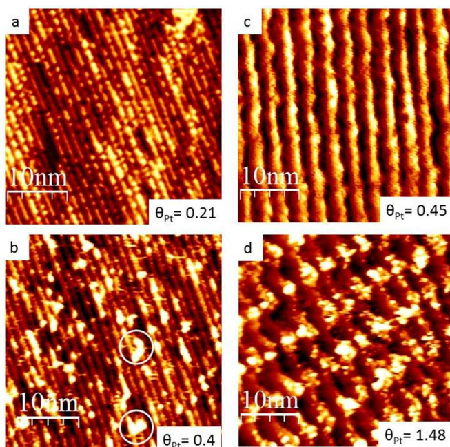
Fig 6. STM images of samples annealed at 473 K. (a,b) Pt/Au(332) and (c,d)Pt/Au(887). Tunneling conditions: a) V_{\text{bias}}=1.25\text{V} , I_t=0.35\text{ nA} ; b) V_{\text{bias}}=1.3\text{V} , I_t=0.41\text{ nA} ; c) V_{\text{bias}}=1.25\text{V} , I_t=0.35\text{ nA} and d) V_{\text{bias}}=1.1\text{V} ; I_t=0.17\text{ nA} .
