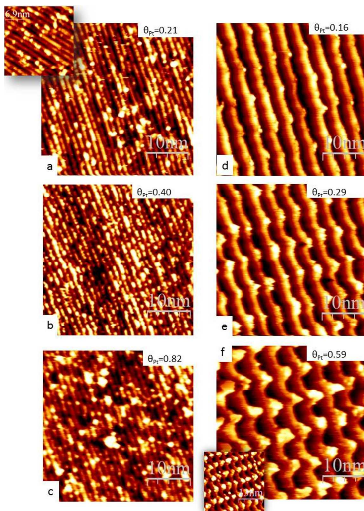
Fig 3. STM images of Pt deposits on Au vicinal surfaces. (a-c) Pt/Au(332) and (d-f)Pt/Au(887). Pt coverage is indicated on each image. Tunneling conditions: (a) V_{\text{bias}}=1.7\text{ V} ; I_t=0.55\text{ nA} ; (b) V_{\text{bias}}=1.25\text{ V} ; I_t=0.36\text{ nA} ; (c) V_{\text{bias}}=1.5\text{ V} ; I_t=0.56\text{ nA} ; (d) V_{\text{bias}}=1.24\text{ V} ; I_t=0.45\text{ nA} ; (e) V_{\text{bias}}=1.32\text{ V} ; I_t=0.32\text{ nA} and (f) V_{\text{bias}}=1.25\text{ V} ; I_t=0.36\text{ nA} . Insets in (a) and (f) correspond to Pt/Au(332) with \theta_{\text{Pt}}=0.18 and Pt/Au(887) with \theta_{\text{Pt}}=1.48 , respectively.
