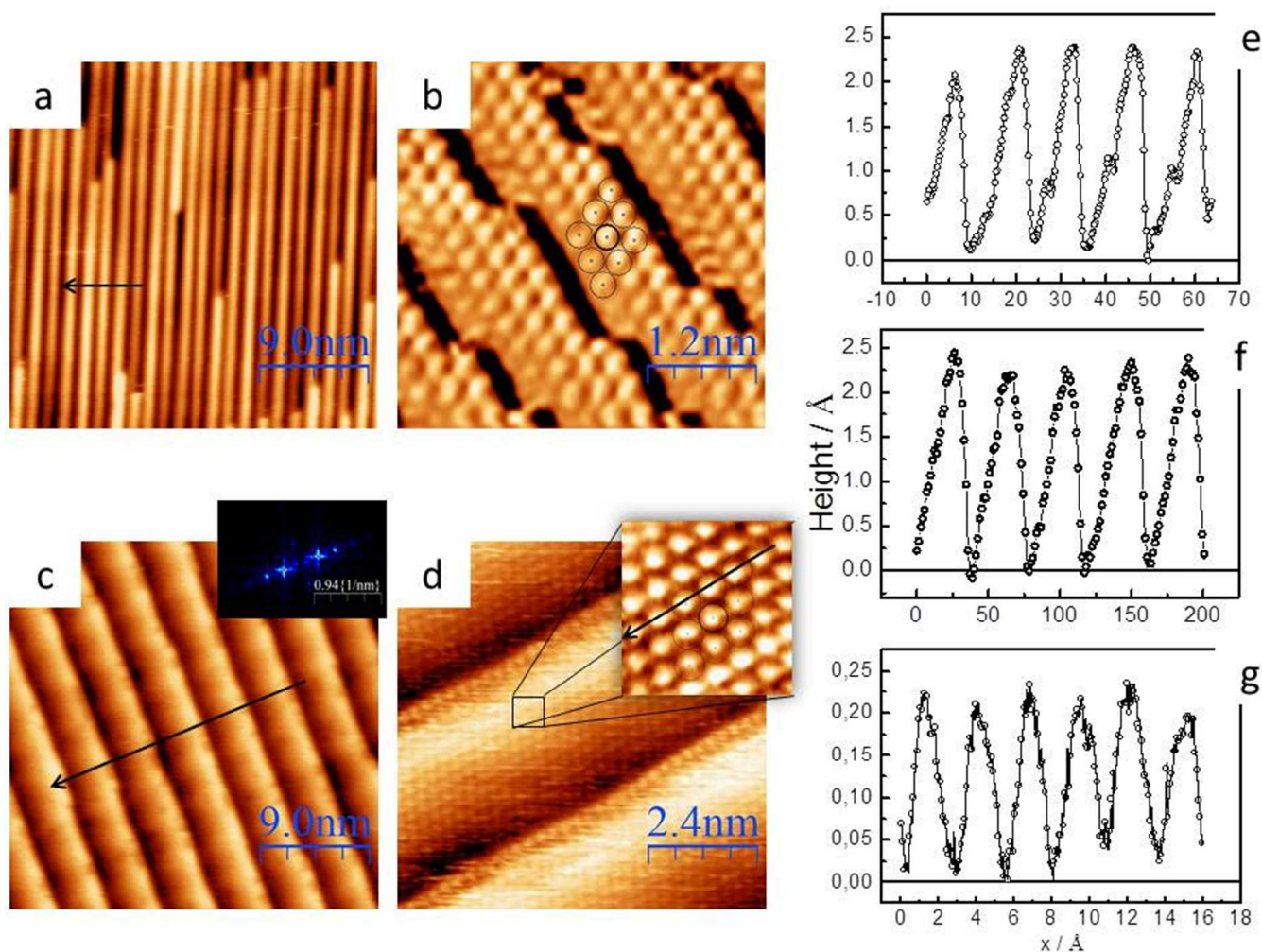
Fig 1. STM images obtained for clean Au(332) (a,b) and Au(887) (c,d). Inset in c corresponds to FFT 2D pattern of STM image. Topographic profiles showing periodic nature of terraces are displayed in (e) and (f) for Au(332) and Au(887), respectively. Atomic profile from inset in (d) is shown in (g). Tunneling conditions are: (a,b) I_{\text{tunnel}} = 0.11 and 0.30 nA, V_{\text{bias}} = 1.2 and 1.7 V; (c,d) I_{\text{tunnel}} = 0.160 and 1.730 nA, V_{\text{bias}} = 1.2 and 0.42 V.
