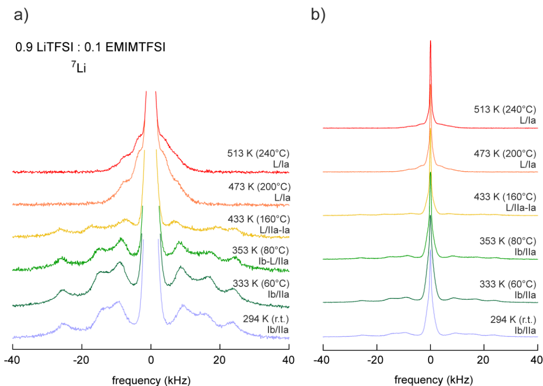
Fig. 3 Change of the solid-state {}^7\text{Li} NMR spectra (194.3 MHz) of \text{Li}_x\text{EMIM}_{(1-x)}\text{TFSI} with x = 0.9 with increasing temperature; a) lower part of the spectra magnifying the quadrupole powder pattern, b) full spectra revealing the two-component NMR central transition. The area fractions of the two NMR lines (see also the inset of Figure 2 b) are plotted in Figure 4 as a function of temperature.
