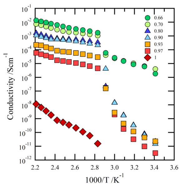
Fig. 5 Ion conductivities obtained for \text{Li}_x\text{EMIM}_{(1-x)}\text{TFSI} ( 0.66 \leq x \leq 1 ) system; data collected during heating.
