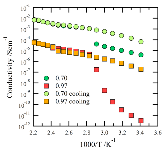
Fig. 7 Comparison of ion conductivities obtained for \text{Li}_x\text{EMIM}_{(1-x)}\text{TFSI} ( x = 0.70 and x = 0.97 ) system; data collected during heating and cooling.
