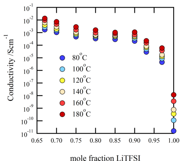
Fig. 6 Conductivity isotherms for \text{Li}_x\text{EMIM}_{(1-x)}\text{TFSI} ( 0.66 \leq x \leq 1 ) system as function of composition; data collected during heating.
