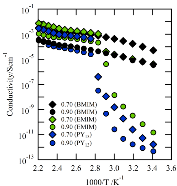
Fig. 8 Comparison of ion conductivities obtained for the \text{Li}_x\text{EMIM}_{(1-x)}\text{TFSI} , \text{Li}_x\text{BMIM}_{(1-x)}\text{TFSI} , and \text{Li}_x\text{PY}_{13(1-x)}\text{TFSI} ( x = 0.70 and x = 0.90 ) systems; data collected during heating.
