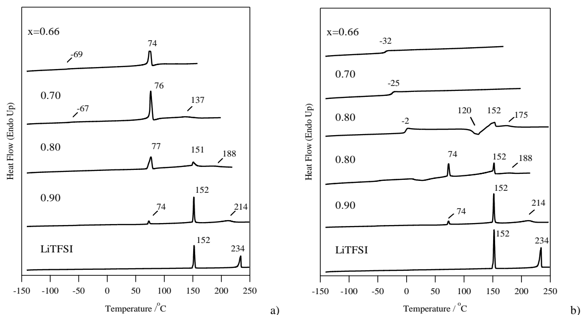
Fig. 1 DSC heating traces for the \text{Li}_x\text{EMIM}_{(1-x)}\text{TFSI} ( 0.66 \leq x \leq 1 ) system; data collected during first heating cycle a), data collected during second heating cycle b).
