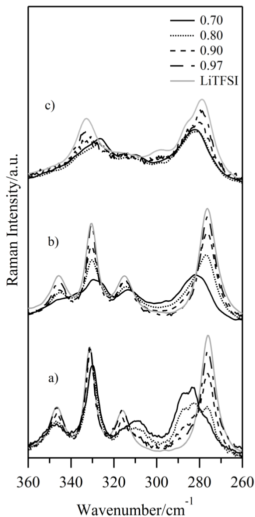
Fig. 10 Raman spectra of the \text{Li}_x\text{EMIM}_{(1-x)}\text{TFSI} ( 0.66 \leq x \leq 1 ) system; collected at 23\text{ }^\circ\text{C} a), 90\text{ }^\circ\text{C} b) and 165\text{ }^\circ\text{C} c).
