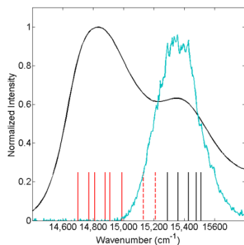
Figure 1. Linear absorption spectrum of LHCII trimers (black) and spectrum of the first two interaction pulses used in the 2DES measurements (blue). Stick plots - Chl a based excitonic states (red) and predominantly Chl b based excitonic states (black). 6,17
