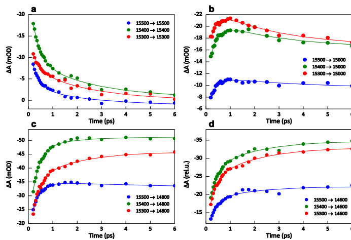
Figure 3. Time traces of the absorptive 2D signal at selected frequency intersections, indicated in the plots as \omega_\tau \rightarrow \omega_t . The top-left panel represents diagonal signals ( \omega_\tau = \omega_t ) and the rest – cross-peak signals. Each point in the time traces is the integrated 2D signal from an area of ca. 50 \text{cm}^{-1} \times 50 \text{cm}^{-1} . Symbols represent the experimentally measured data points and solid lines show the best fit using a global three-exponential analysis with lifetimes of 0.3 , 2.3 and 175 ps across all \omega_\tau/\omega_t .
