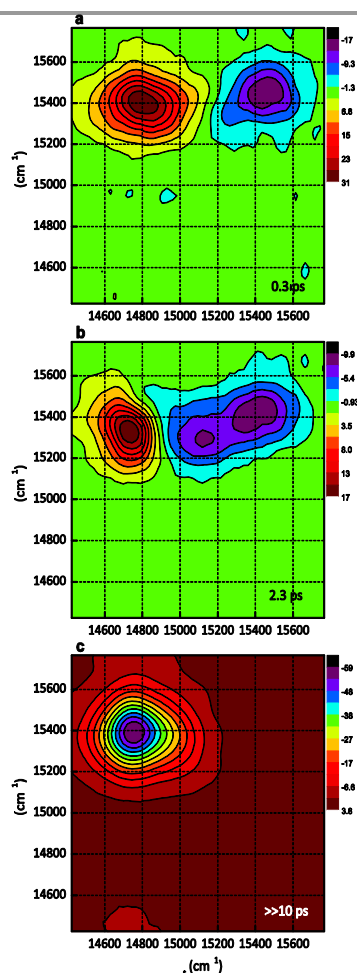
Figure 4. 2D decay-associated spectra resulting from a global fit of the 2D spectra with three exponential terms. The respective lifetimes are indicated in the plots (lower-right corner). Blue colours represent negative pre-exponential amplitudes, i.e. decay of the bleaching signal, and red colours represent positive amplitudes, i.e. rise of the bleaching signal. The first two 2D DAS show rise of the cross-peak, centered at \omega_r \sim 14800 \text{ cm}^{-1} , and the final DAS shows decay of the cross-peak.
