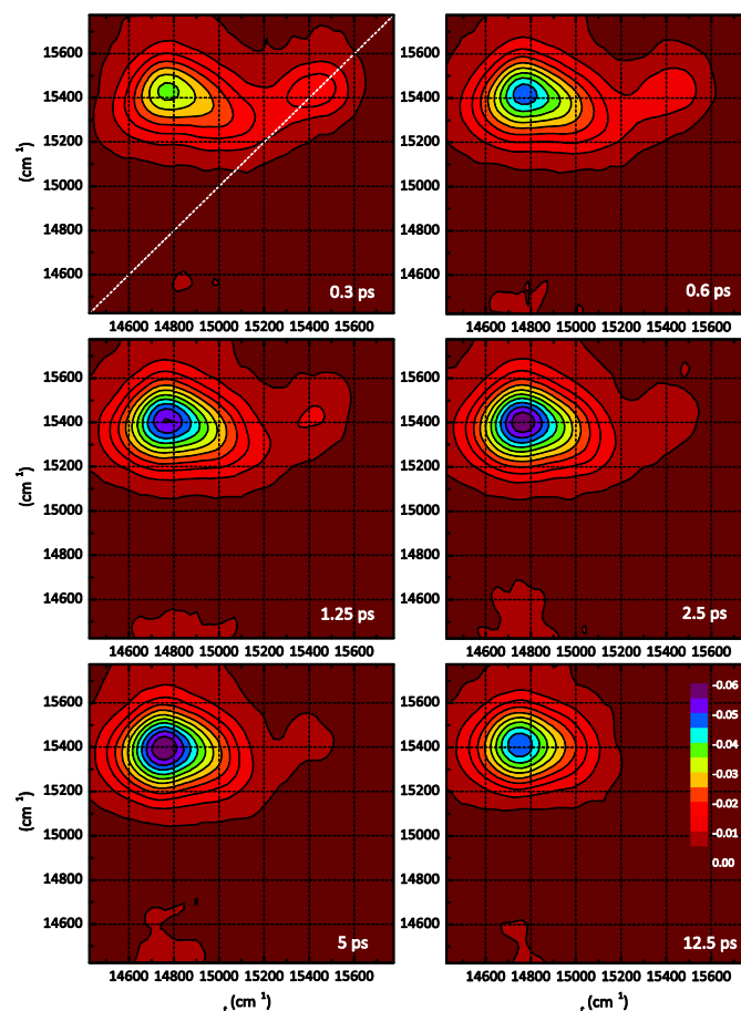
Figure 2. Purely absorptive 2DES recorded at waiting times T_w = 0.3, 0.6, 1.25, 2.5, 5 and 12.5 ps. The same colour-coding scale is used for all spectra, with red colour representing positive signal and blue colour representing negative signal. The axes correspond to the ‘pump’ frequency \omega_\tau and the ‘probe’ frequency \omega_t .
