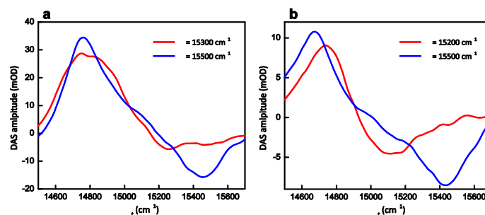
Figure 5. Horizontal slices of the 2D DAS for \tau = 0.3 \text{ ps} and \tau = 2.3 \text{ ps} at selected pump frequencies \omega_r , showing EET originating from excitonic states with the respective transition resonance frequency \omega_t .
