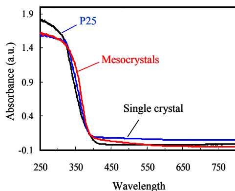
Fig. 8 UV-visible absorbance spectra of P25, \text{TiO}_2 single crystals and \text{TiO}_2 mesocrystals.
