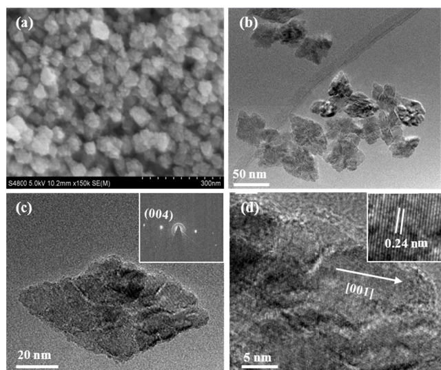
Fig. 2 SEM (a), TEM (b, c) and HRTEM (d) images of anatase TiO 2 mesocrystals synthesized under solvothermal conditions. The insets (c) and (d) are a SAED pattern and an enlarged HRTEM image.
