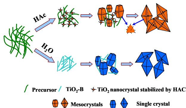
Fig. 6 Schematic of a tentative mechanism for the formation of \text{TiO}_2 mesocrystals.
