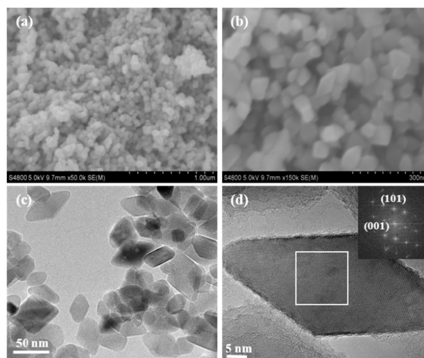
Fig. 3 SEM (a, b), TEM (c) and HRTEM (d) images of anatase TiO 2 single crystals synthesized under hydrothermal conditions. The inset in (d) is an FFT pattern.
