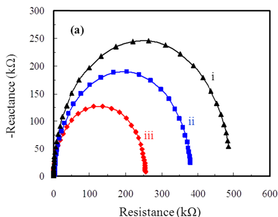
Fig. 9 EIS Nyquist plots of (i) P25, (ii) \text{TiO}_2 single crystals and (iii) \text{TiO}_2 mesocrystals under light illumination.
