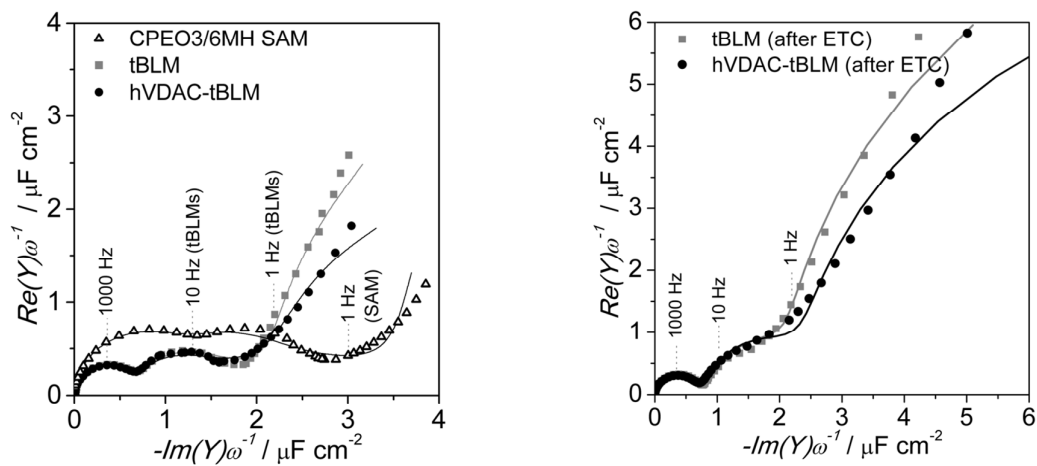
Figure 1 Cole-Cole representations of the EIS data of the formation of tBLMs on the nanostructured Au electrode before (left) and after (right) the ETC. Lines represent the fit of the equivalent circuit R_{\text{Solution}}(R_{\text{Bilayer}}C_{\text{Bilayer}})(R_{\text{Spacer}}C_{\text{Spacer}})Q (see Supporting Information) to the respective spectra. Hollow triangles refer to the impedance of the mixed CPEO3/6MH SAM; grey squares and black circles represent the tBLM and hVDAC1-tBLM, respectively. Labels indicate several frequencies of the EIS data.
