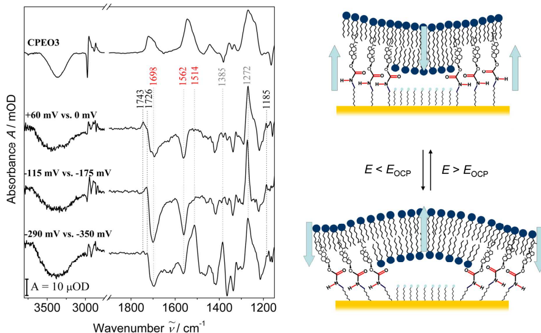
Figure 3 Left: Potential-dependent SEIRA difference spectra of pure tBLMs recorded between the potentials of +60 and 0 mV, -115 and -175 mV, and -290 and -350 mV (sv. Ag/AgCl). The SEIRA spectrum of a CPEO3 SAM, recorded vs. 1-propanol, is given on top for comparison. Bands of POPC and CPEO3 are labeled in black and red, respectively. Right: Schematic model for the electric field-dependent effects on the tBLM. Red bonds of the CPEO3 molecules refer to the labels in the spectra on the left side.
