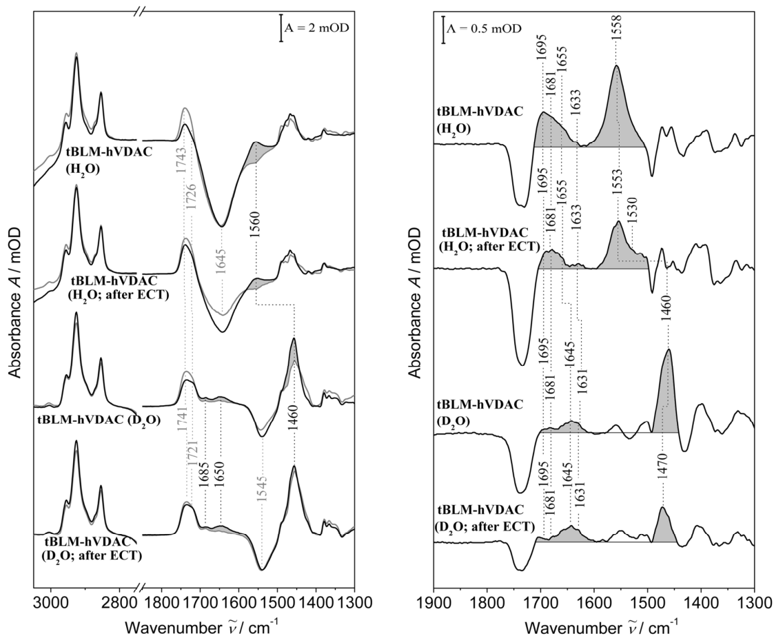
Figure 2 Left: SEIRA difference spectra of tBLMs (grey) and hVDAC1-tBLMs (black) recorded from samples in H 2 O and D 2 O, using the spectrum of the mixed SAM as the reference spectrum. Black digits refer to bands of hVDAC1 and grey digits to lipid and water. Right: SEIRA difference spectra calculated by subtracting the pure tBLM spectrum from the respective spectra of hVDAC1-tBLM on the left side. In both panels, amide I and II bands are marked in grey.
