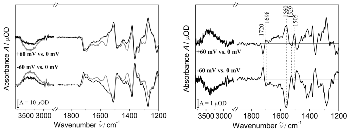
Figure 4 Left: Potential-dependent SEIRA difference spectra at the given potentials E_f (vs. EOCV) of hVDAC1-tBLMs (black) and pure tBLMs (grey). Right: Potential-dependent SEIRA double-difference spectra calculated as “hVDAC1-tBLM (black) minus tBLM (grey)” at the respective potentials.
