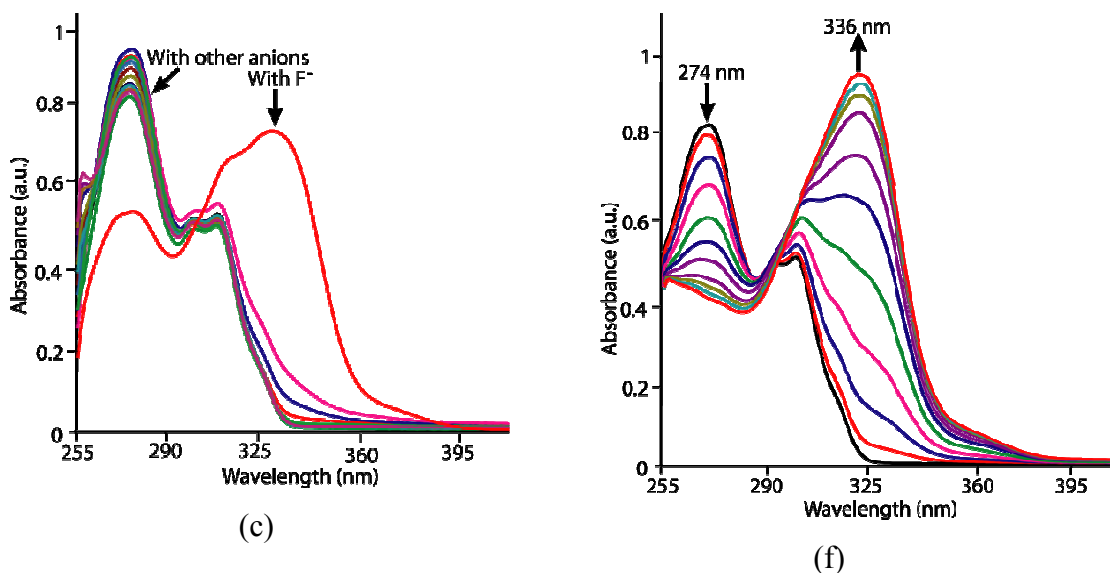
Figure 6: UV-visible spectra of (a) 1 , (b) 2 , (c) 3 ( 10^{-5} M) in dimethylsulphoxide (DMSO) with different tetrabutylammonium salts ( 100 \mu\text{l} of 10^{-5} M solution) showing fluoride salt only can cause changes in absorptions. UV-visible spectroscopic titration of TBAF ( 0 \mu\text{l} - 100 \mu\text{l} of 10^{-5} M solution) with (d) 1 ; (e) 2 and (f) 3 ( 10^{-5} M solution in DMSO).
