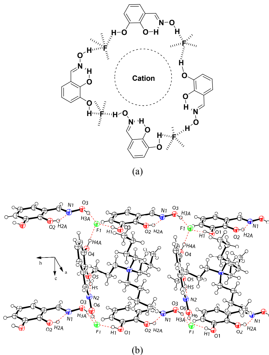
Figure 4: (a) Representation of fluoride assisted cyclic motif observed in the packing of cocrystal 5 . (b) Packing pattern of fluoride assisted assembly of 5 showing encapsulation of tetrabutylammonium cations.
