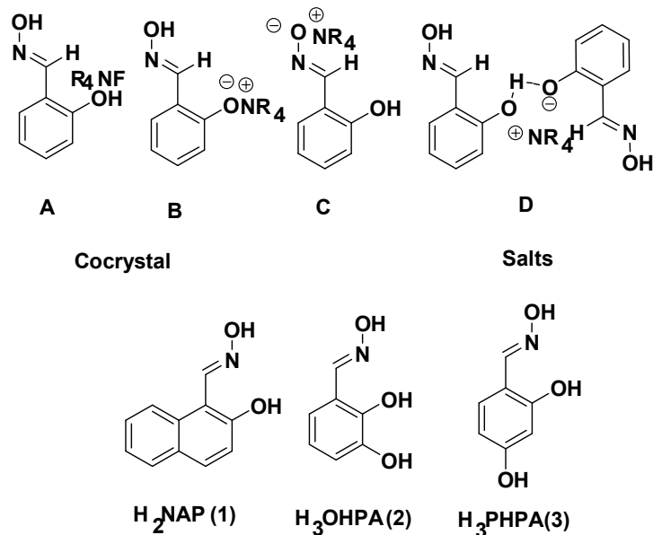
Figure 1: Structures of oximes 1-3 . A-D are some possible cocrystals and salts of quaternary ammonium fluoride with 2-hydroxyphenylaldoxime.
