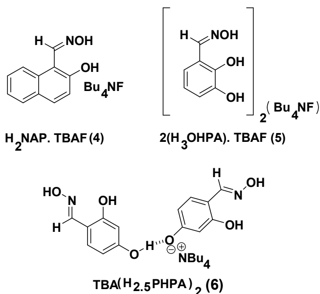
Figure 2: Cocrystals and salt from aldoximes
