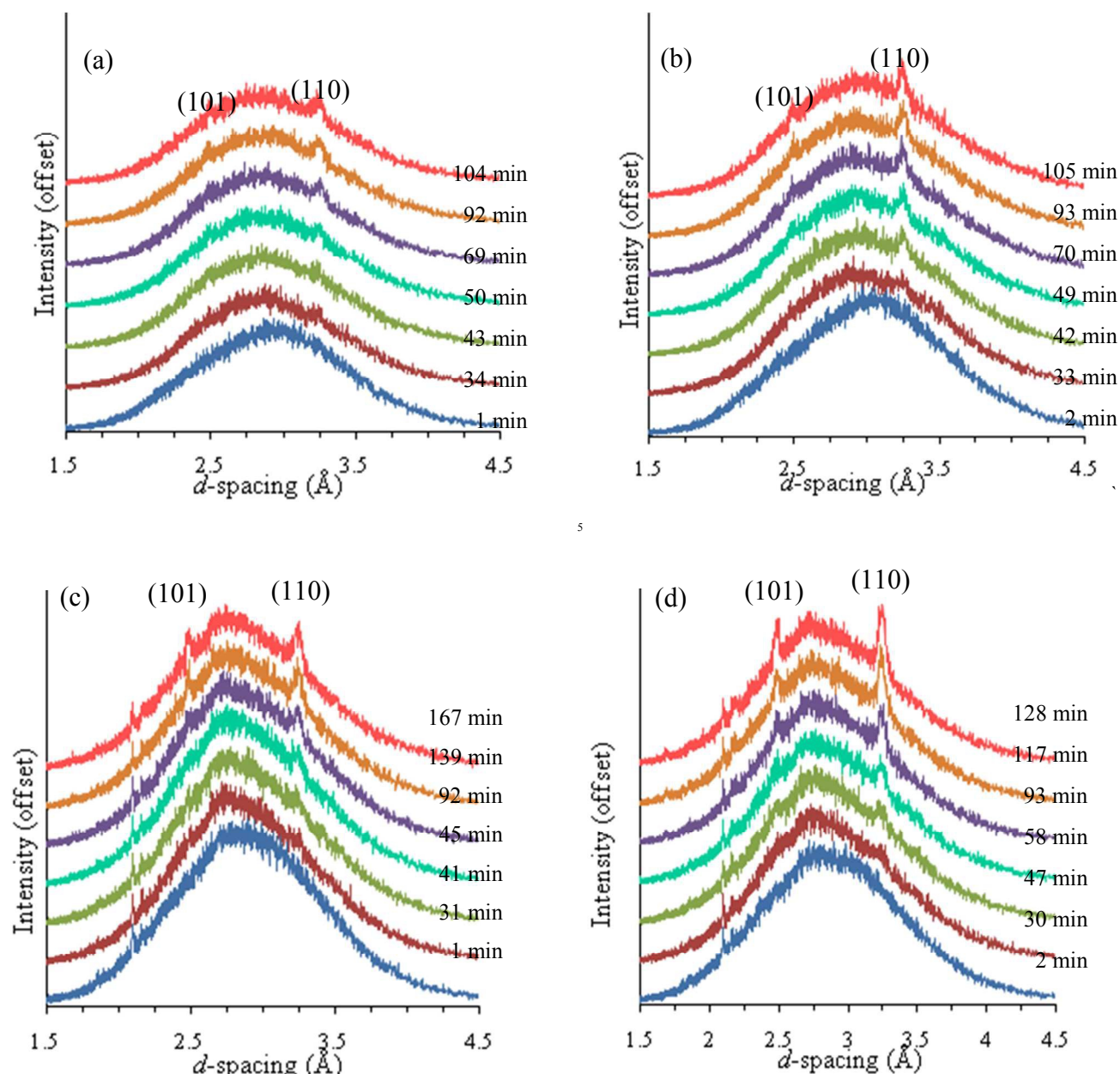
Fig. 1. In situ EDXRD data collected during the hydrothermal synthesis of TiO 2 nanoparticles from HNO 3 peptized sol-gels at *(a) 210 °C, (b) 230 °C, (c) 250 °C and *(d) 270 °C. * Modified versions of our previously published EDXRD graphs [50].
