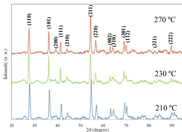
Fig. 3. XRD patterns of TiO 2 nanoparticles produced by in situ hydrothermal reactions of HNO 3 peptized sol-gels at *210 °C, 230 °C and *270 °C. * Modified versions of our previously published XRD patterns [50].
