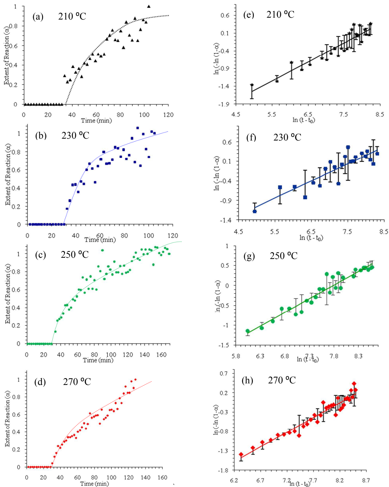
5 Fig. 2. Extent of reaction against time for (110) peak of \text{TiO}_2 particles produced by in situ hydrothermal processes at 210, 230, 250 and 270 °C (a-d) and their corresponding Sharp and Hancock plots showing the kinetic data (e-h) respectively.
