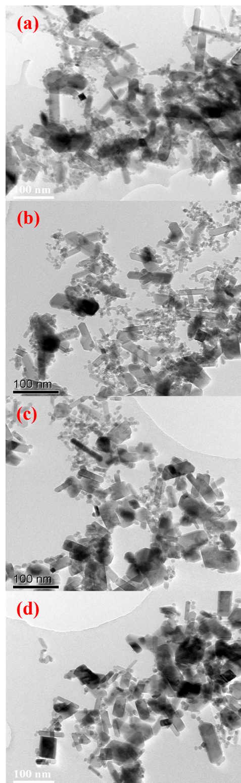
Fig. 4. TEM images of TiO 2 nanoparticles produced by the in situ hydrothermal reactions of HNO 3 peptized sol-gels at (a) 210 °C, (b) 230 °C, (c) 250 °C and (d) 270 °C.
