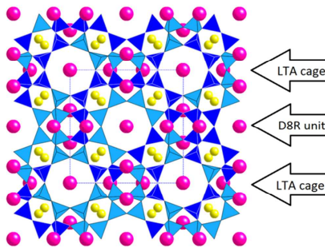
Figure 1 Zeolite RHO, Si and Al tetrahedral units are represented by blue and light blue tetrahedra, Cs atoms are in pink and Na atoms are yellow. LTA and D8R secondary building units are labelled. In this representation, there are 8 LTA cages in each corner and one in the middle, and 8 D8R units connecting the corner LTA units.
