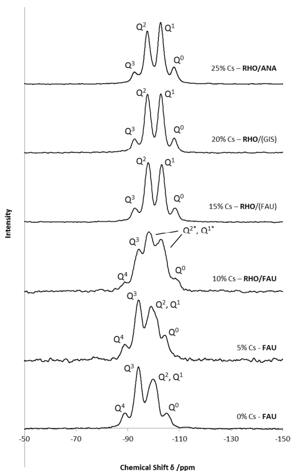
Figure 10 ^{29}\text{Si} SS MAS NMR data for all samples.
