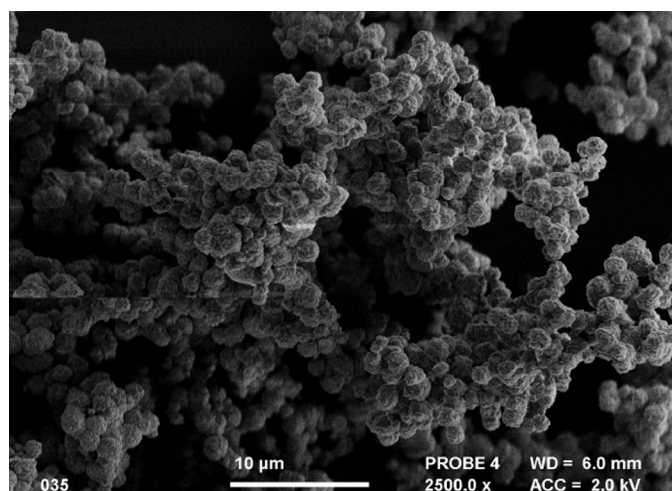
Figure 5 SEM micrographs for sample 1, 0% of Cs, where faujasite zeolite can be seen. The scale bar is 10 micrometres.
