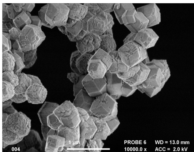
Figure 4 An SEM image of a zeolite RHO sample synthesised using 18-crown-6 ether as organic template. Although some crystals are not smooth, the overall rhombic dodecahedral geometry can be seen. Scale bar equal 1 micrometer.
