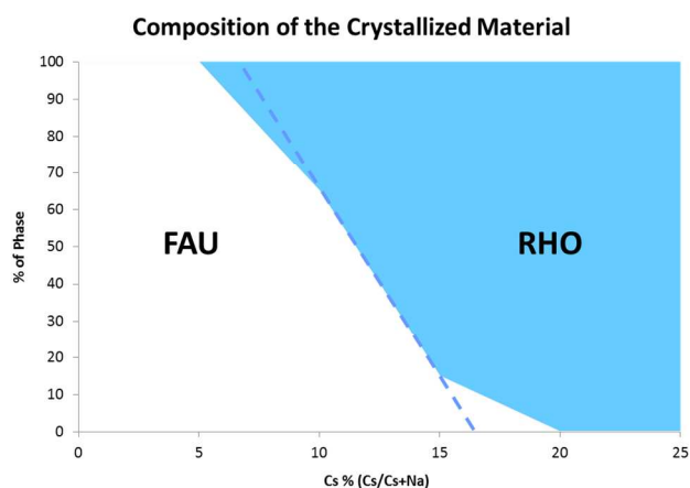
Figure 3 A Schematic Phase Diagram showing the estimated % of each zeolite (zeolites RHO and Na-X (FAU)) at different cation contents.
