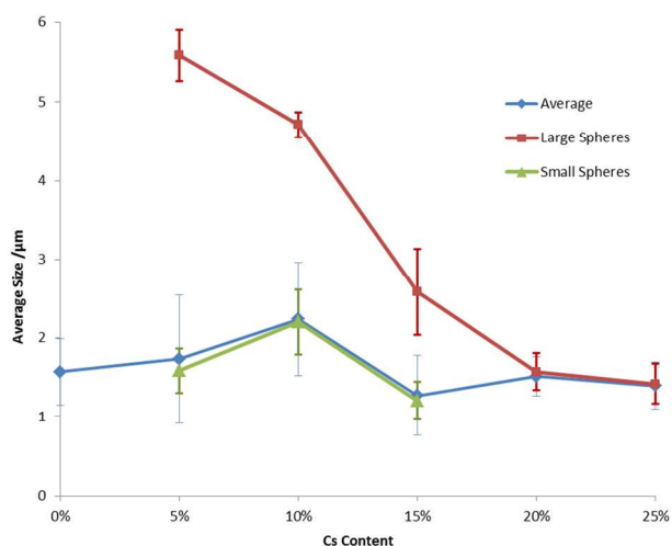
Figure 8 Average size of particles calculated from SEM data for samples 1-6.
