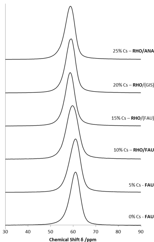
Figure 9 ^{27}\text{Al} SS MAS NMR data for all samples.
