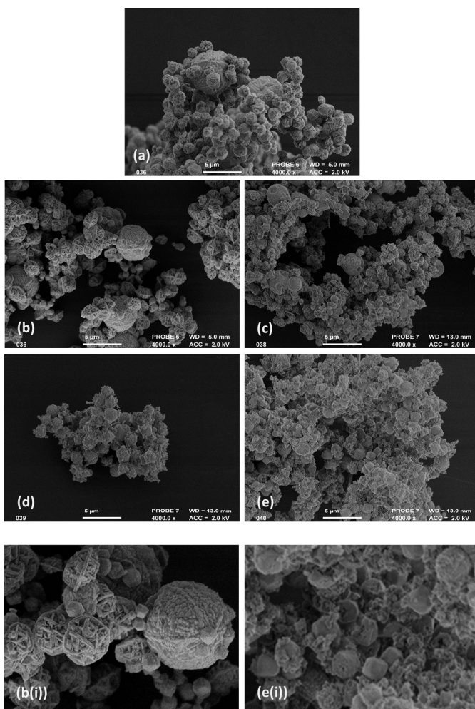
Figure 6 SEM micrographs for samples 2-6: a)5% of Cs, faujasite zeolite; b)10% of Cs, a mixture of RHO and faujasite zeolites; c)15% of Cs, mainly zeolite RHO, with faujasite impurity; d)20% of Cs, predominantly zeolite RHO; e) 25% of Cs, mainly zeolite RHO with analcime impurity. The scale bar is 5 micrometres. Figures b(i) and e(i) are to scale zoomed in micrographs of figures b and e respectively. There is a clear distinction of morphology in these micrographs.
