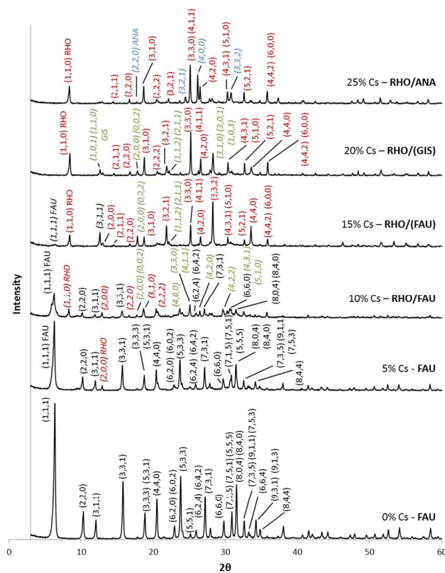
Figure 2 PXRD spectra for samples 1-6. The (h,k,l) labels are shown in different colours to indicate the peaks assigned to the different zeolites present.
