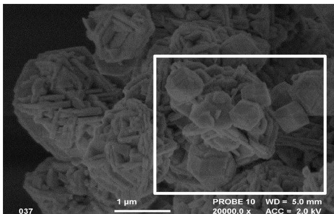
Figure 7 An SEM image of the 10% caesium sample, showing the third particle species – nanoscale polyhedrons which are highlighted by the white box. Scale bar is equal 1micrometer.
