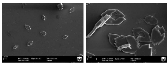
Fig. 5 SEM image of calcium oxalate (0.30 mM) particles formed in the presence of 5 g/L a) \text{TzPhCN}^- (0.029 M) and b) \text{BaPhCN}^- (0.034 M)
