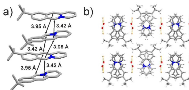
Figure 7. X-ray crystal structure of: a) of an infinite stack of 9-C(CH 3 ) 3 cations (hydrogen atoms are omitted for clarity), and b) crystal packing of 9-C(CH 3 ) 3 viewed along the crystallographic axis c .
