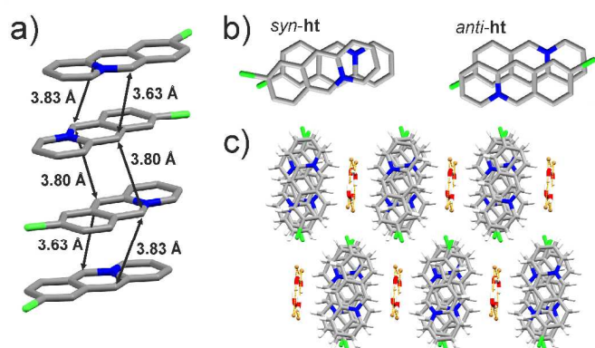
Figure 2. X-ray crystal structure of: a) an infinite stack of 9-Cl cations (hydrogen atoms are omitted for clarity), b) parallel and angular offsets in pairs of syn-ht and anti-ht pairs of acridizinium cations, and c) crystal packing of 9-Cl viewed along the crystallographic plane (-110).
