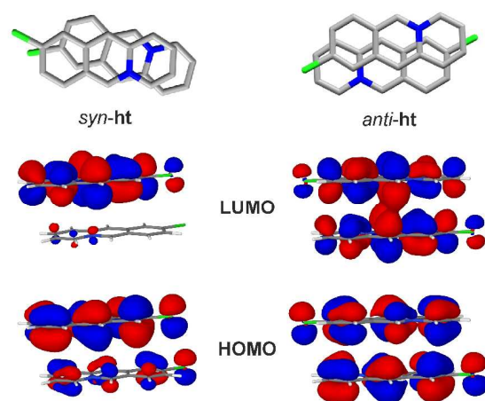
Figure 8. HOMO and LUMO orbitals of the syn-ht (left) and anti-ht (right) pairs of 9-chloroacridizinium cations in 9-Cl .
