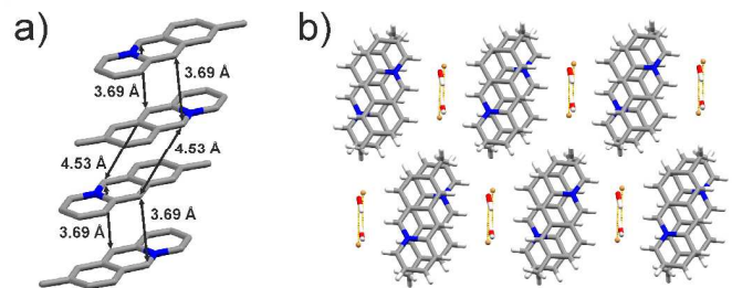
Figure 6. X-ray crystal structure of: a) of an infinite stack of 9-CH 3 cations (hydrogen atoms are omitted for clarity), and b) crystal packing of 9-CH 3 viewed along the crystallographic axis a .
