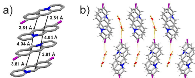
Figure 4. X-ray crystal structure of: a) of an infinite stack of 9-I cations (hydrogen atoms are omitted for clarity), and b) crystal packing of 9-I-Br viewed along the crystallographic axis a .
