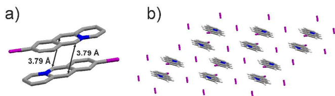
Figure 5. X-ray crystal structure of: a) of an infinite stack of 9-I cations (hydrogen atoms are omitted for clarity), and b) crystal packing of 9-I-I 3 viewed along the crystallographic plane (-101).
