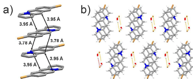
Figure 3. X-ray crystal structure of: a) of an infinite stack of 9-Br cations (hydrogen atoms are omitted for clarity), and b) crystal packing of 9-Br viewed along the crystallographic axis a .
