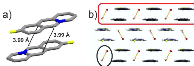
Figure 1. X-ray crystal structure of: a) two stacked 9-F cations (hydrogen atoms are omitted for clarity, only one occupancy is shown), and b) crystal packing of 9-F viewed along a^* .
