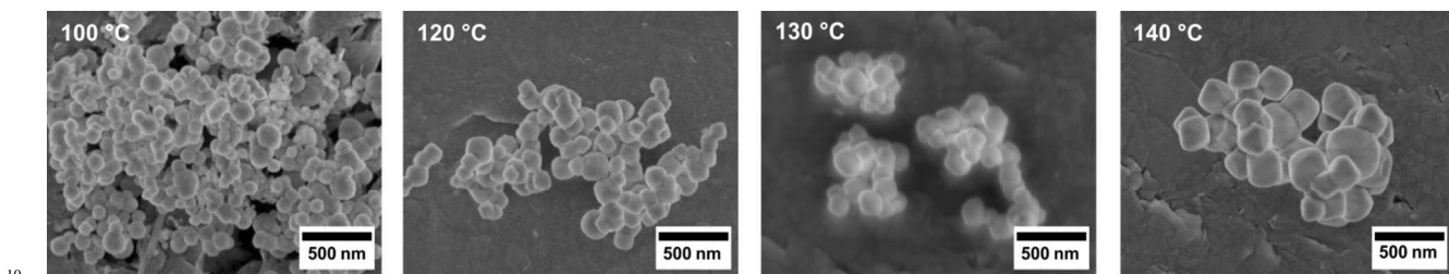
Fig. 7 SEM images of Zr-fumarate MOF synthesised at various temperatures (as given in the images) in a DMF-based synthesis ( \text{ZrCl}_4/\text{H}_2\text{fum}/\text{formic acid}/\text{DMF} 1:3:70:500).
