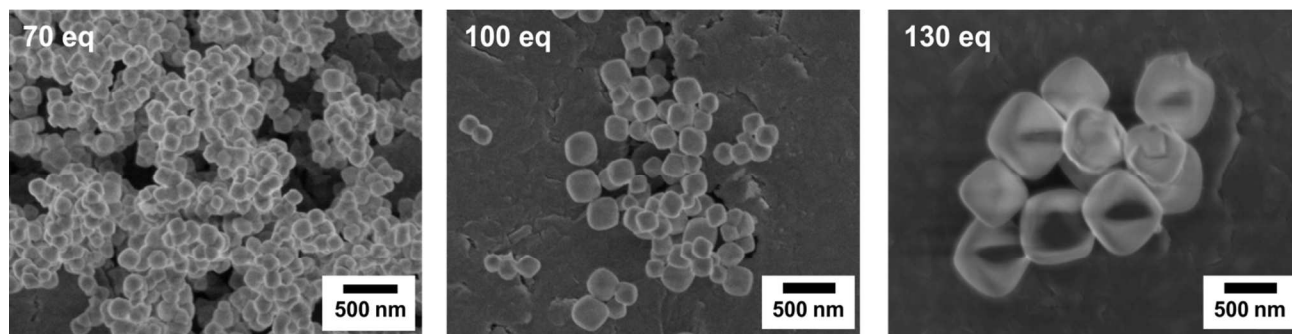
Fig. 9 SEM images obtained from Zr-fumarate MOF synthesised with various amounts of formic acid in a DMF-based synthesis ( \text{ZrCl}_4/\text{H}_2\text{fum}/\text{formic acid}/\text{DMF} 1:3: x :500) at 120 °C.
