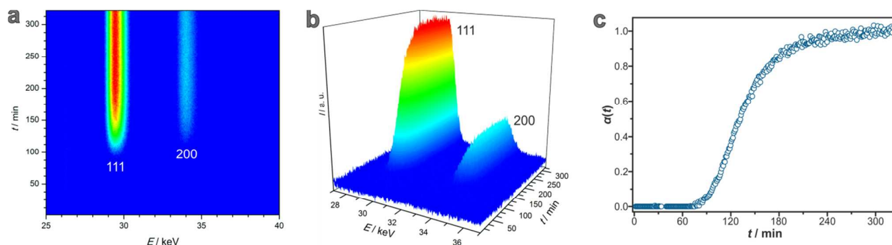
Fig. 1 Examples for the visualisation of time-resolved EDXRD data from a Zr-fum MOF synthesis (molar ratios ZrCl_4/H_2fum/formic\ acid/H_2O of 1:3:150:1074 at 43 °C). The 111 and 200 Bragg reflections are visible. a) 2D contour plot; (b) 3D view; (c) crystallisation curve \alpha(t) of the 111 Bragg reflection.
