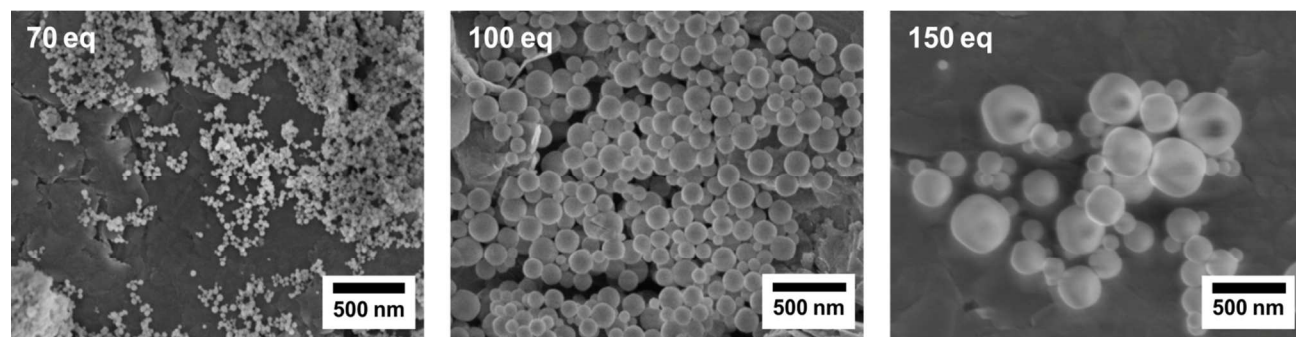
Fig. 4 SEM images of Zr-fum MOF samples synthesised with various concentrations of modulator (as given in the images) in a water-based synthesis at 43 °C ( ZrCl_4/H_2fum/formic\ acid/H_2O 1:3: x :1074).
