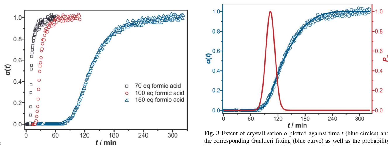
Fig. 2 Extent of crystallisation \alpha plotted against time t . Crystallisation curves measured for syntheses of Zr-fum MOF in water-based systems under variation of the concentration ( x equivalents) of the modulator formic acid x ( ZrCl_4/H_2fum/formic\ acid/water in molar ratios of 1:3: x :1074, 43 °C).
