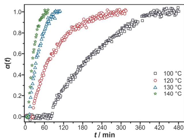
Fig. 5 Extent of crystallisation \alpha plotted against time t . Crystallisation curves measured for syntheses of Zr- fum MOF in DMF-based systems under variation of the temperature T ( \text{ZrCl}_4/\text{H}_2\text{fum}/\text{formic acid}/\text{DMF} in molar ratios of 1:3:70:500).
